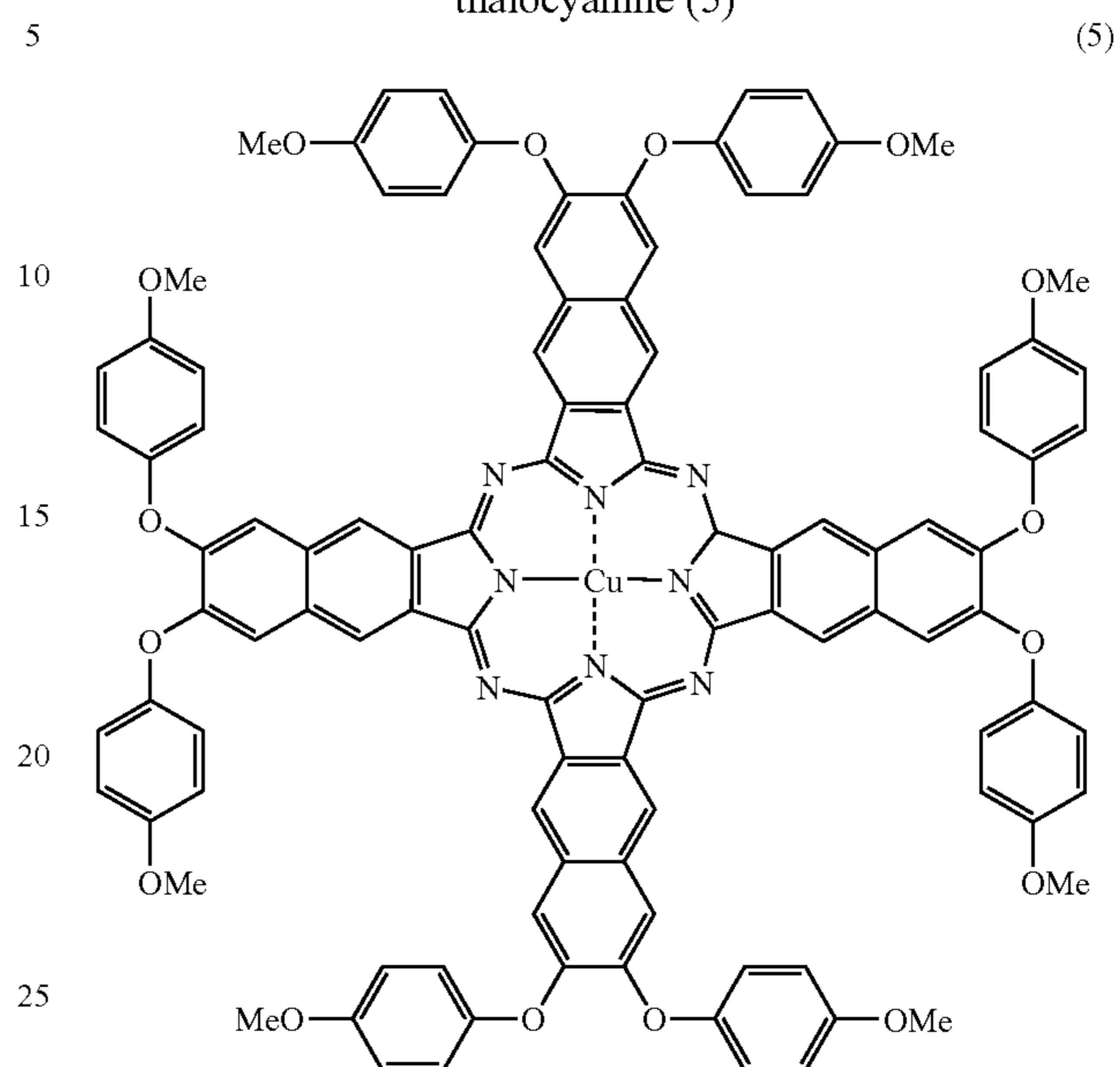
Copper(II) tetrakis[6,7-(4'-methoxyphenoxy)]naphthalocyanine (5)
