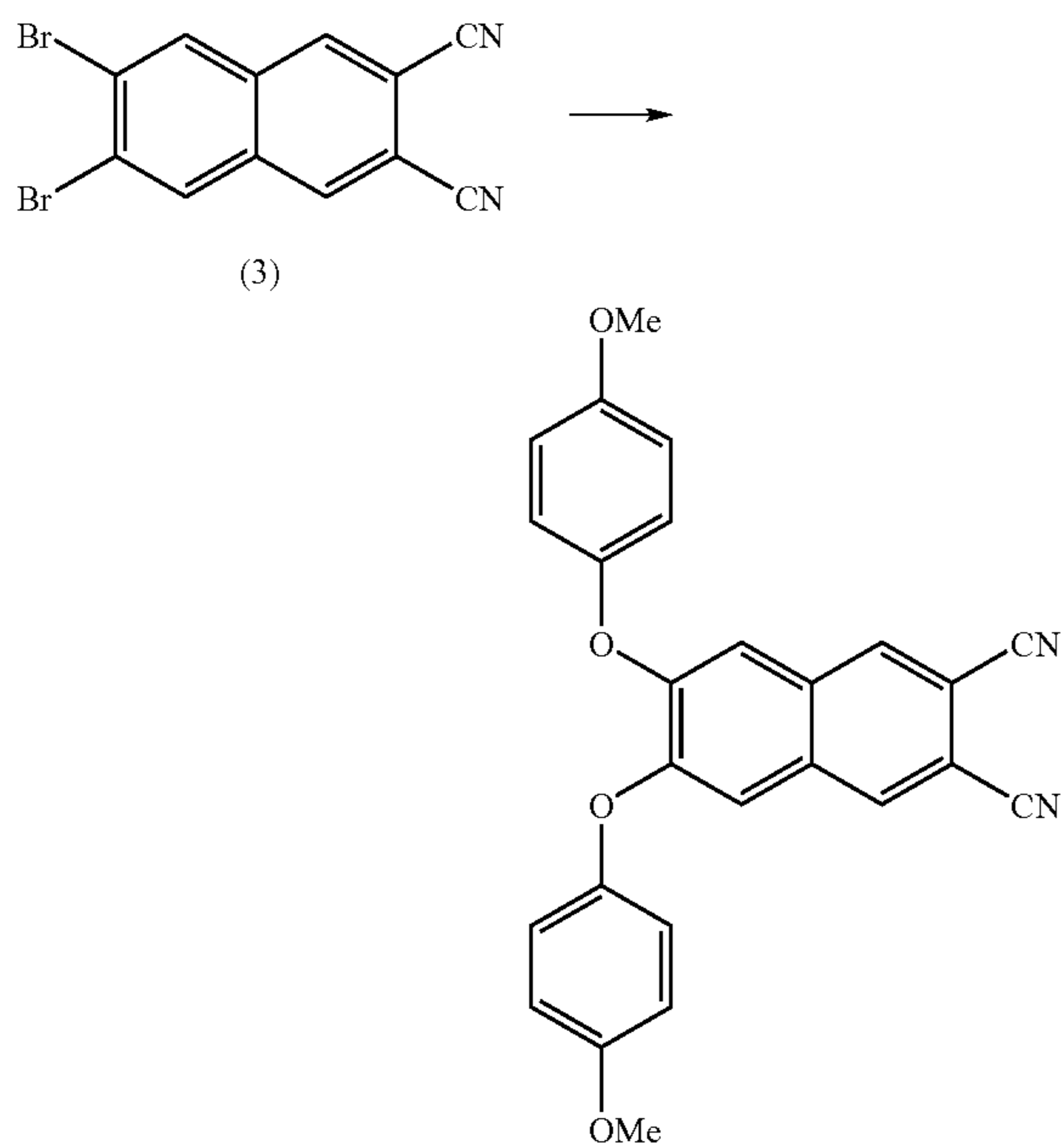
6,7-(4'-Methoxyphenoxy)naphthalene-2,3-dicarbonitrile (4)
