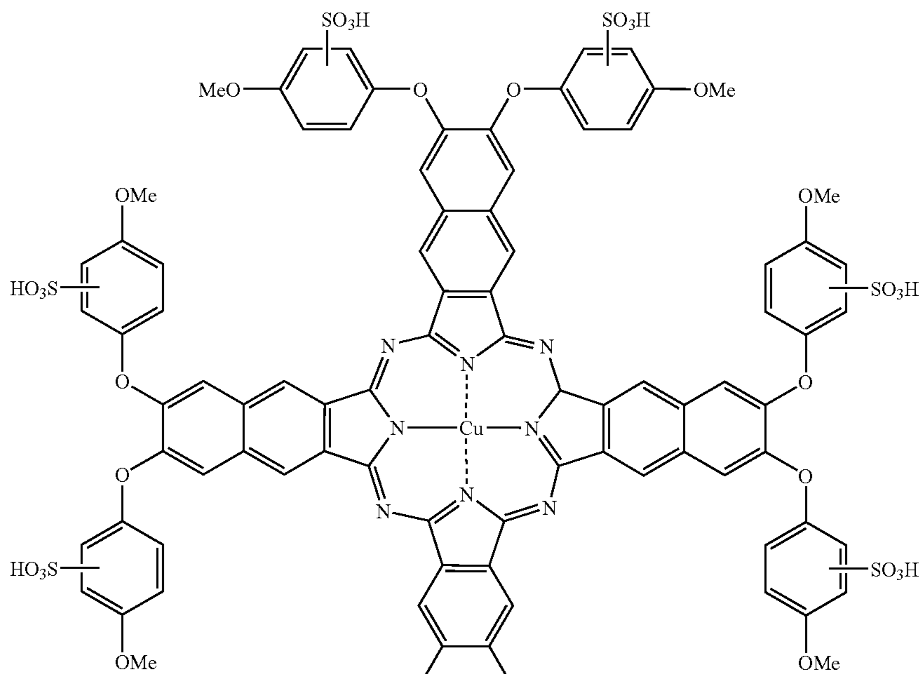
Sulfonation of copper(II) tetrakis[6,7-(4'-methoxyphenoxy)]naphthalocyanine
