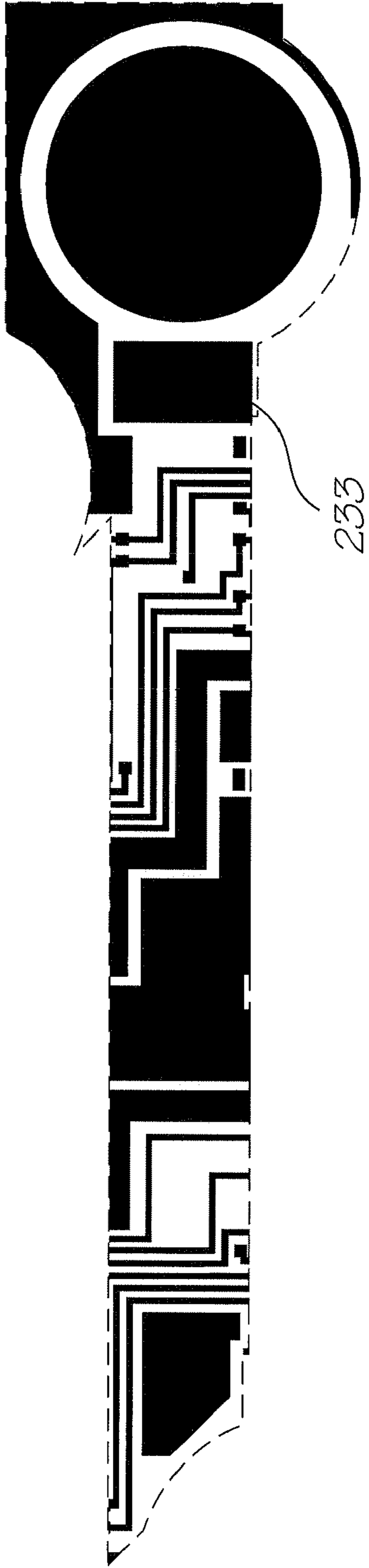
Metal 2 mask
