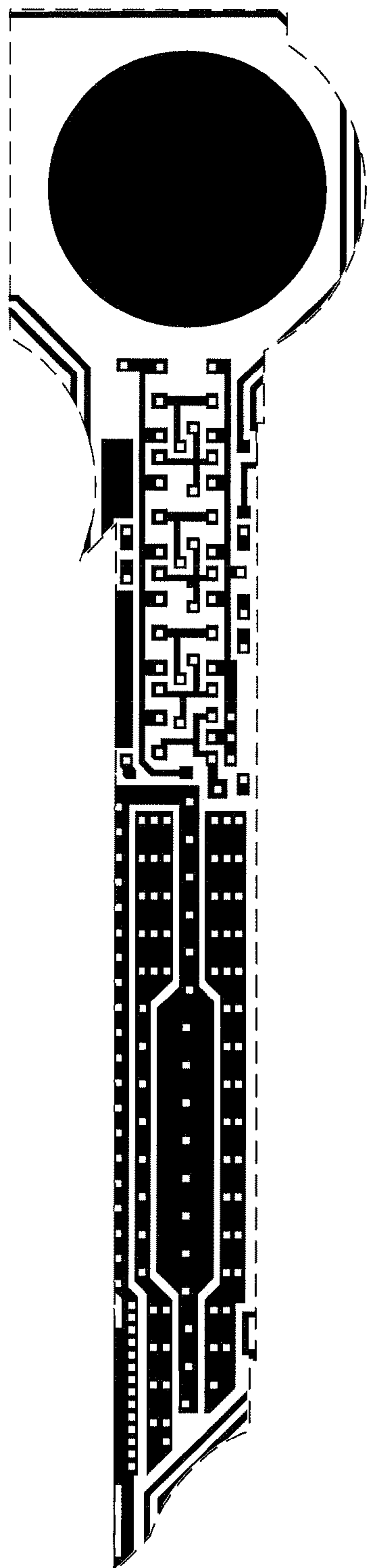
Metal 1 mask
