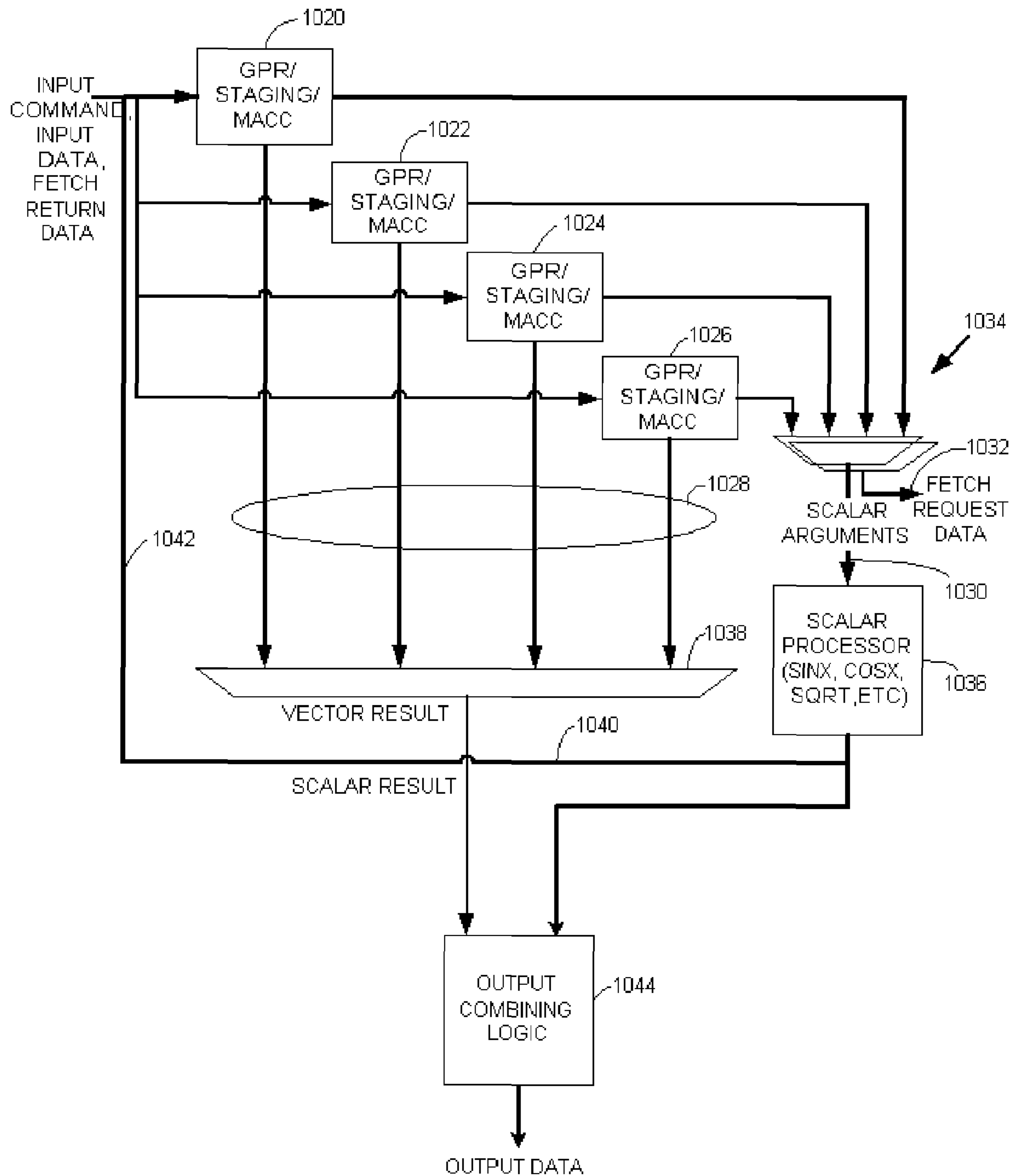
ALU (VECTOR SCALAR PROCESSOR) FIG. 10
