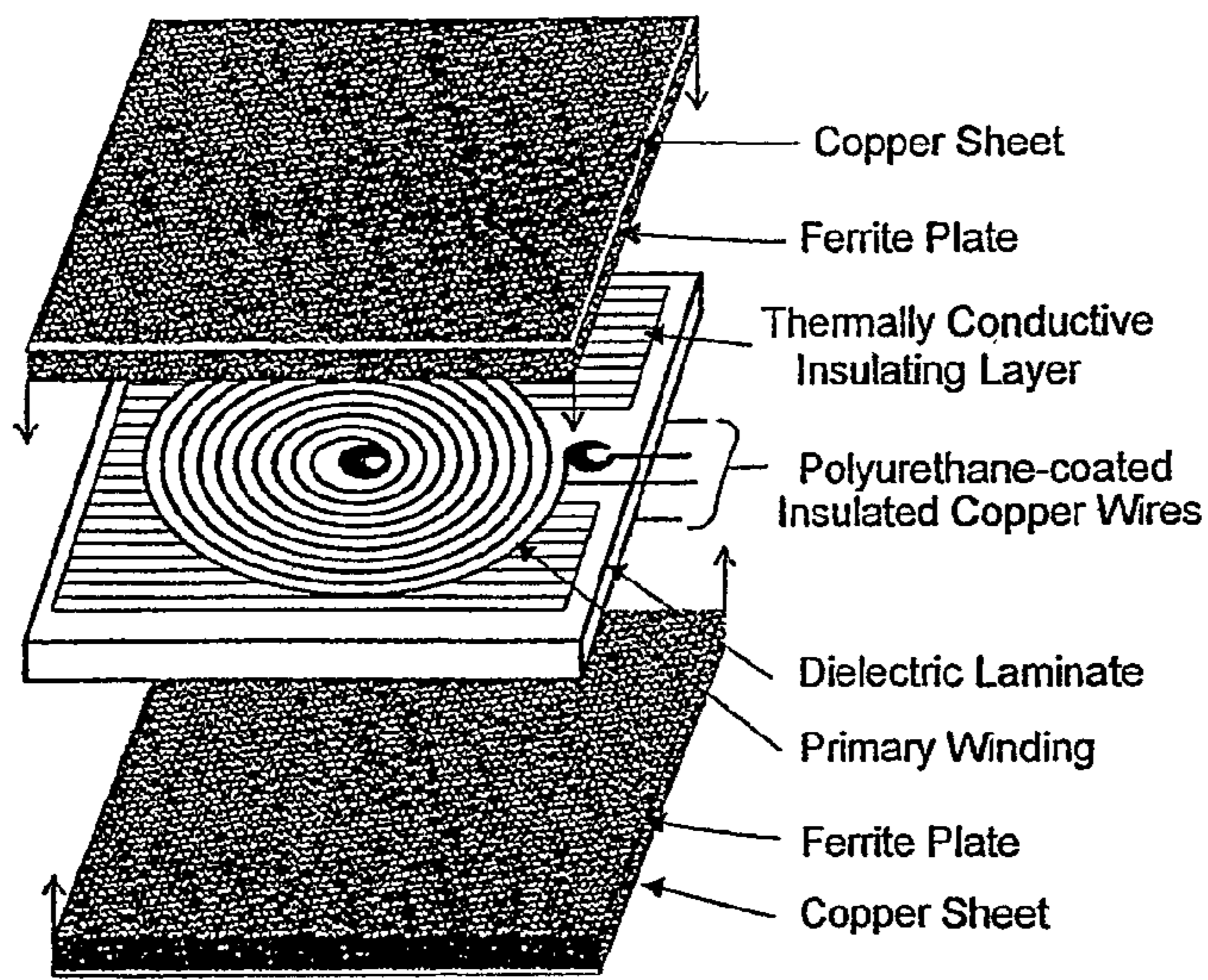
FIG.3 (PRIOR ART)
