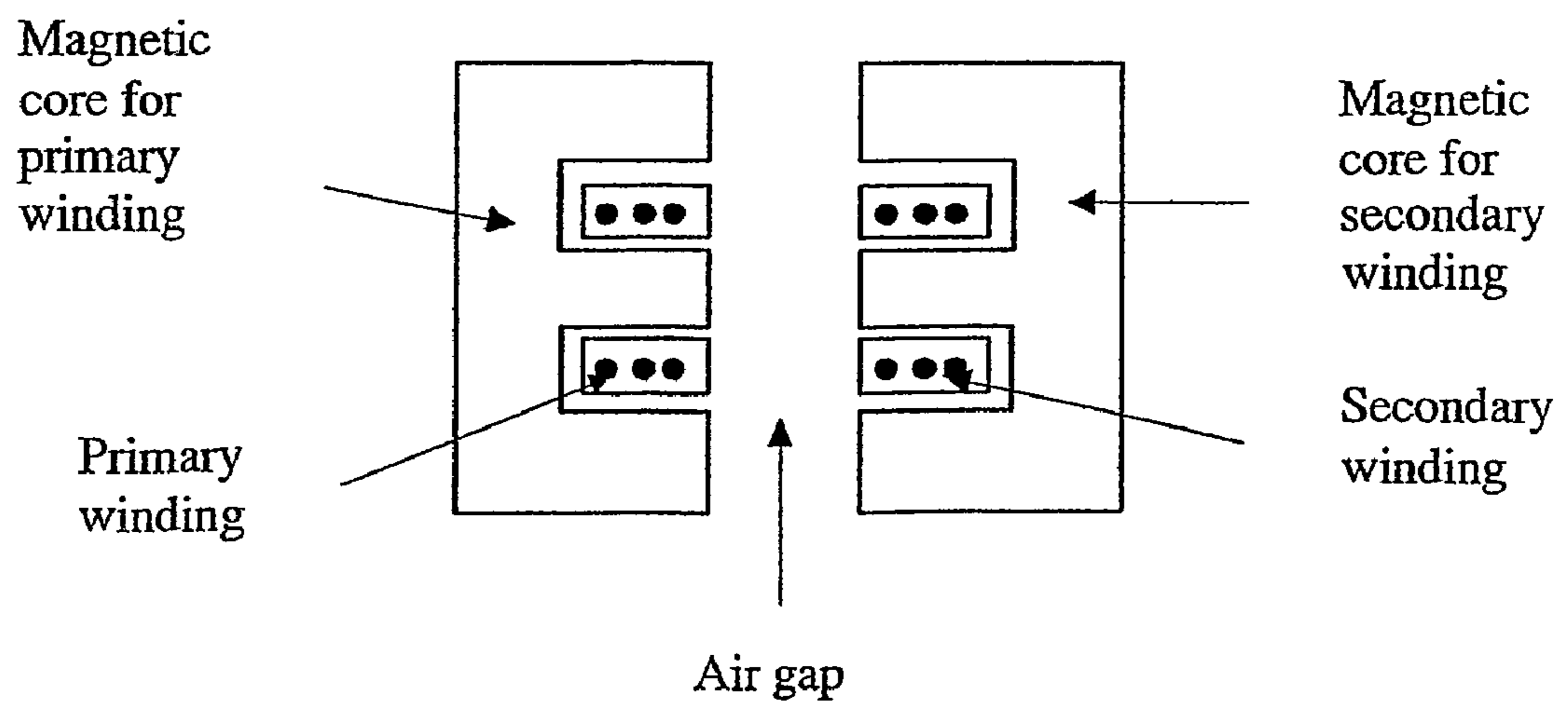
FIG. 2 (PRIOR ART)
