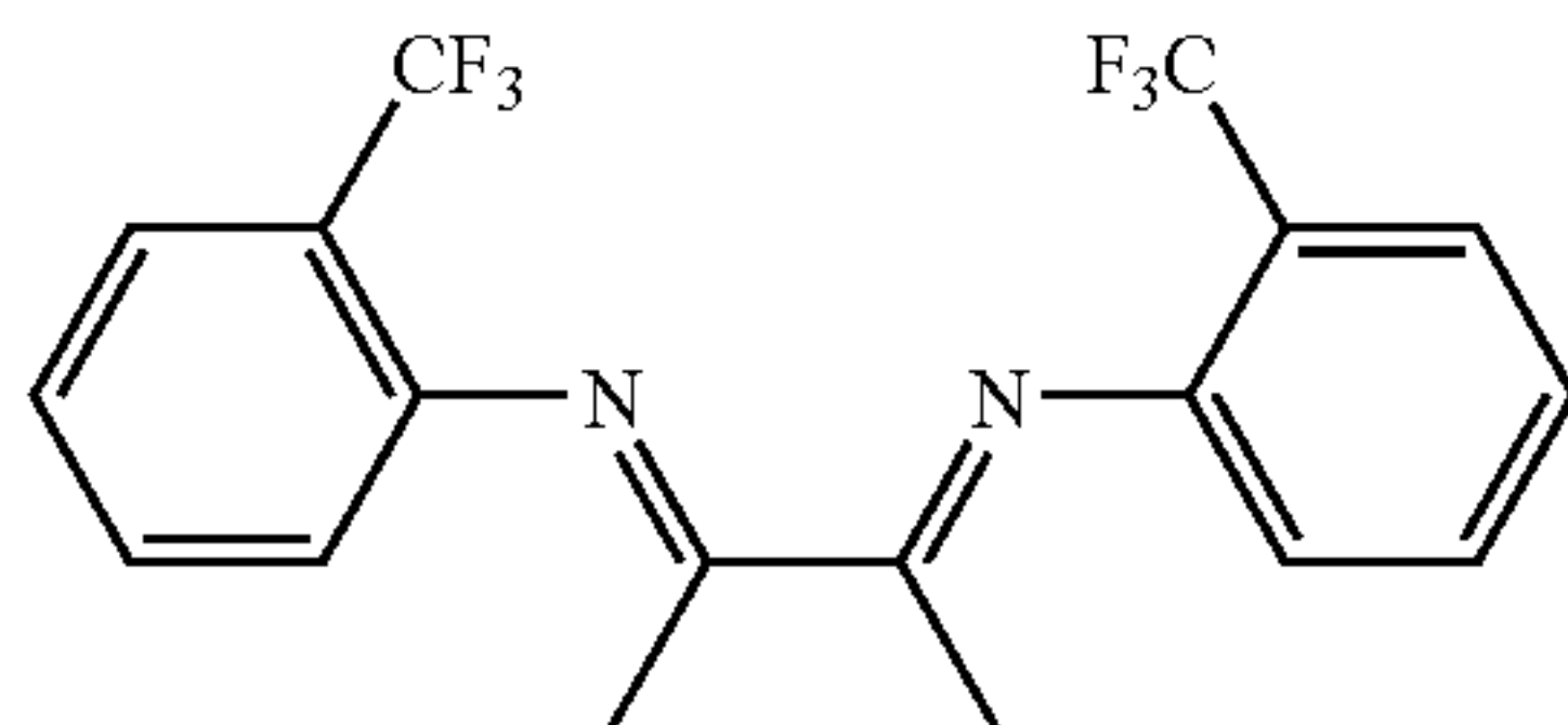
N,N'-di(trifluoromethylbenzene)-2,3-diiminoethane
