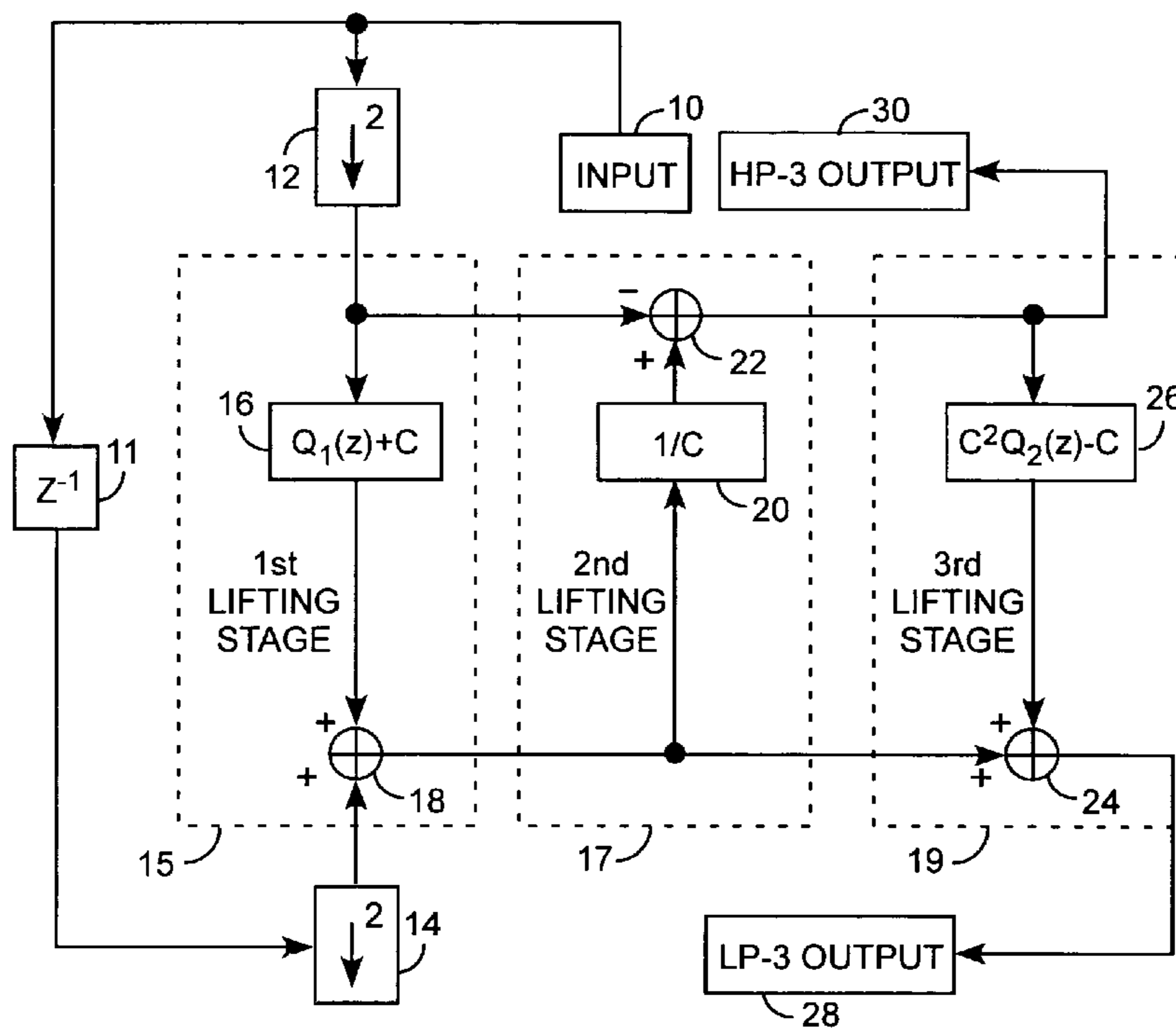
THREE LIFTING STAGE WAVELET TRANSFORM
