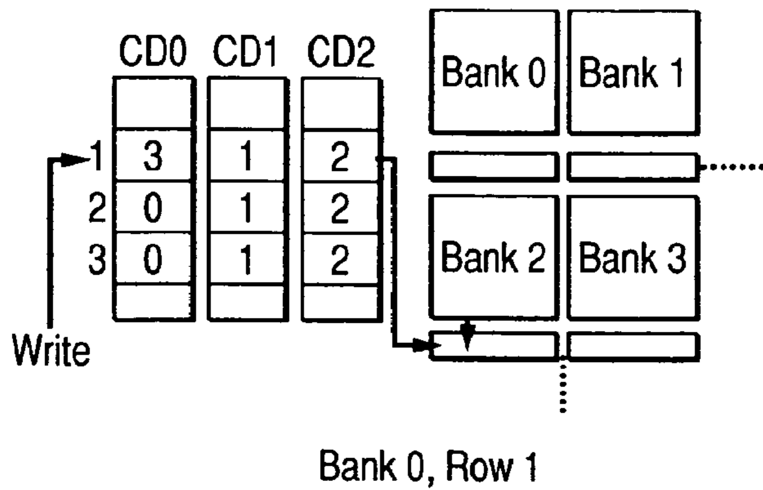
CYCLE #1: WRITE ACCESS, CACHE MISS STATE
