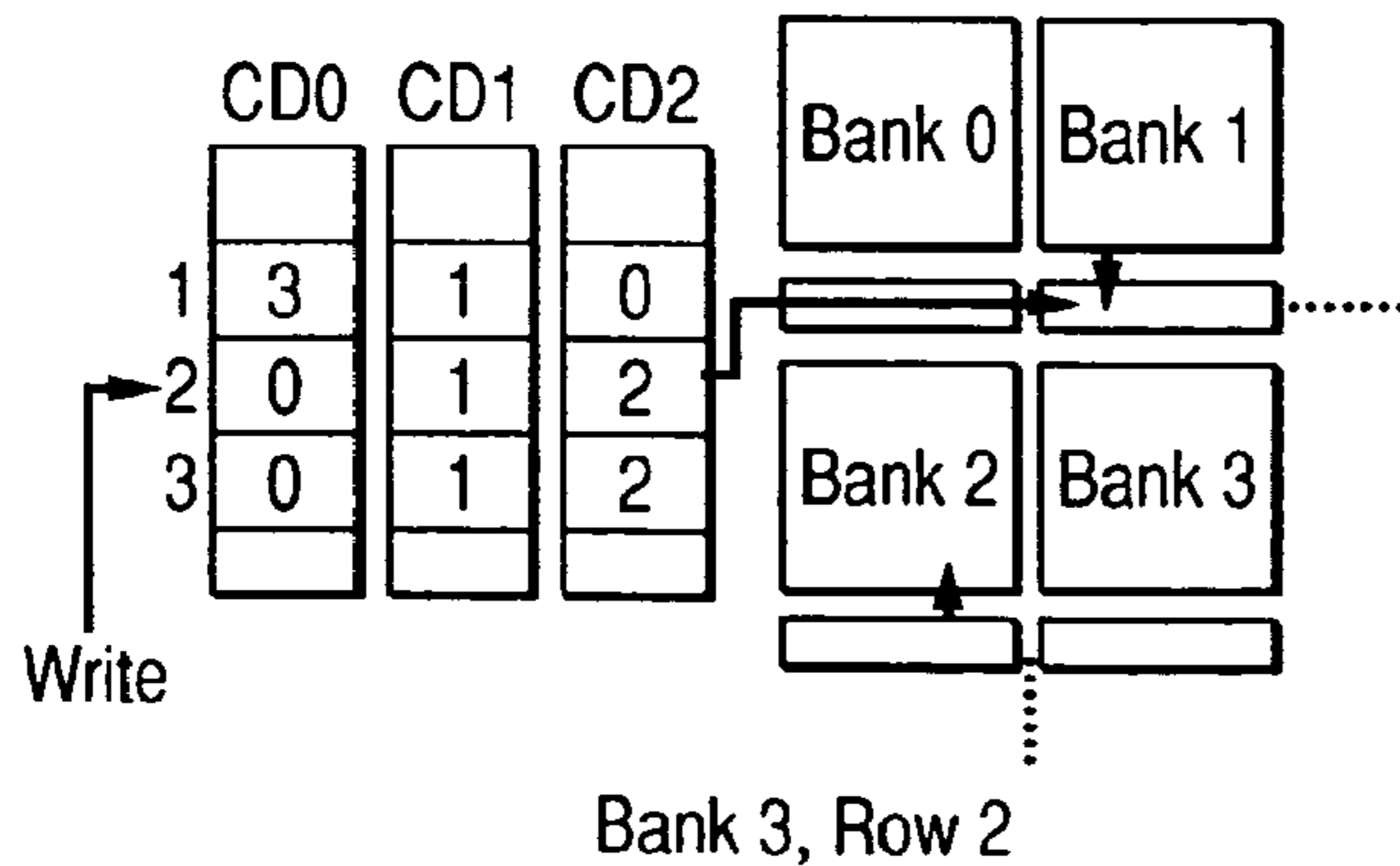
CYCLE #2: WRITE ACCESS, CACHE MISS STATE
