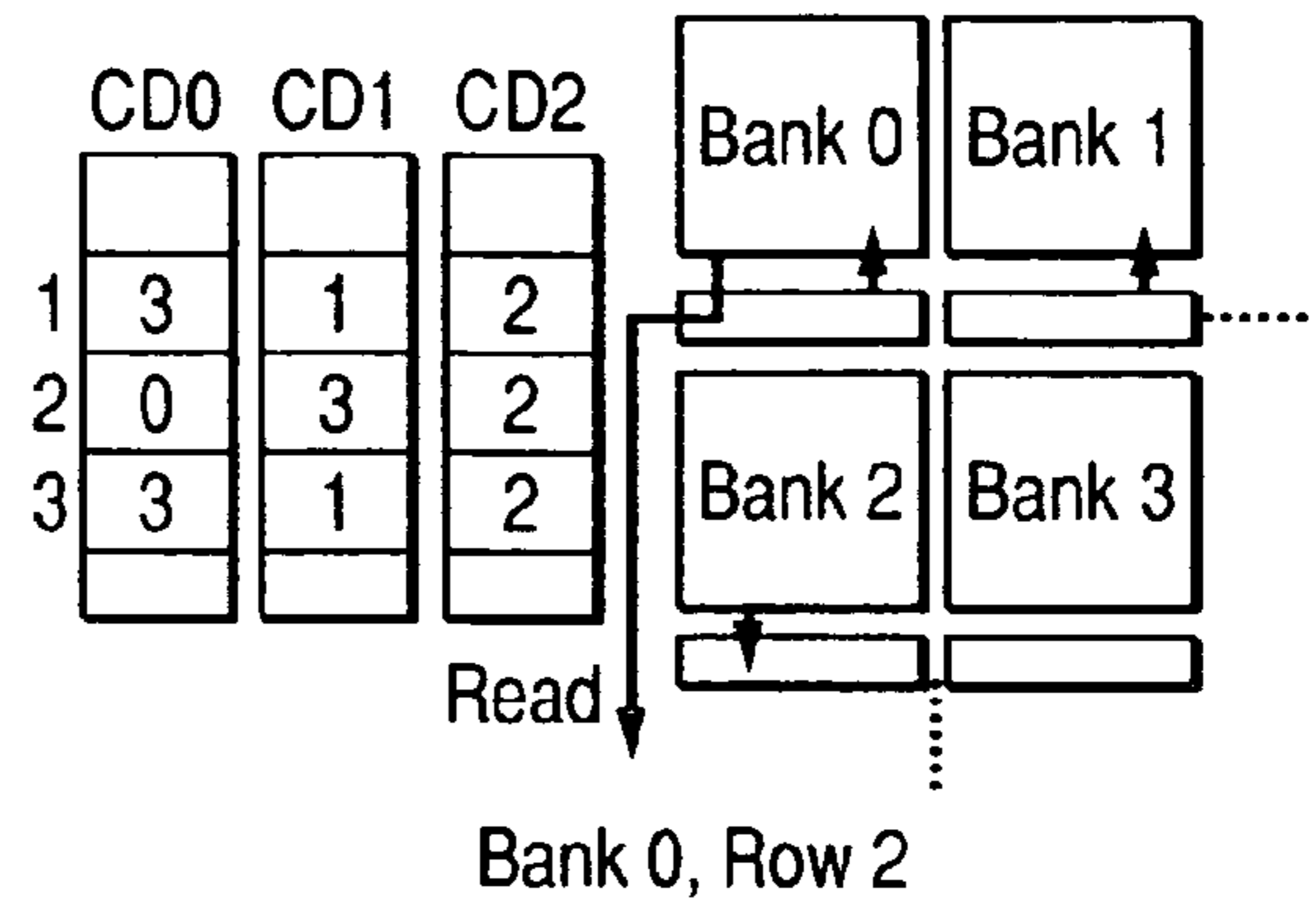
CYCLE #4: READ ACCESS, CACHE MISS STATE
