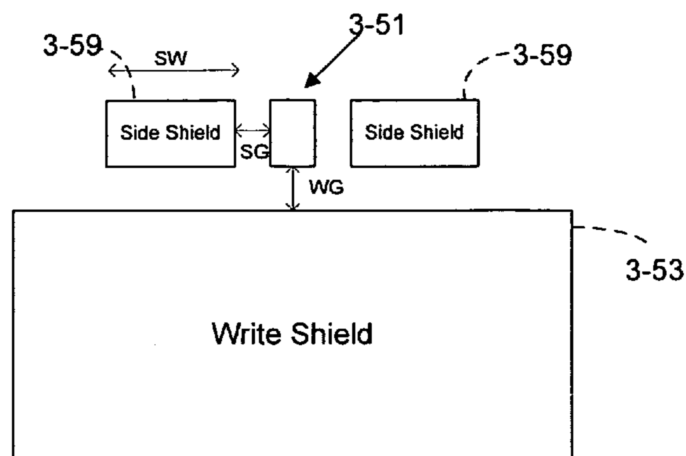
(b) Bottom (ABS) View
