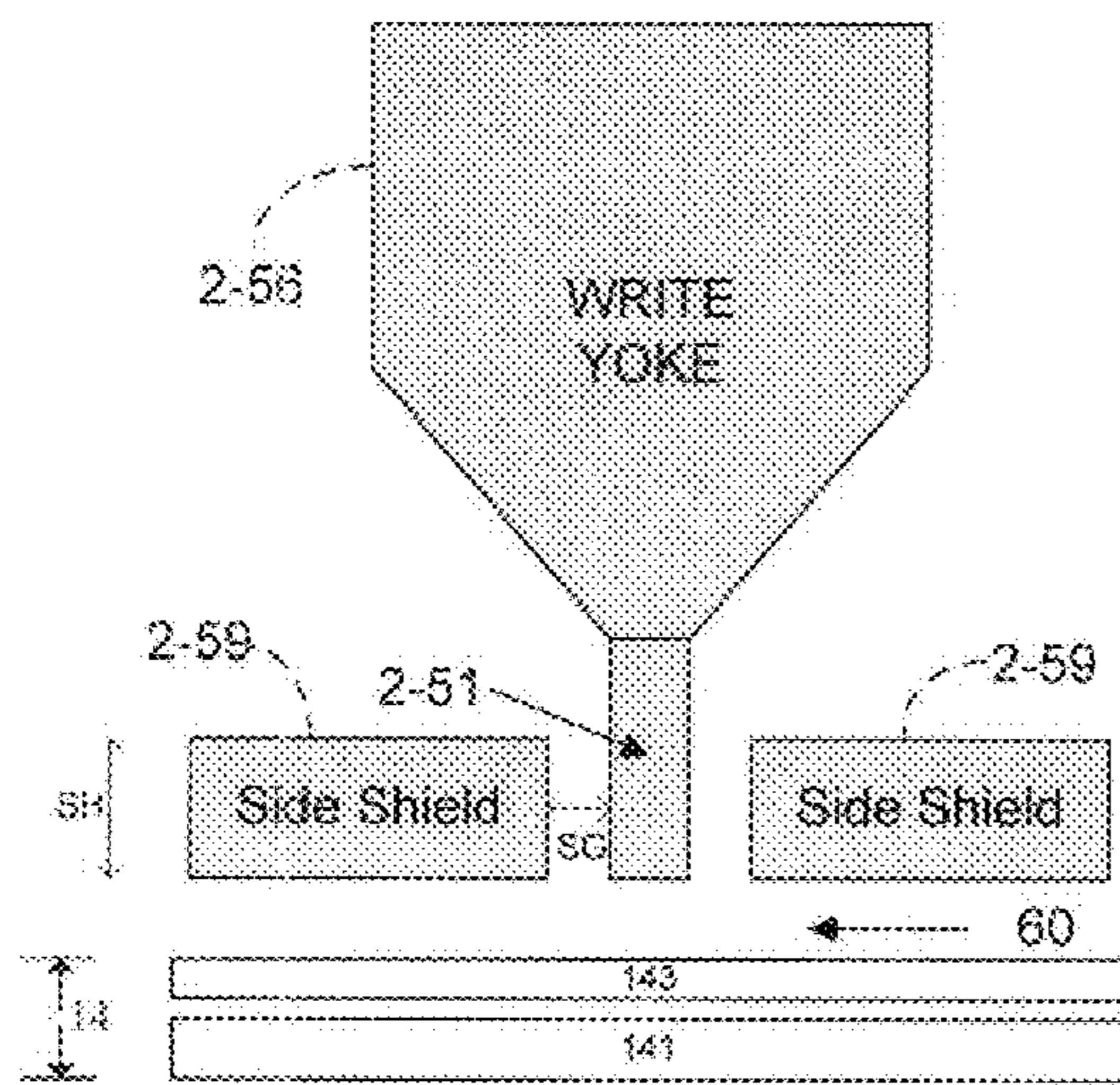
(a) Frontal View
