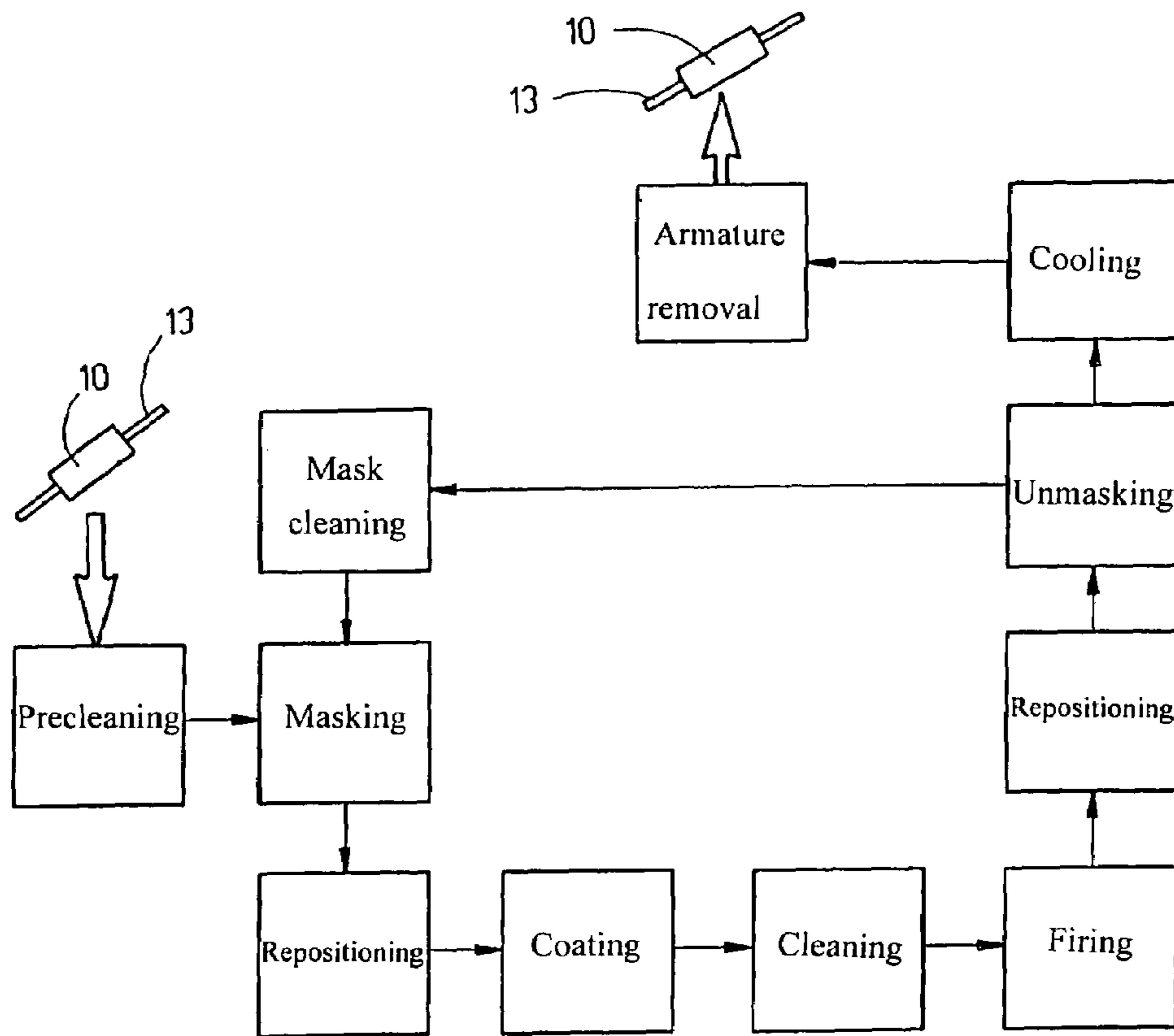
Fig.1 (PRIOR ART)
