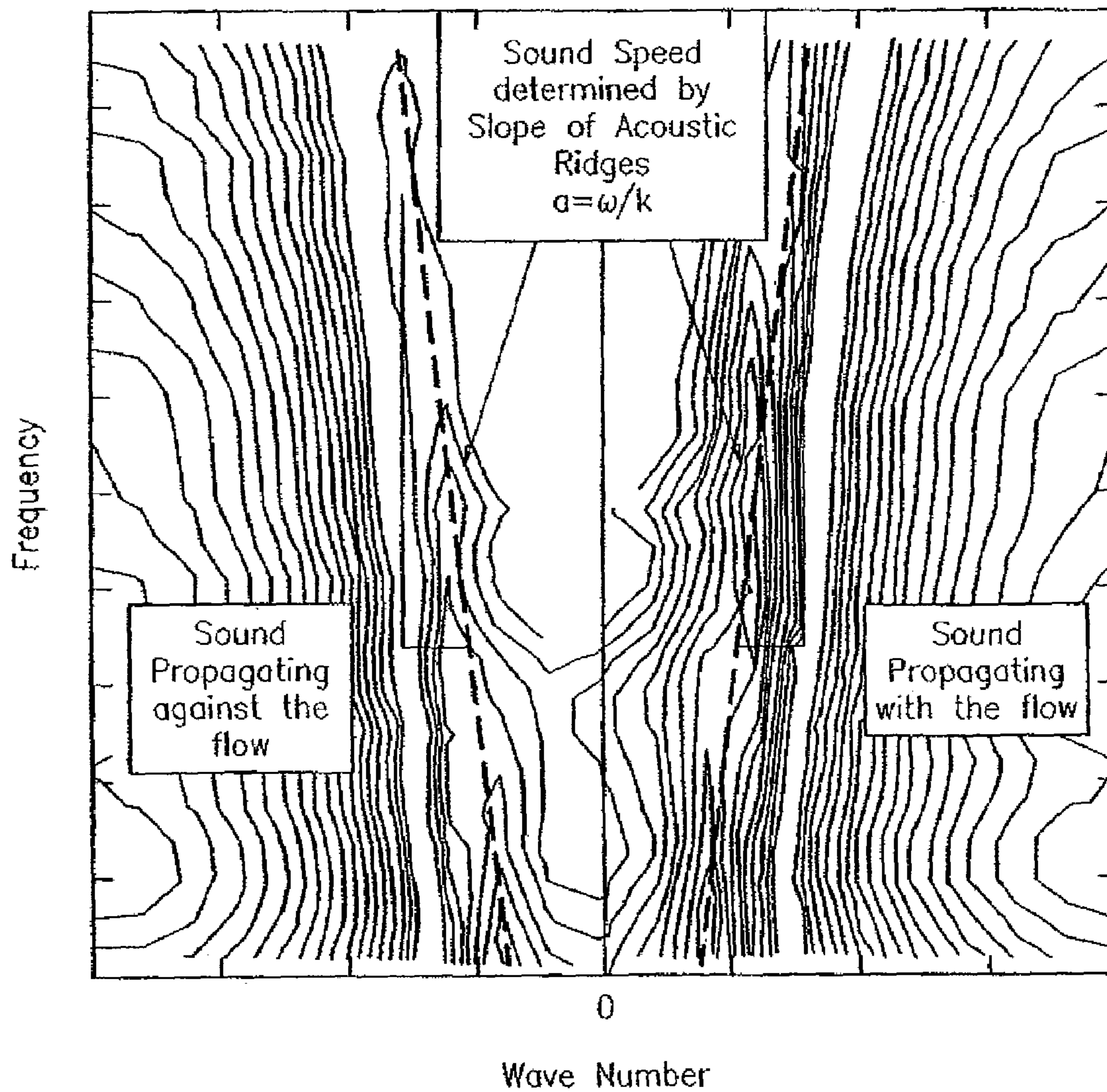
K- \omega plot showing Acoustic Ridges (in water with entrained air)
