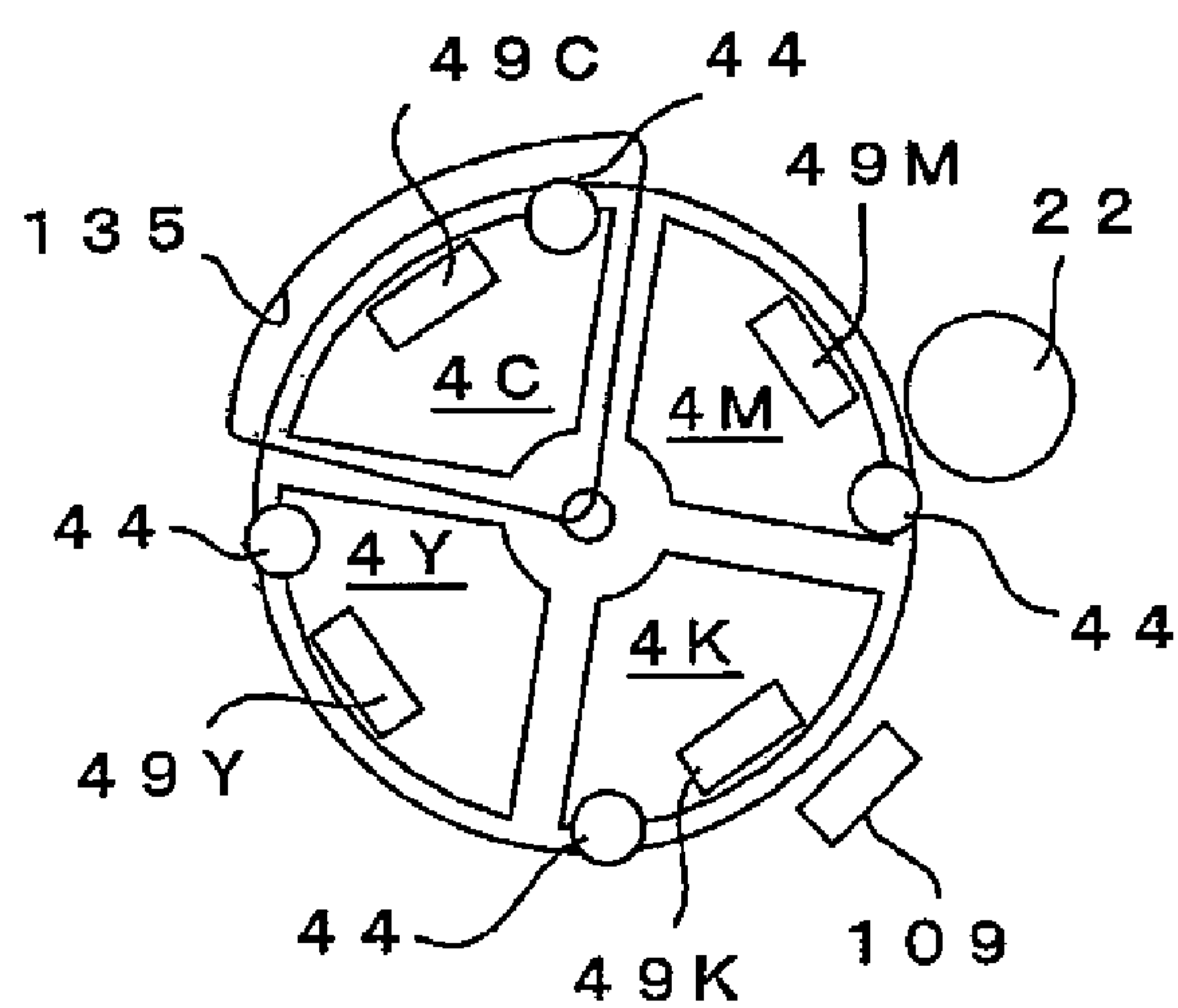
FIG. 5C : MOUNTING/DISMOUNTING POSITION
