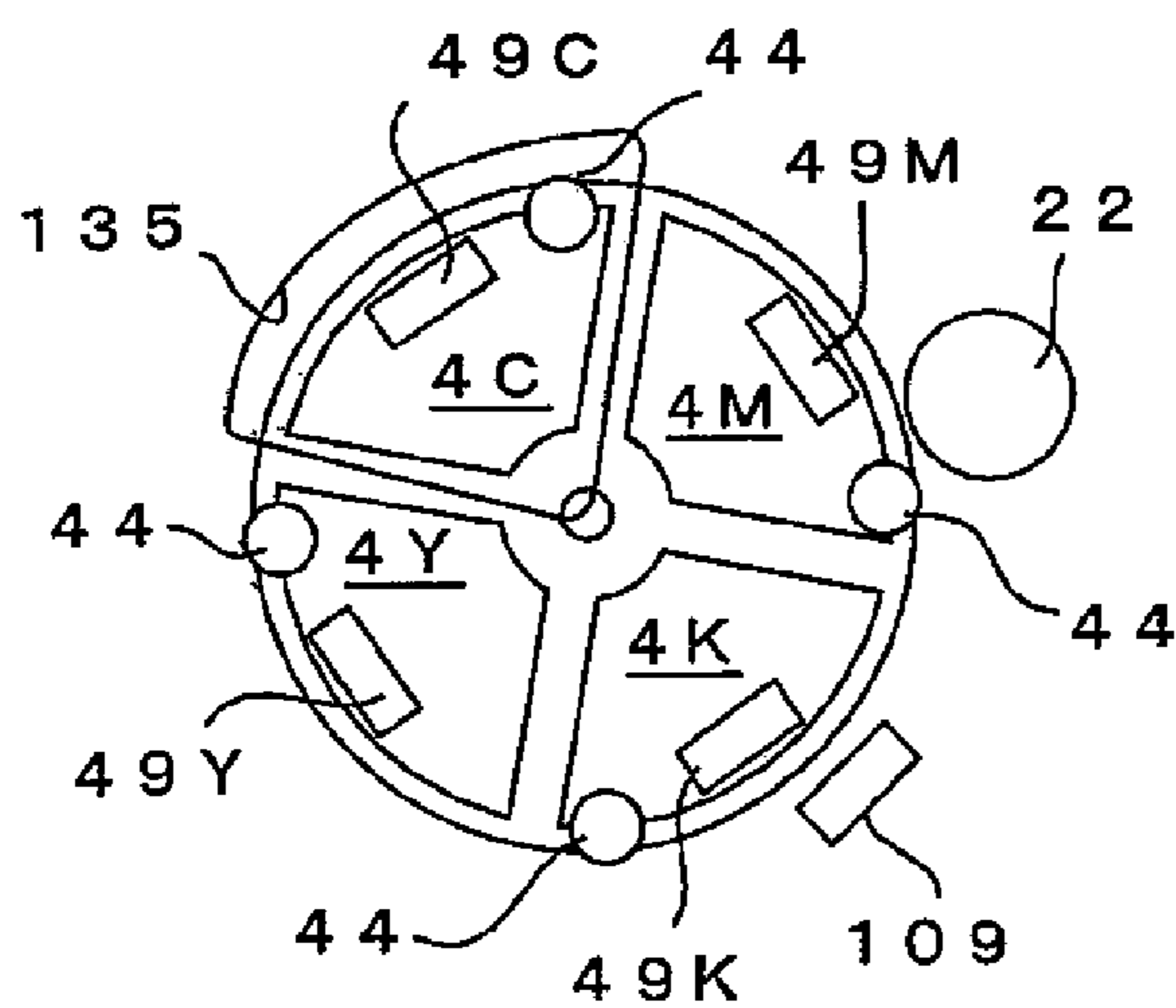
FIG. 5C : MOUNTING/DISMOUNTING POSITION
