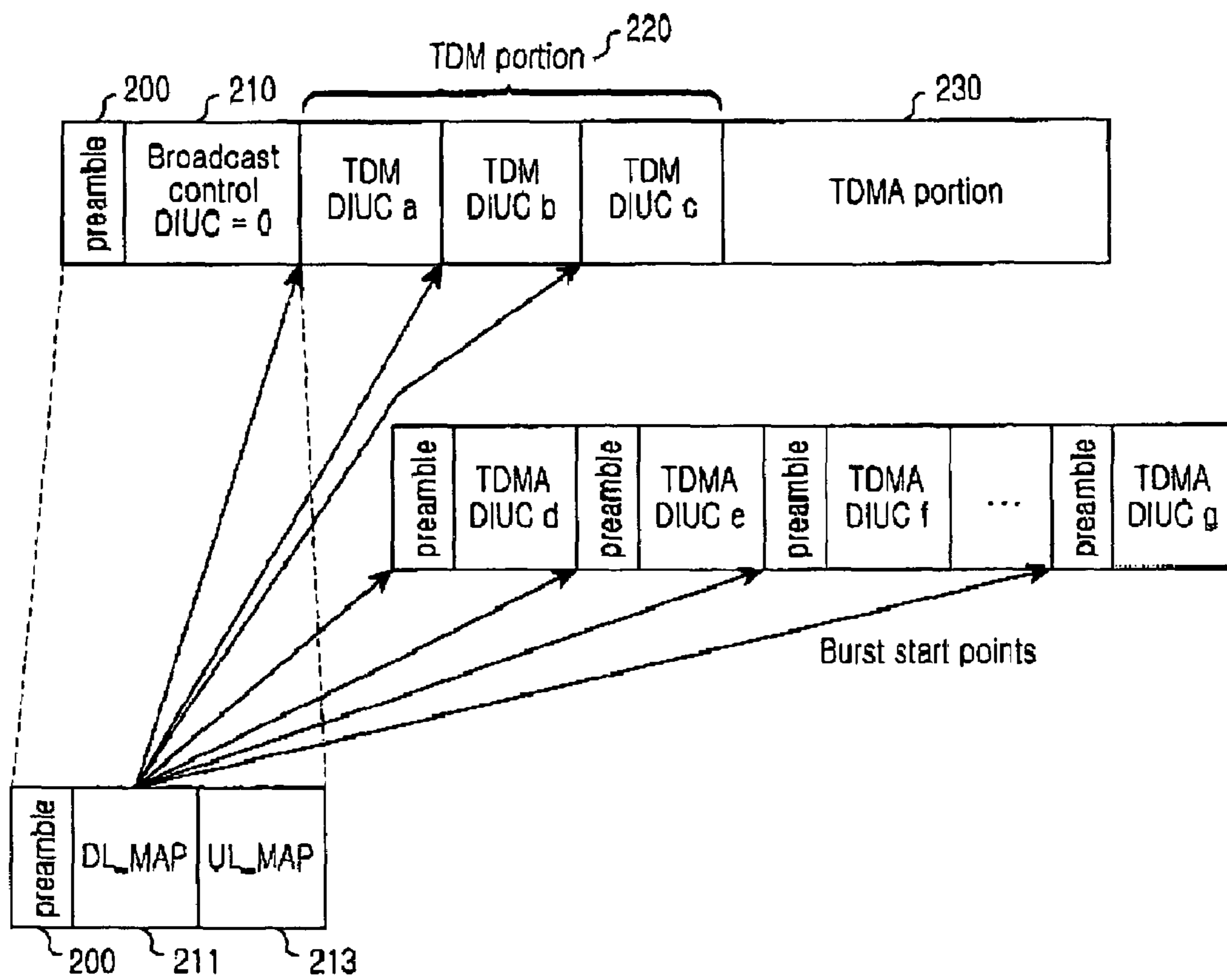
FIG.2 (PRIOR ART)
