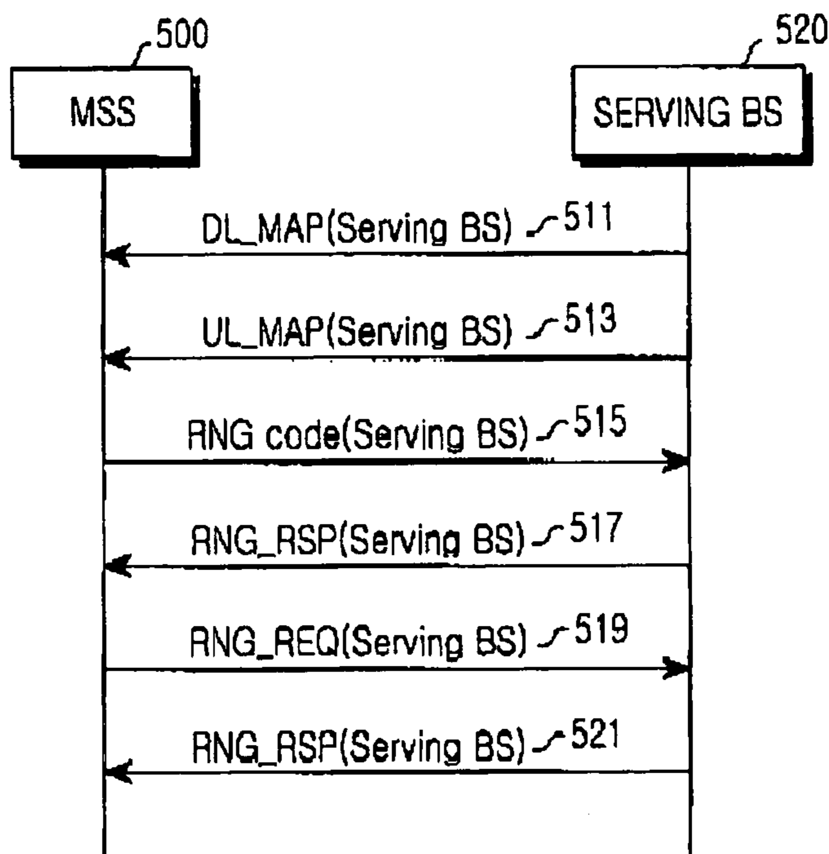
FIG.5 (PRIOR ART)
