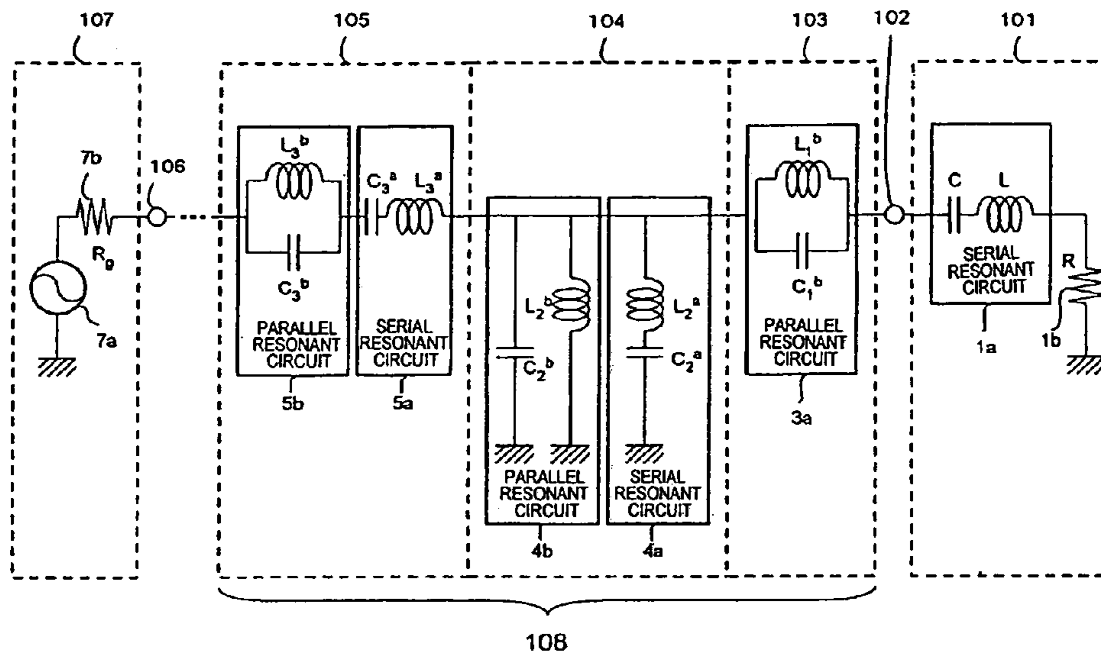
FIG. 11 - PRIOR ART -
