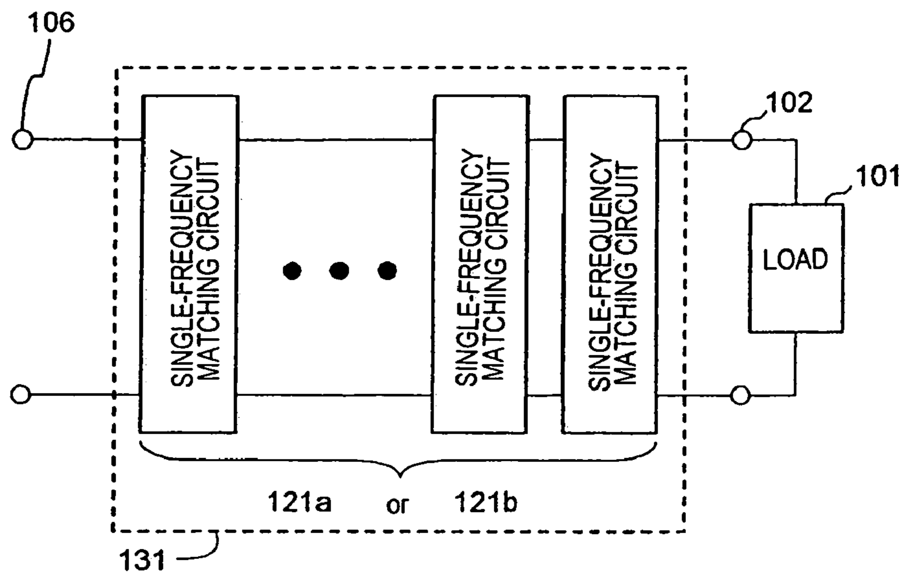
FIG. 13 – PRIOR ART –
