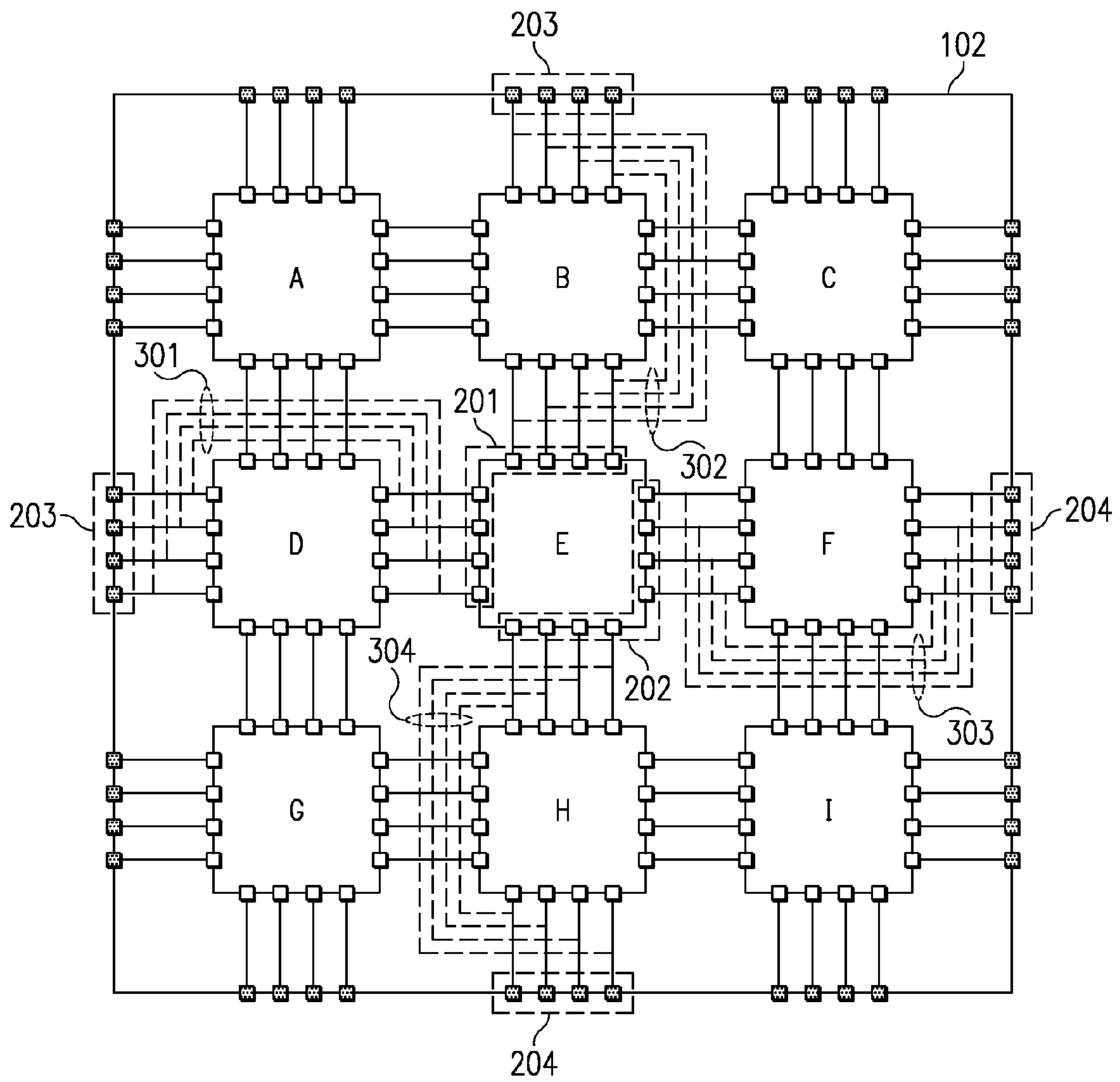
FIG. 3 (PRIOR ART)
