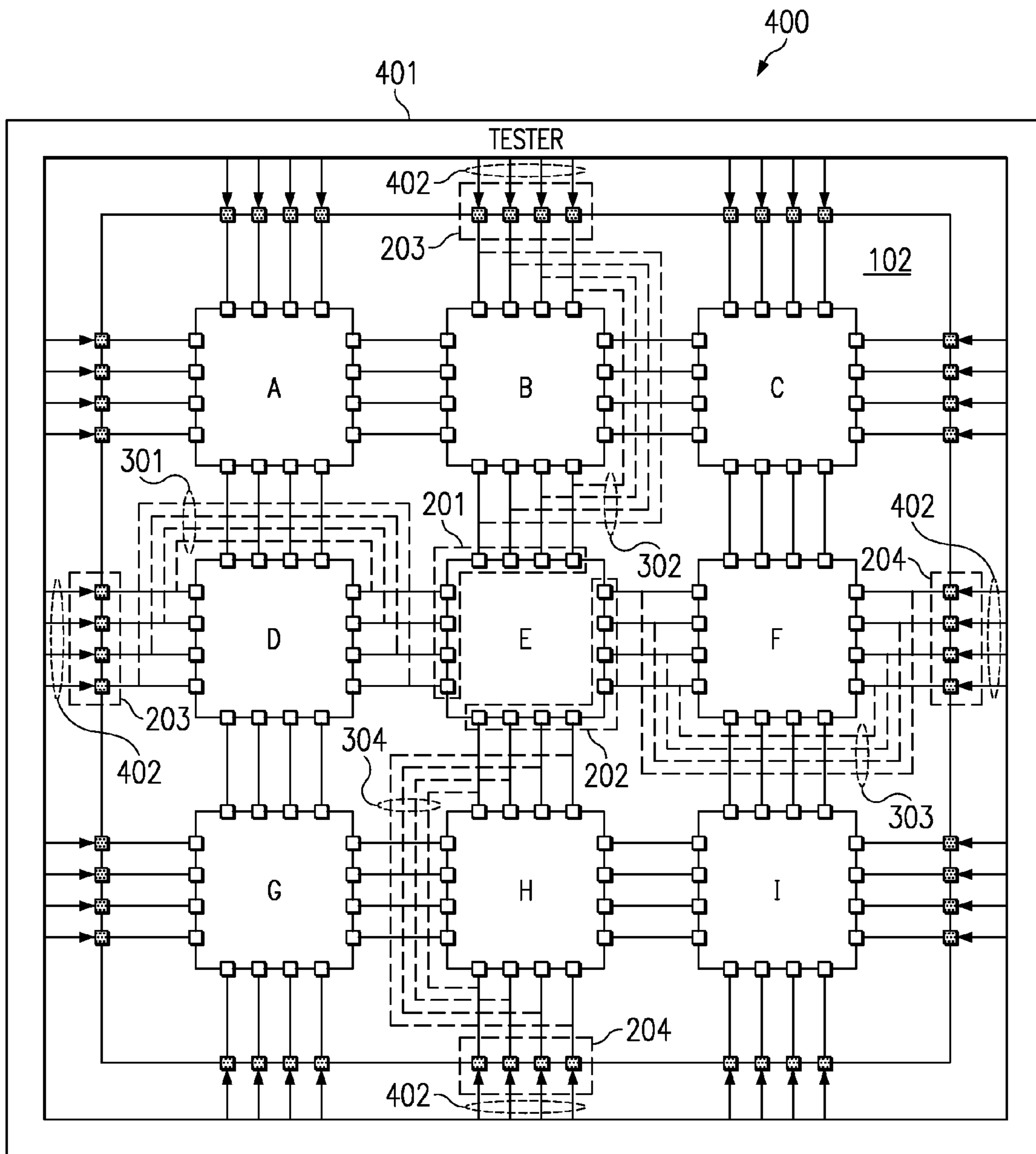
FIG. 4 (PRIOR ART)
