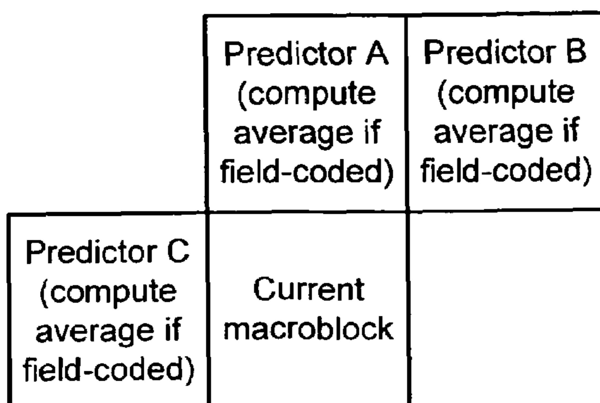
Figure 5, prior art
