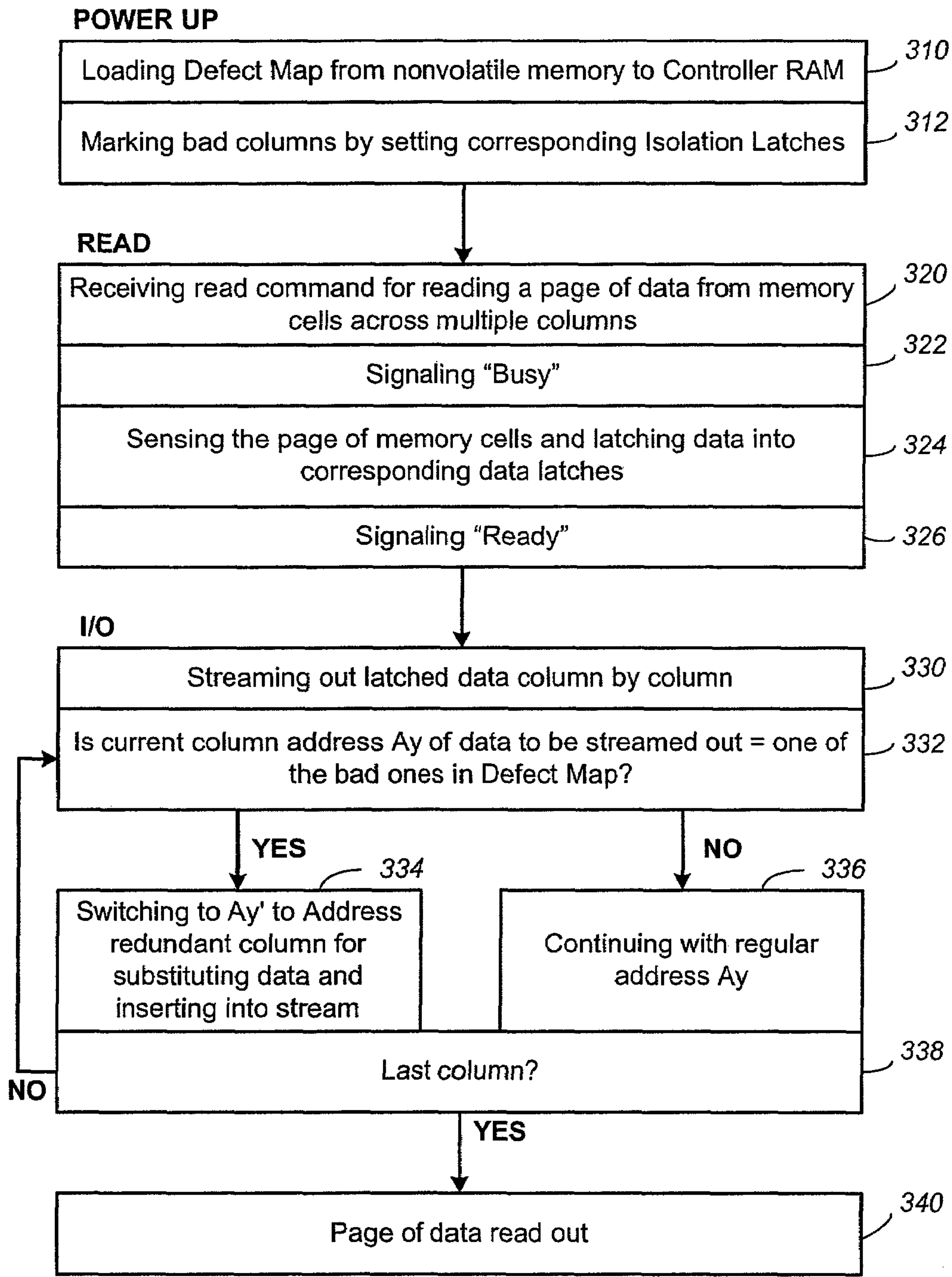
READ OPERATION (Prior Art)
