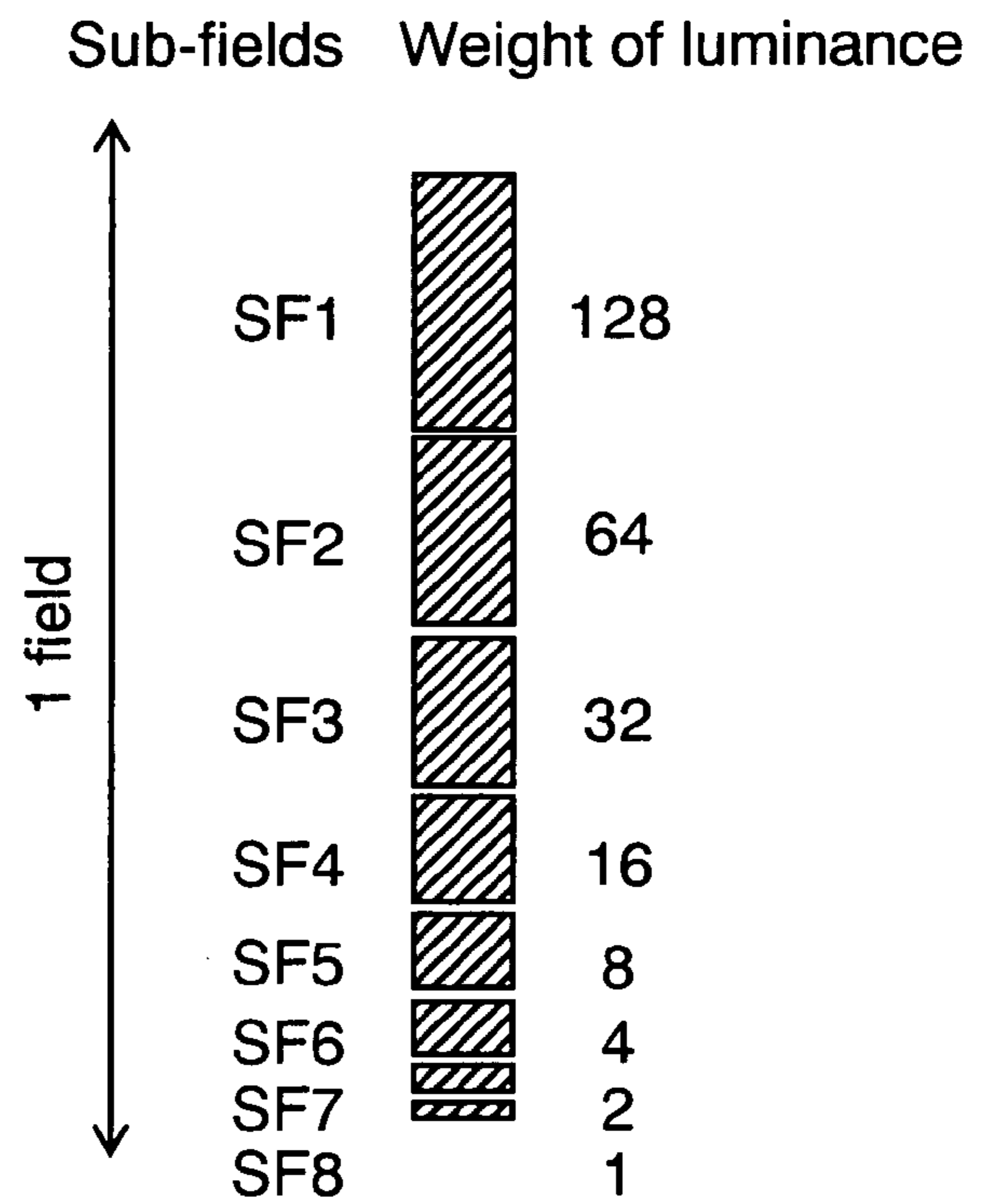
Descending coding
