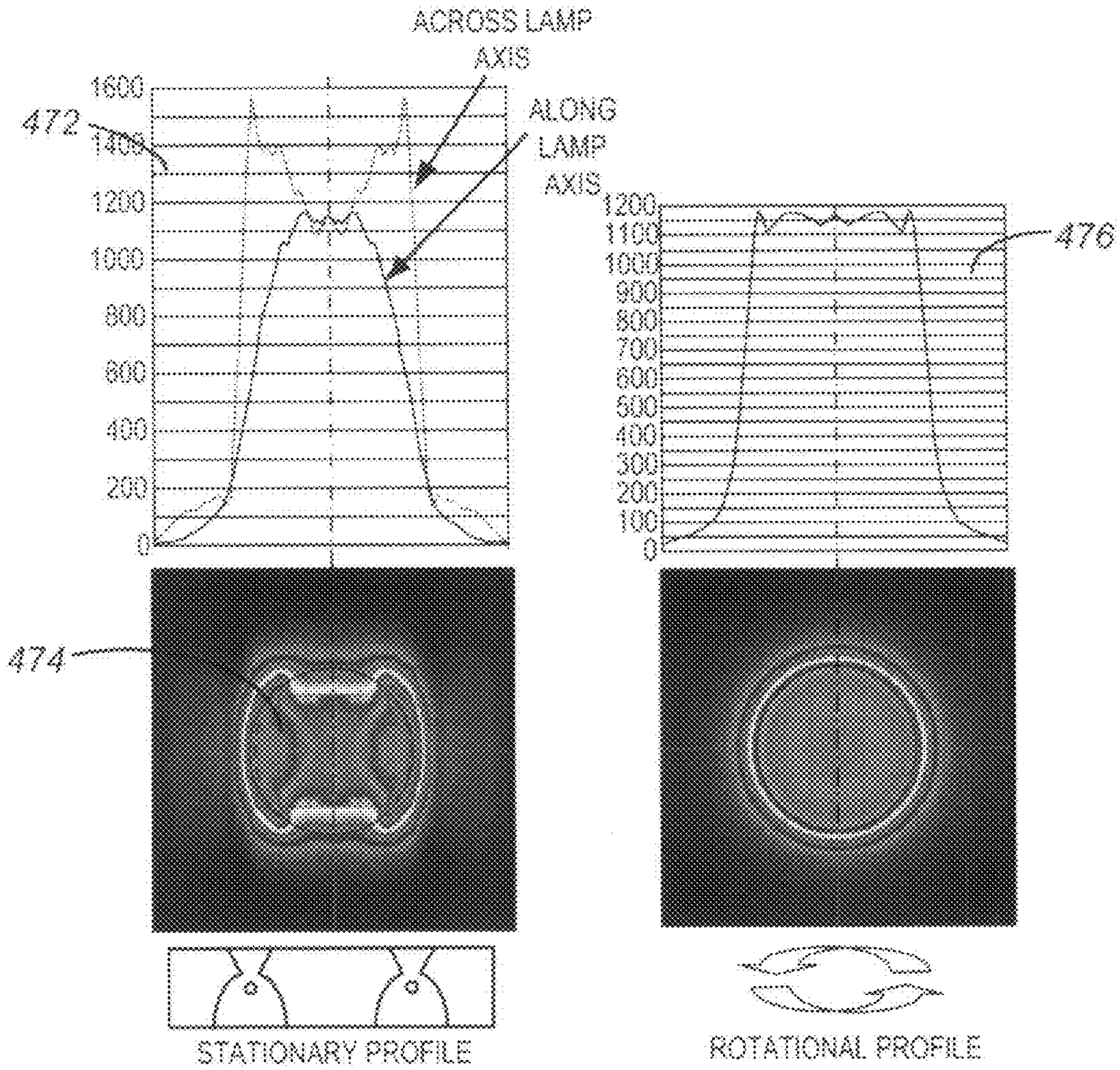
Primary (asymmetric) + Secondary Reflector - dual lamp
