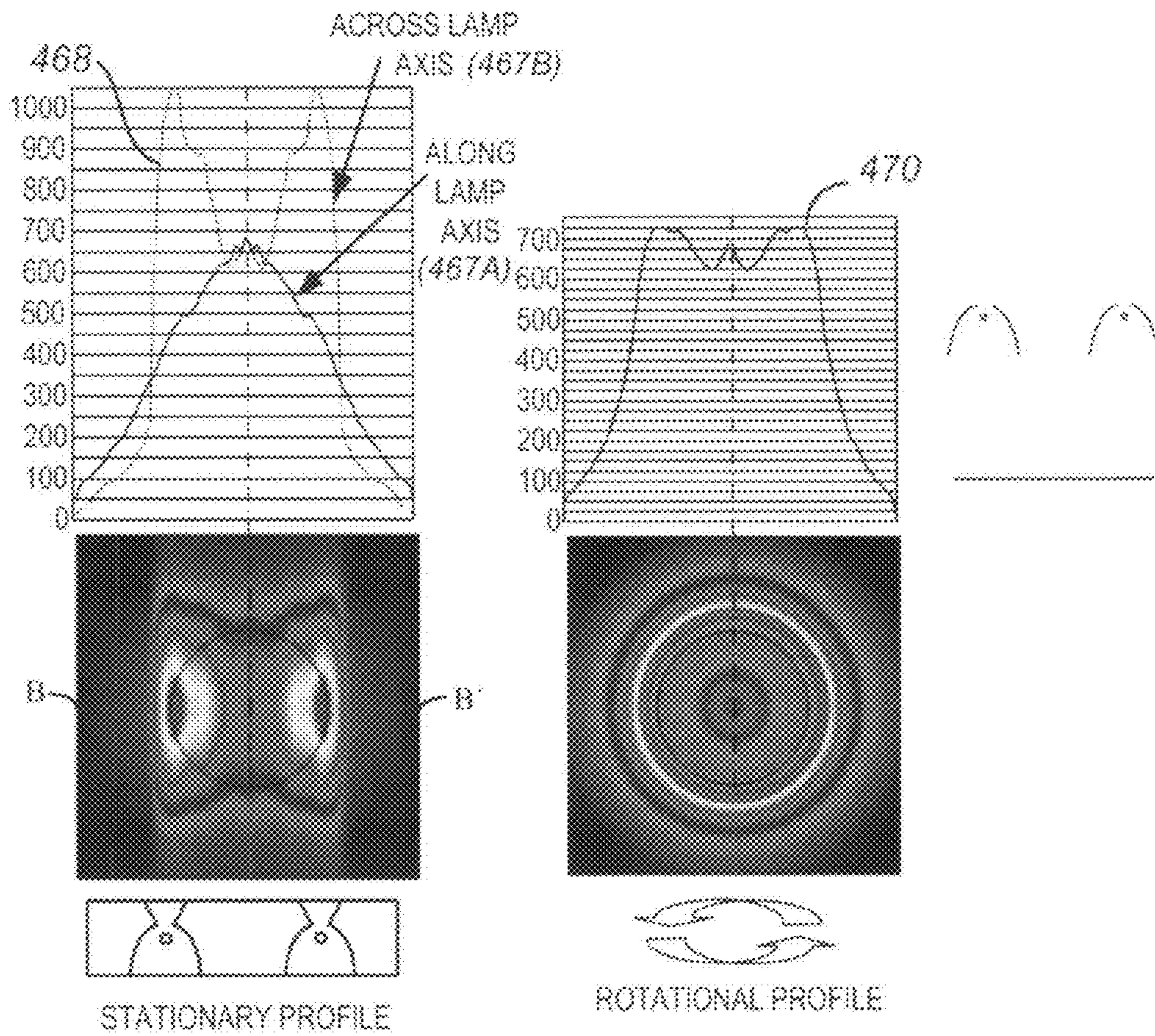
Primary Reflector (asymmetric) - dual lamp
