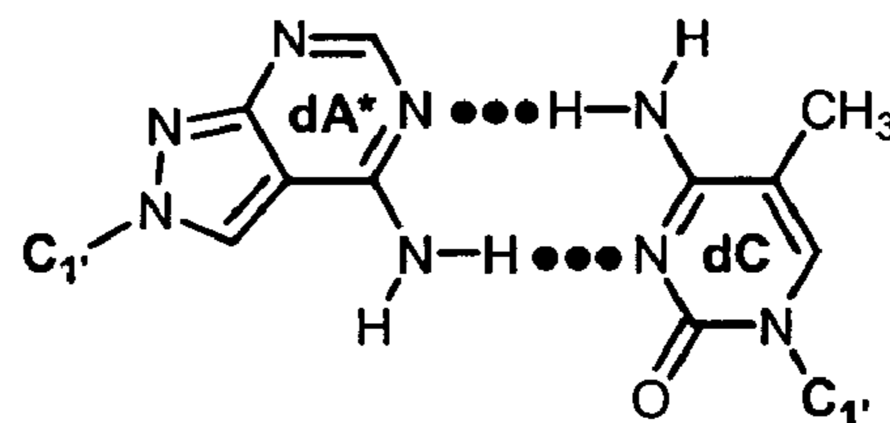
reversed Watson-Crick
