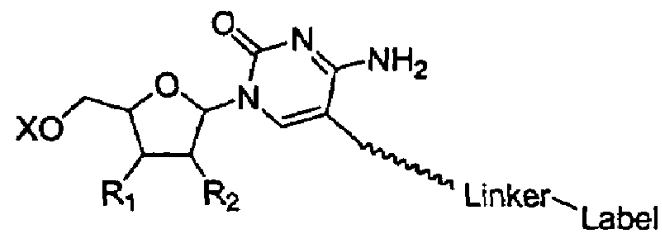
Cytidine C5-linker
