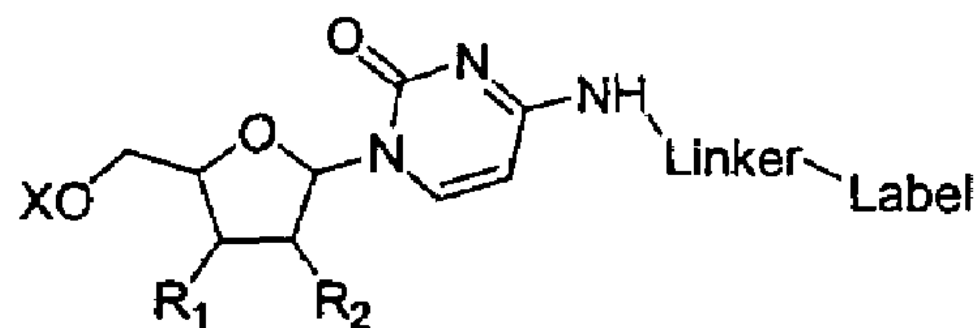
Cytidine N4-linker
