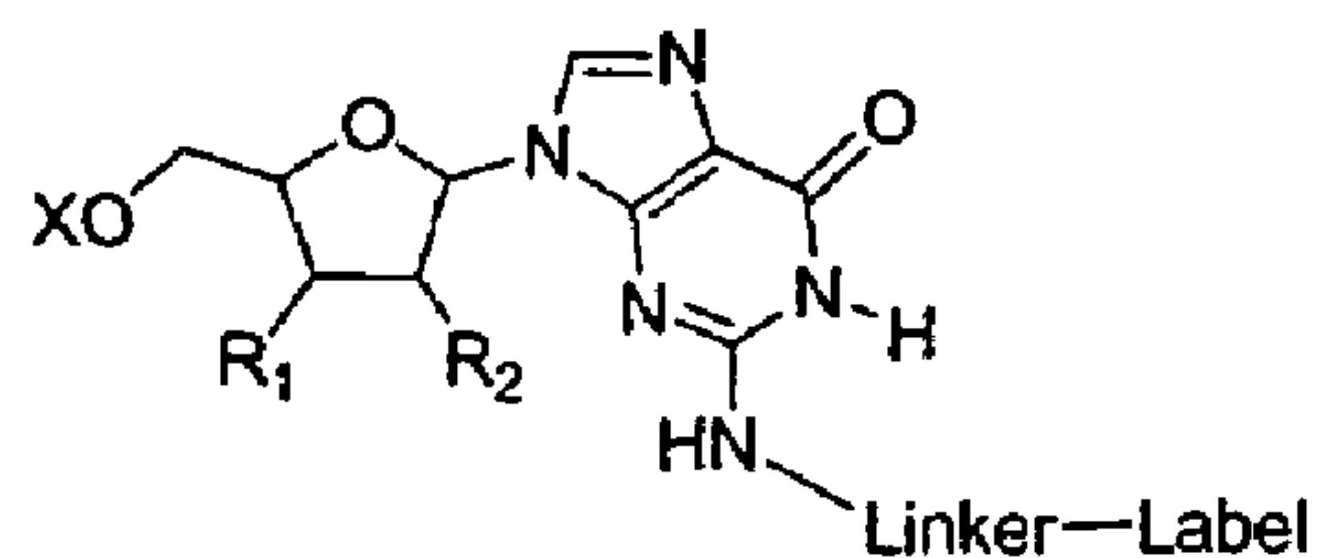
Guanosine N2-linker
