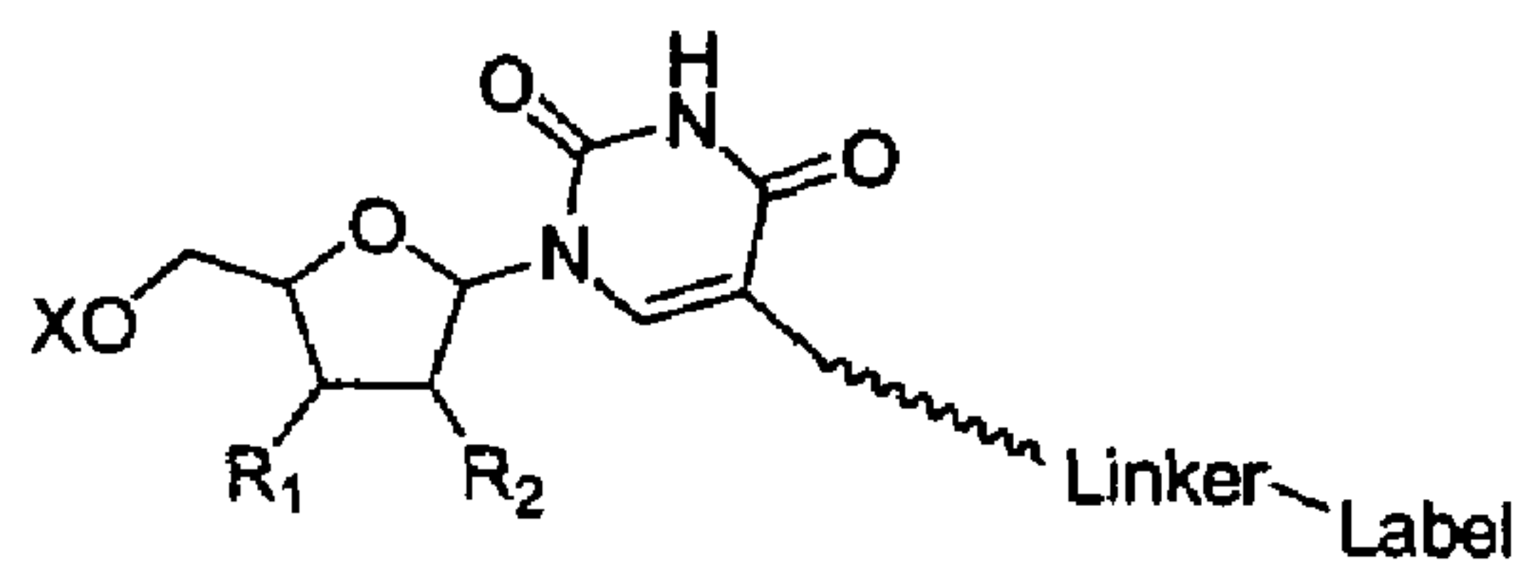
Uridine C5-linker
