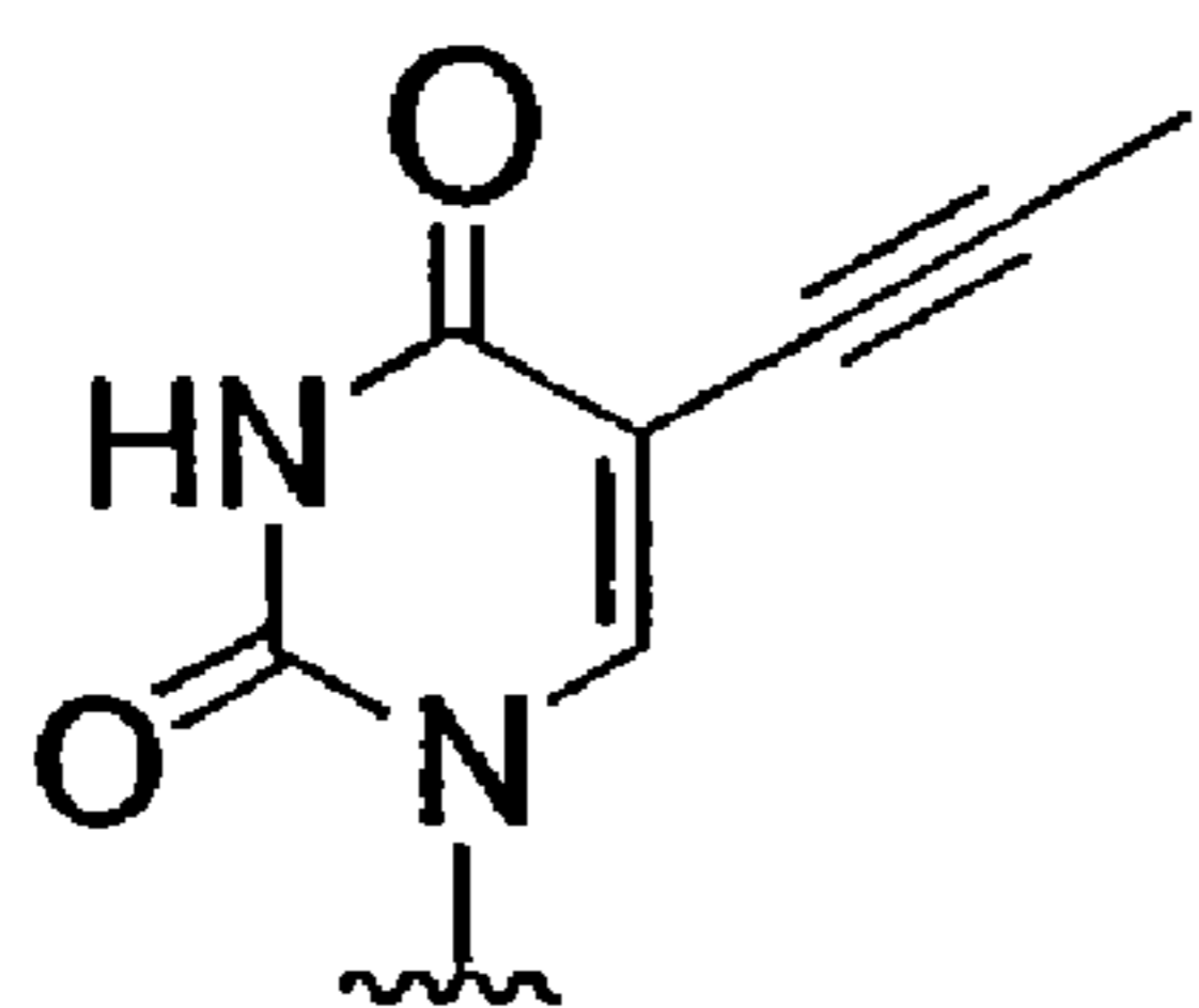
5-propynyl-U
