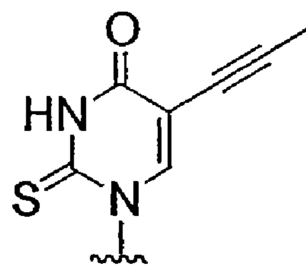
2-thio-5-propynyl-U
