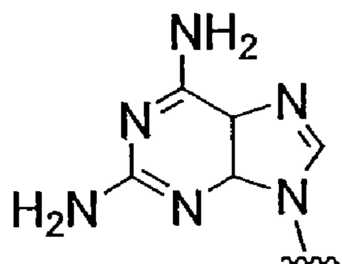
N9-(2,6,-diaminopurine)
