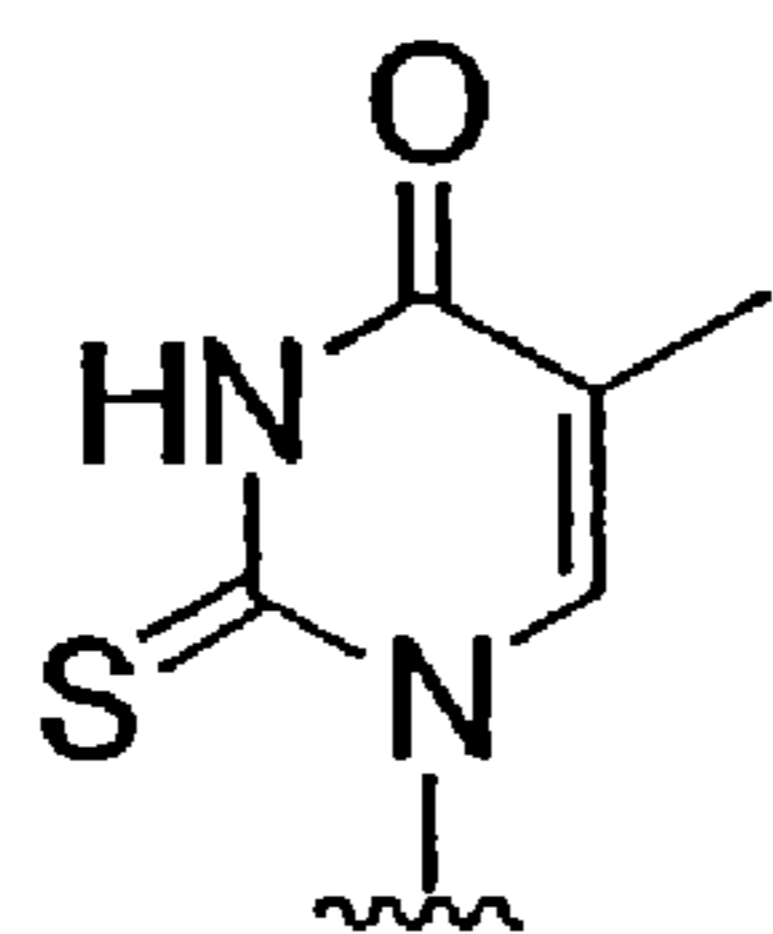
2-thio-T
