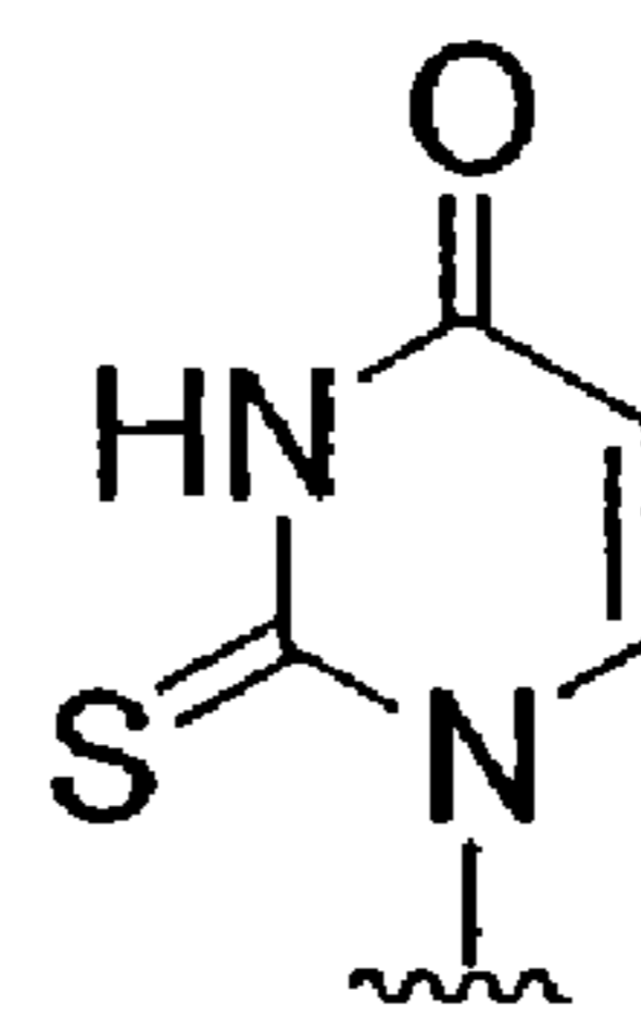
2-thio-U
