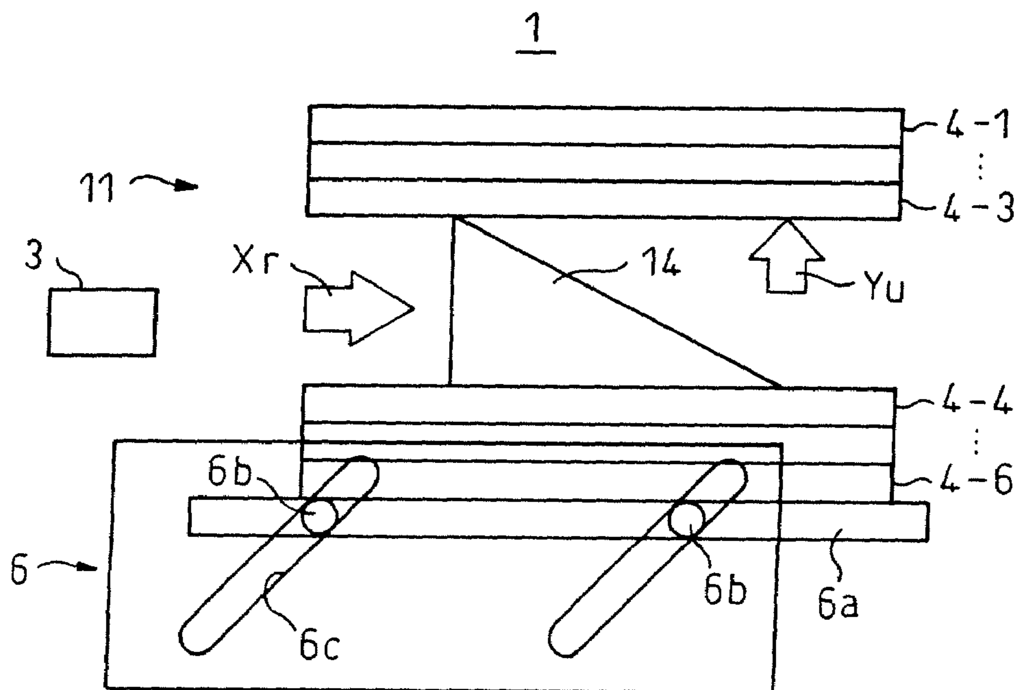
FIG.2 PRIOR ART
