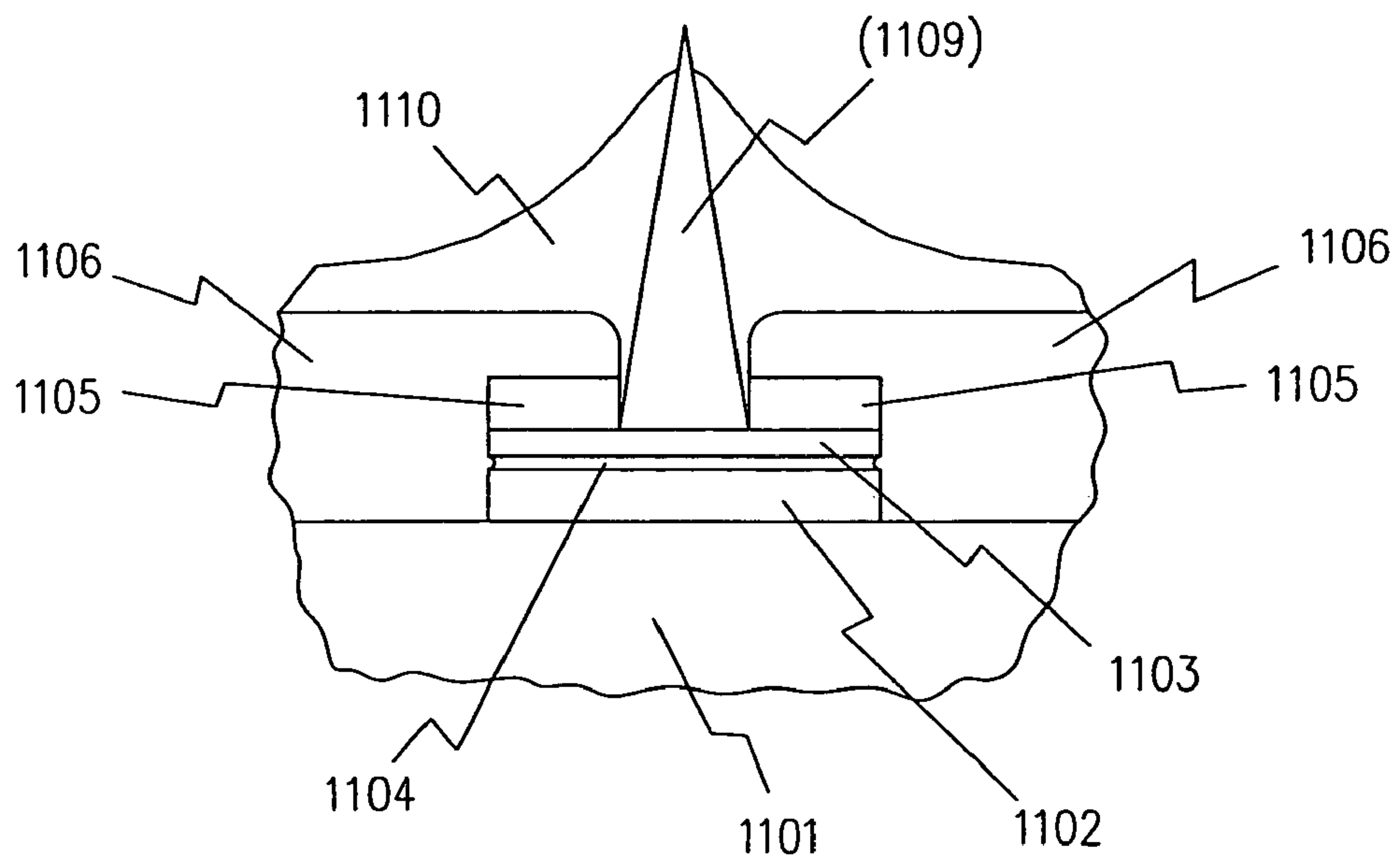
FIGURE 11b ELECTRODES
