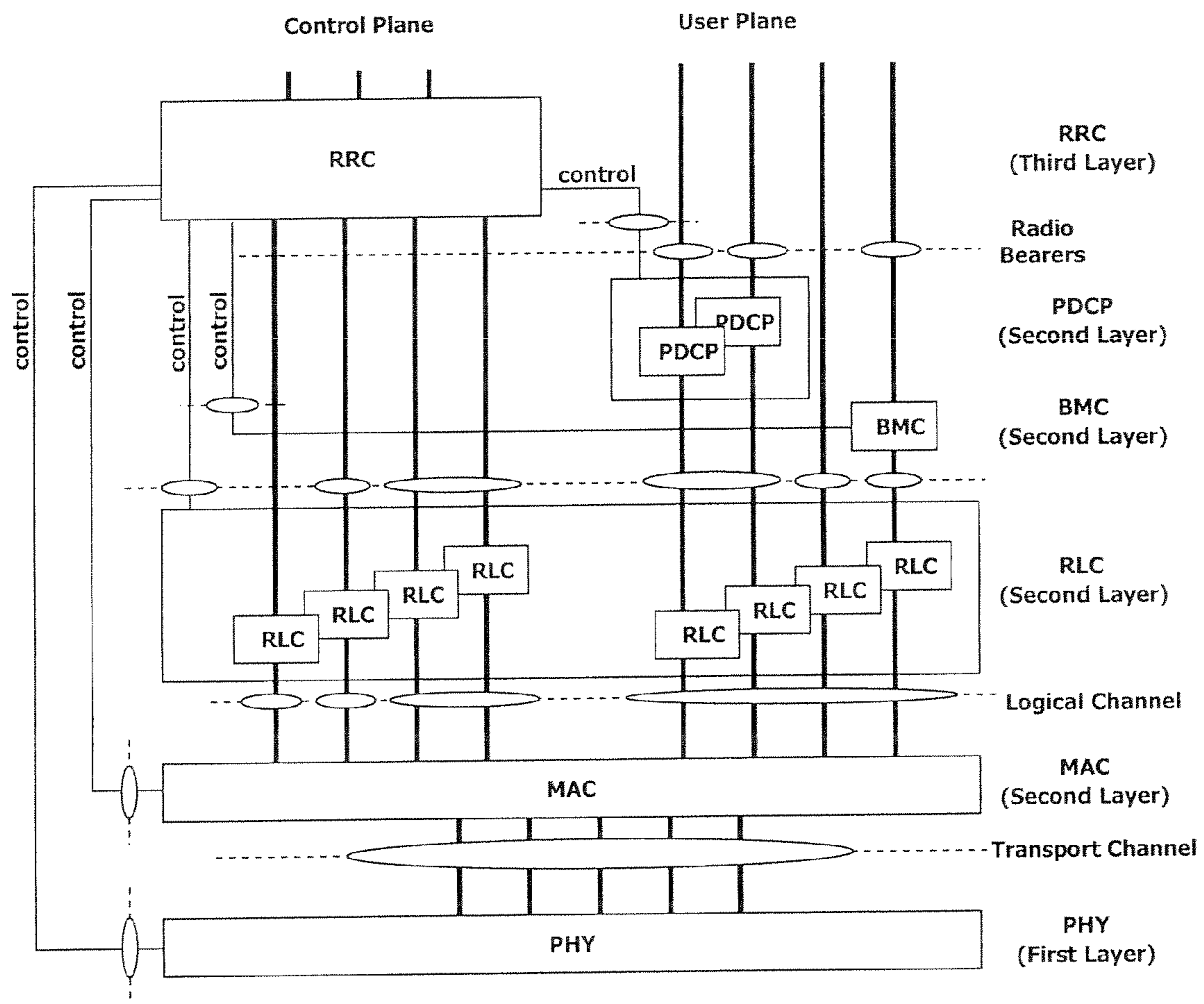
FIG.1 BACKGROUND ART
