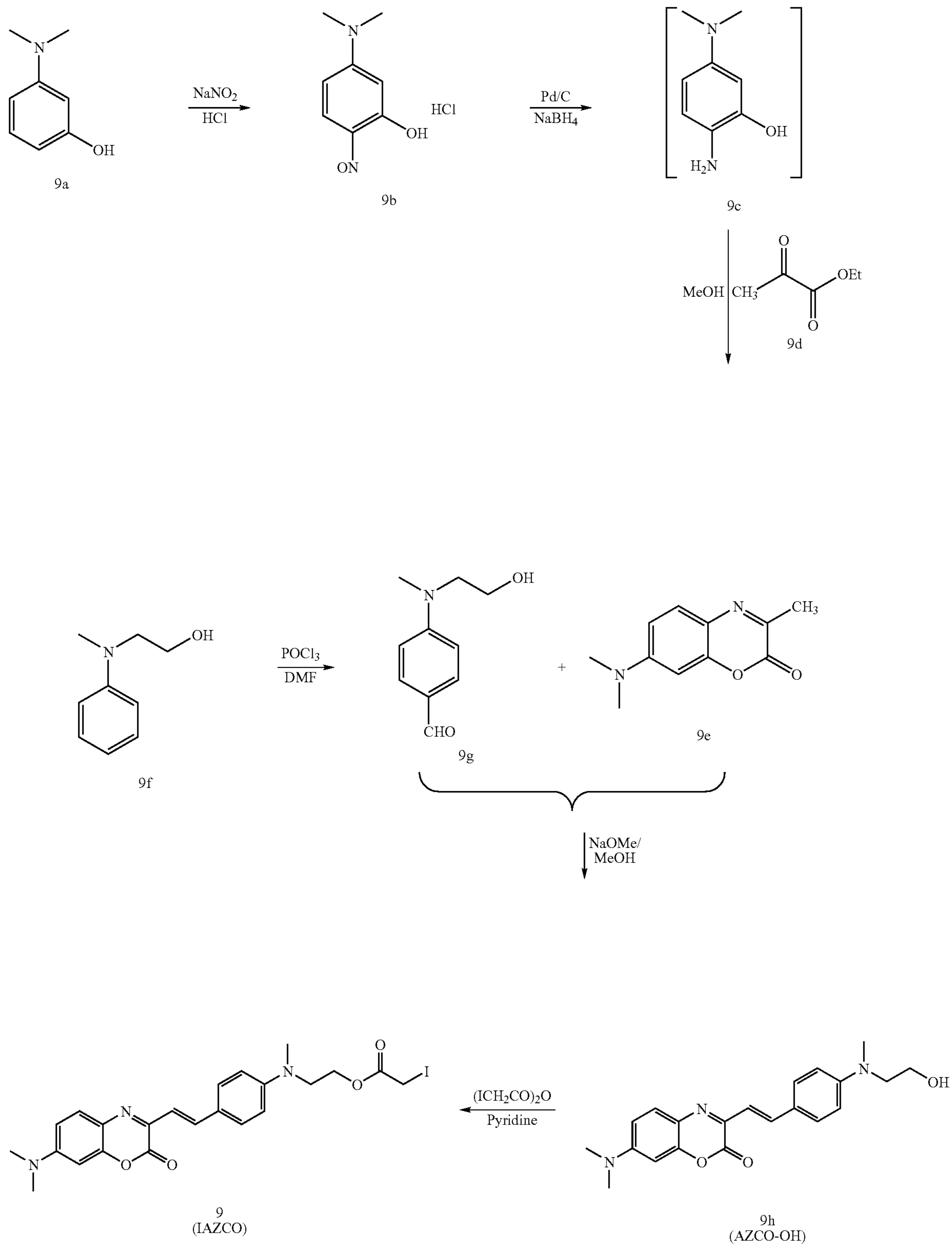
Scheme VIII
