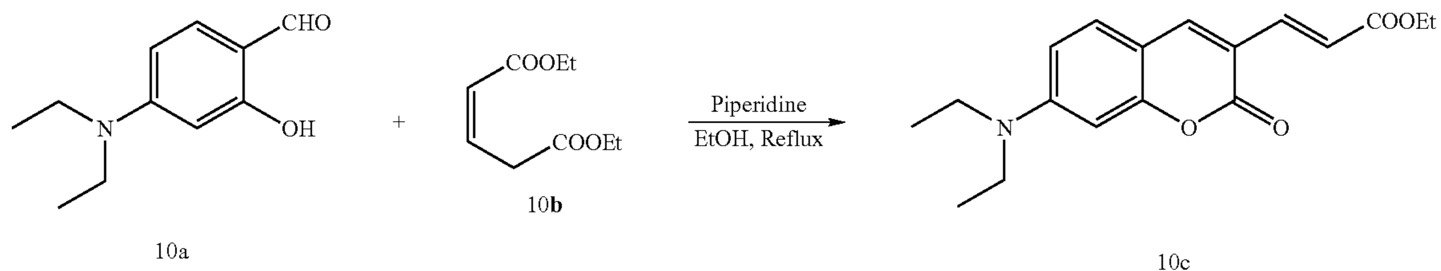
Scheme IX
