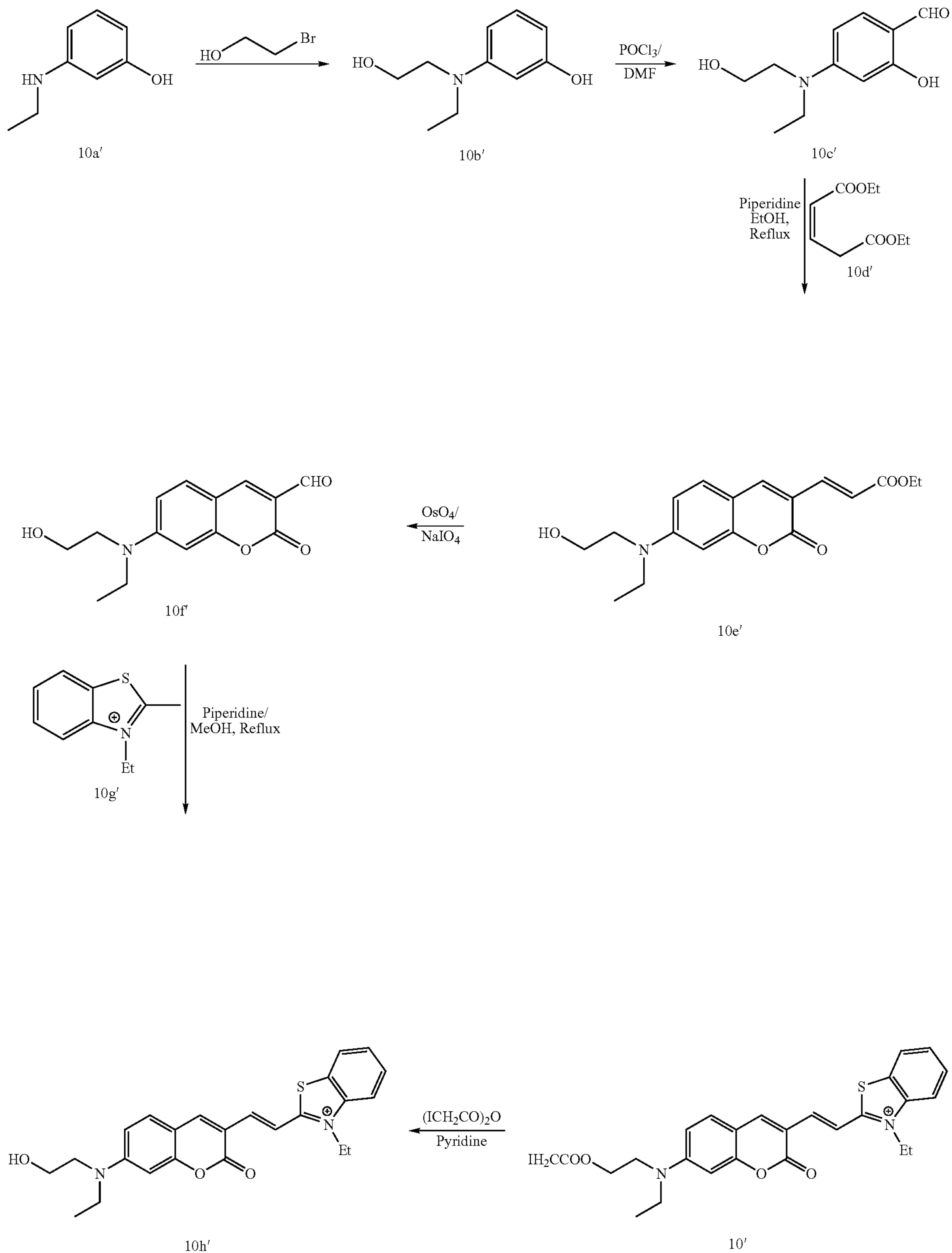
Scheme IXa
