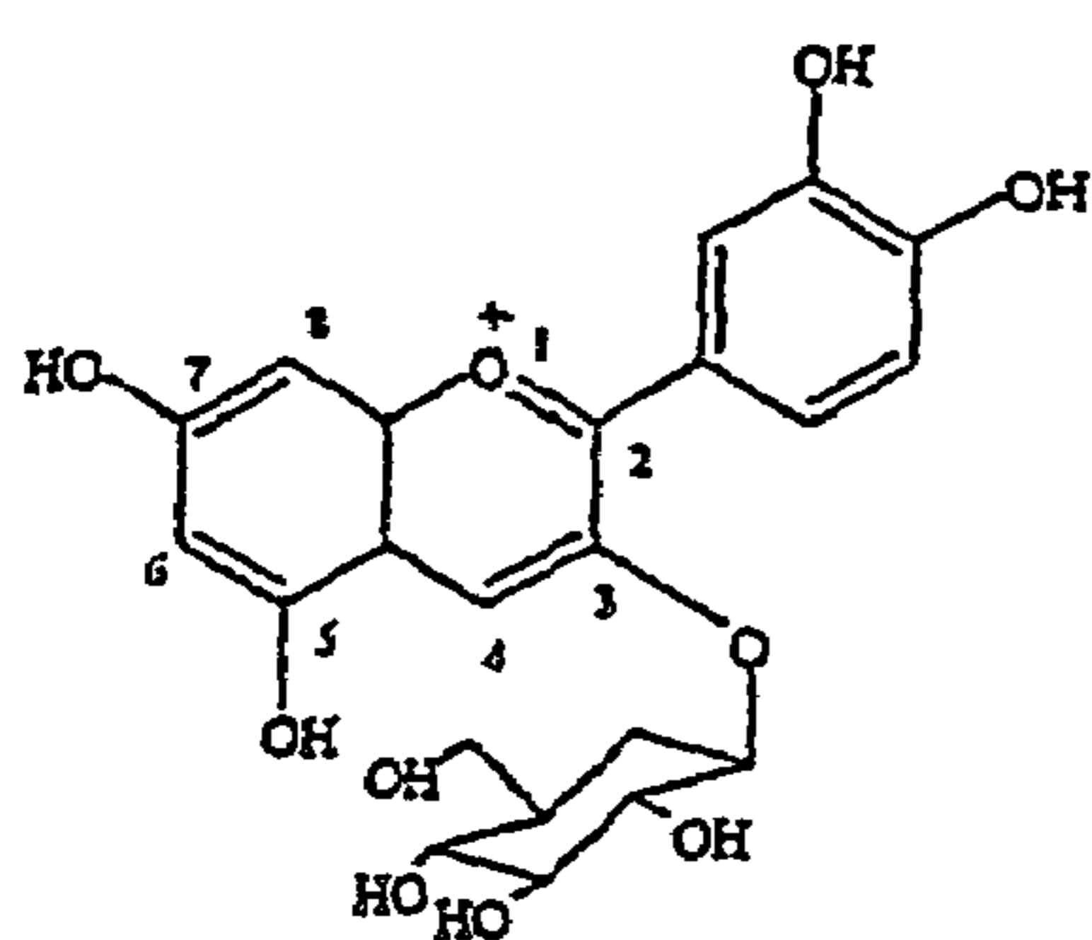
I: Cyanidin-3-glucoside
