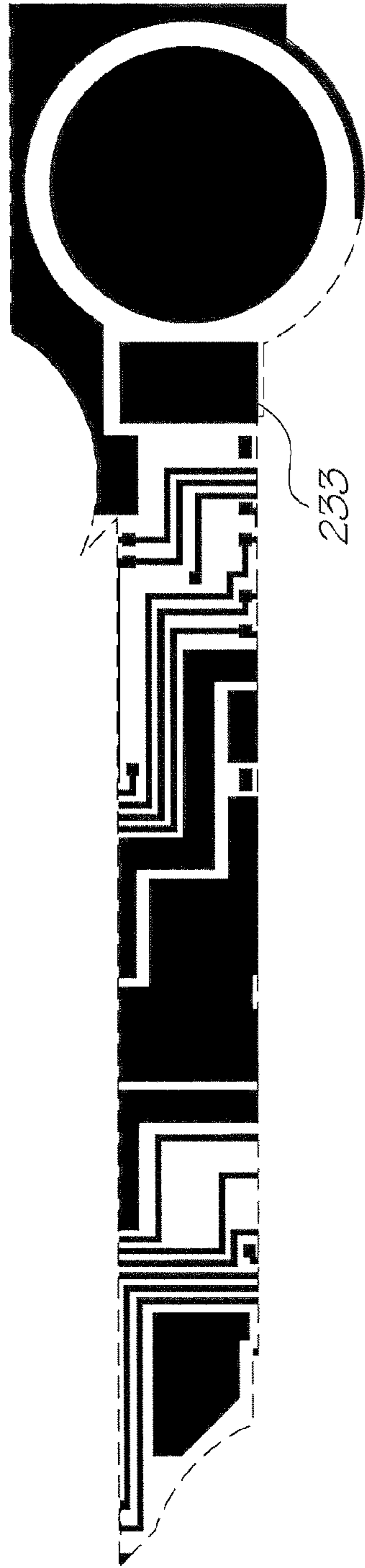
Metal 2 mask
