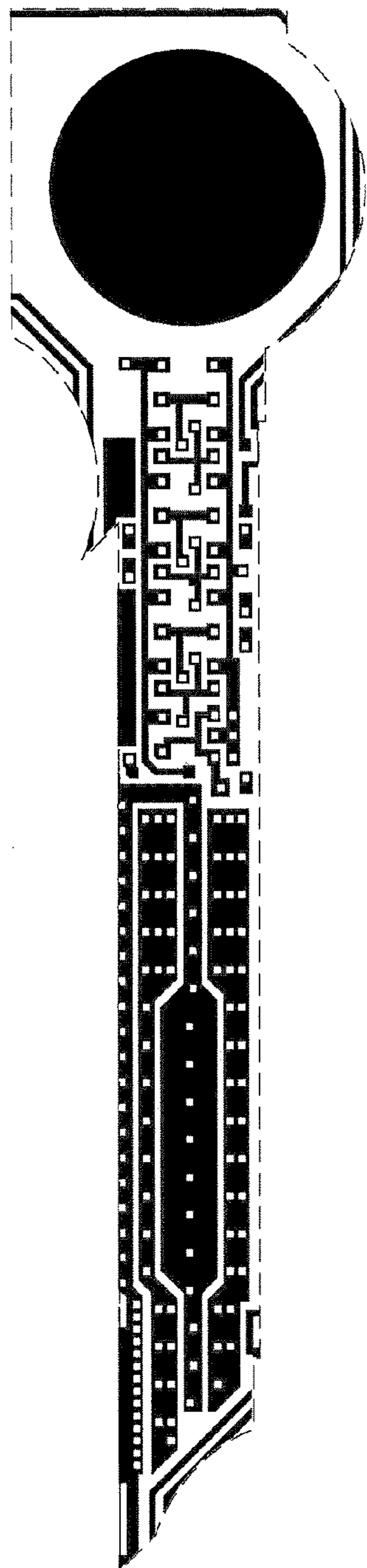
Metal 1 mask
