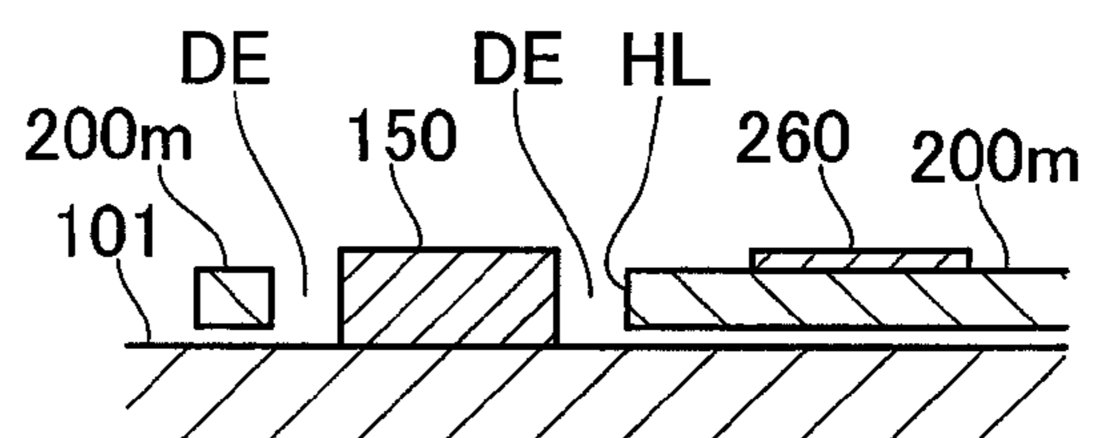
B-B CROSS SECTION
