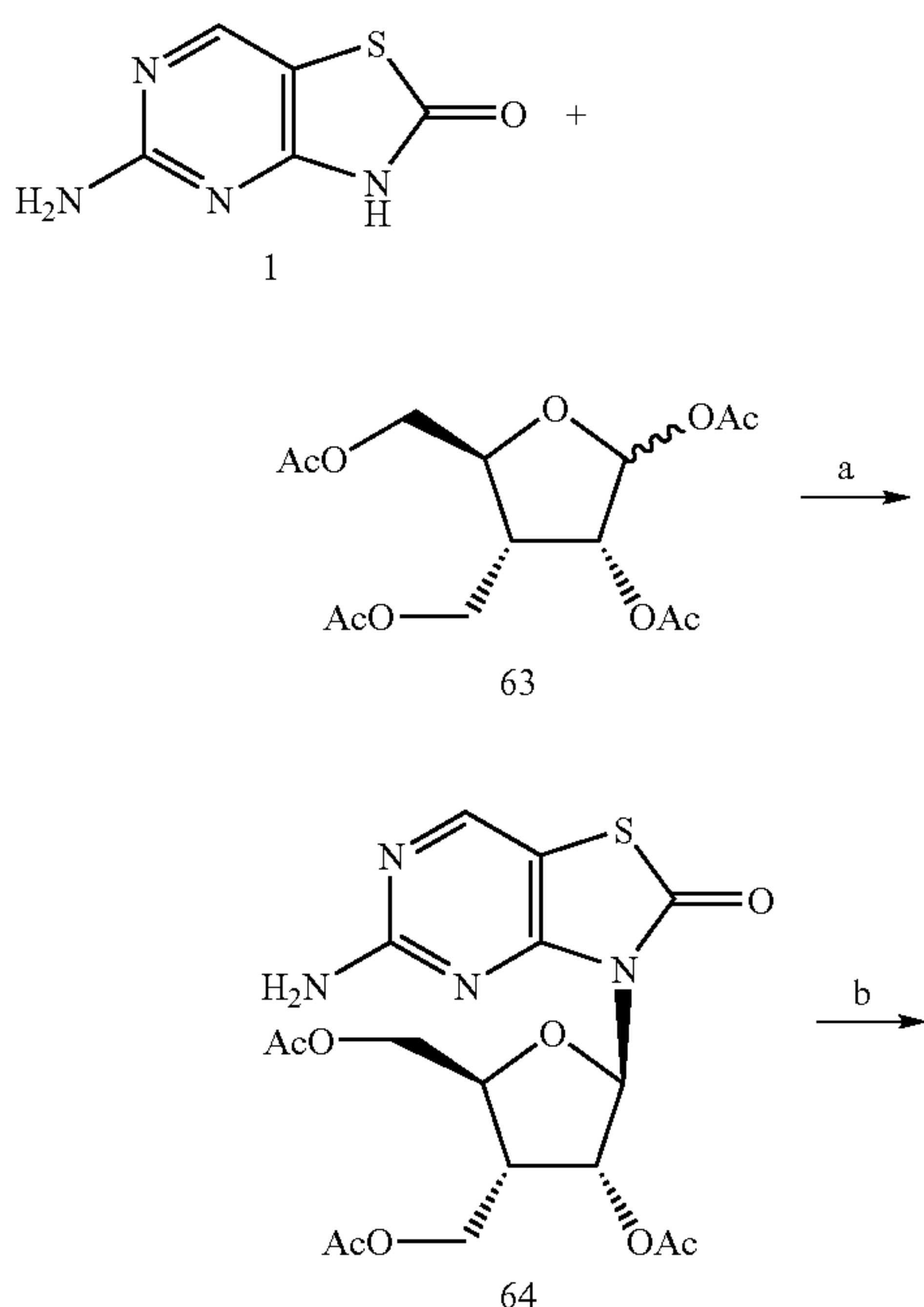
Scheme 3
