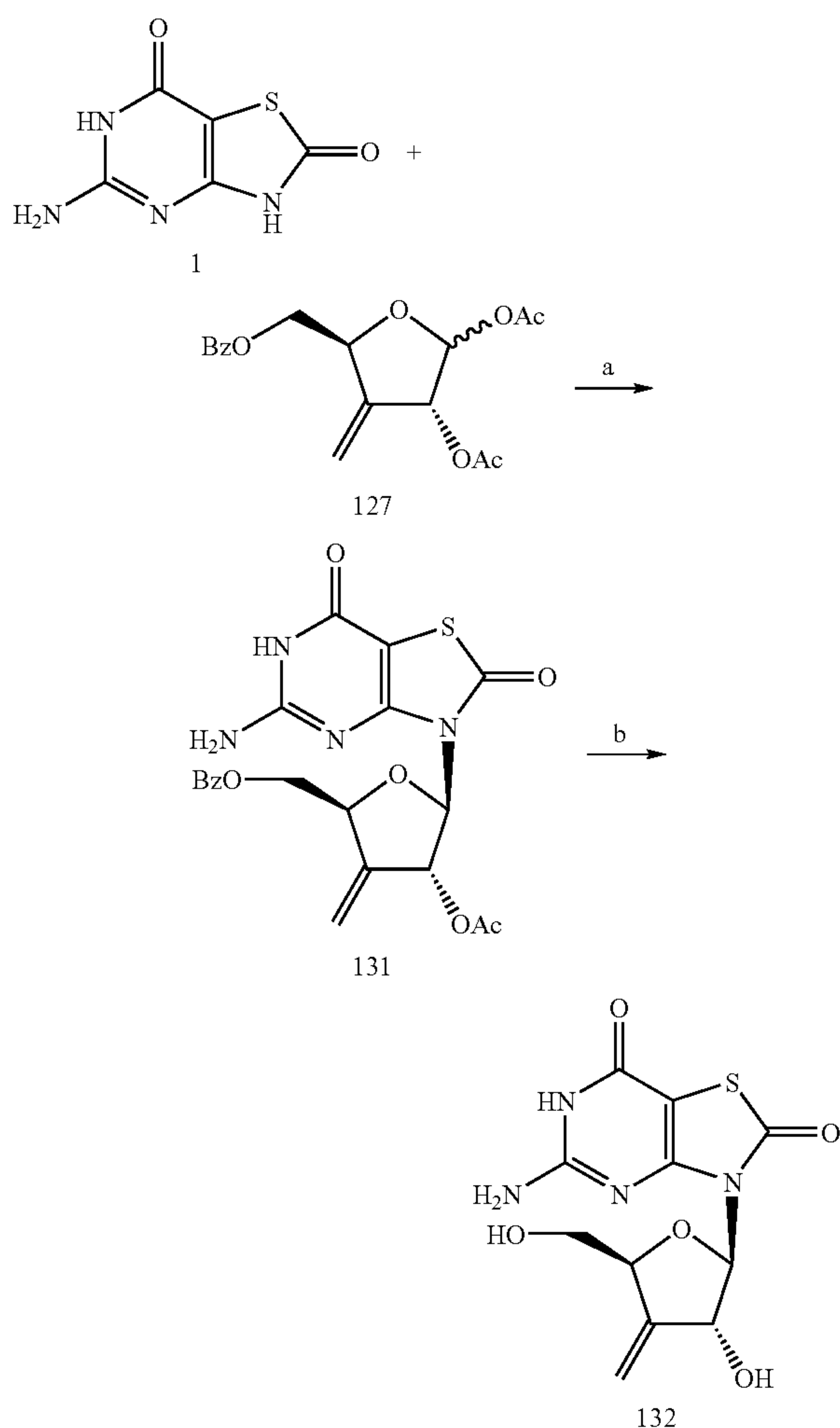
Scheme 7
