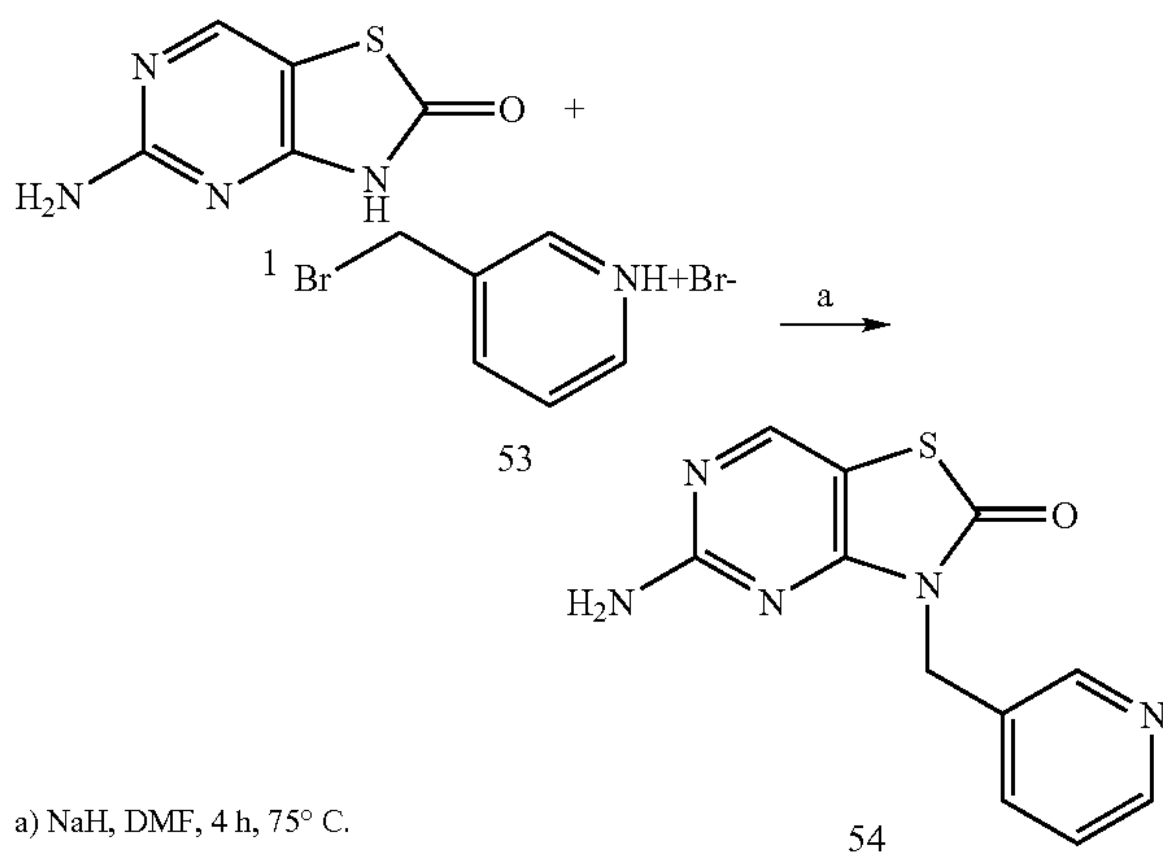
Scheme 1
