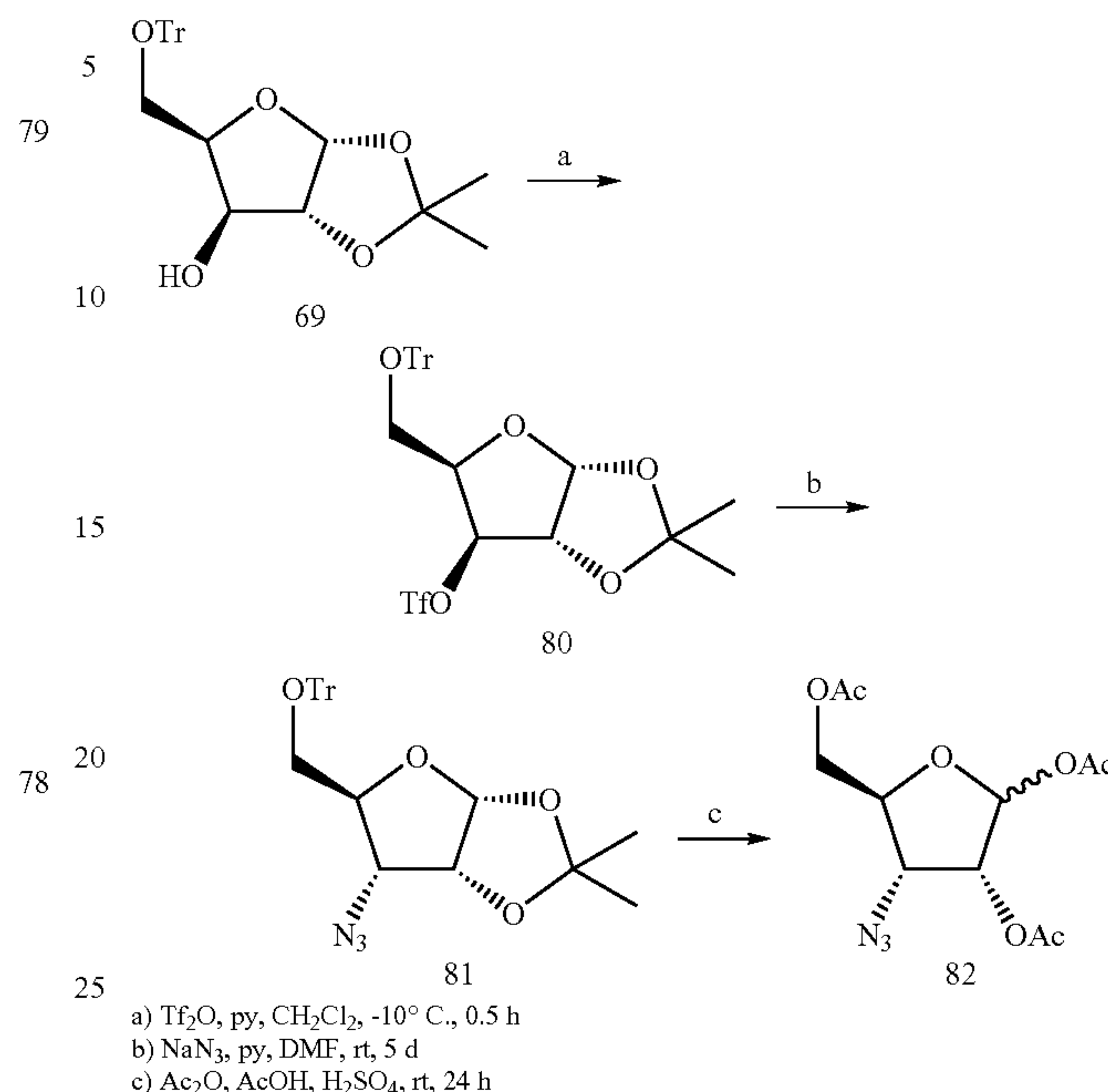
Scheme 5
