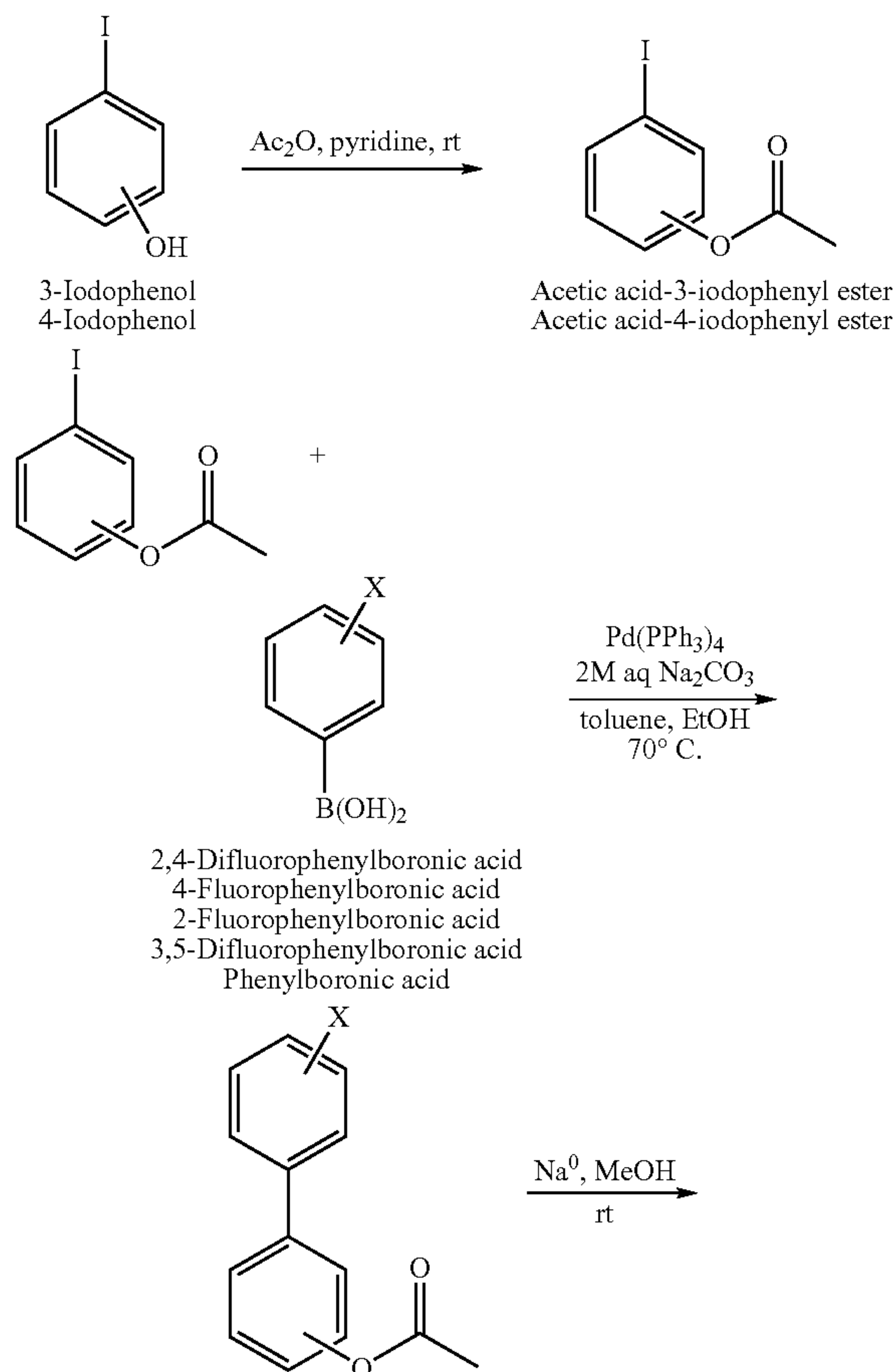
Scheme 1
