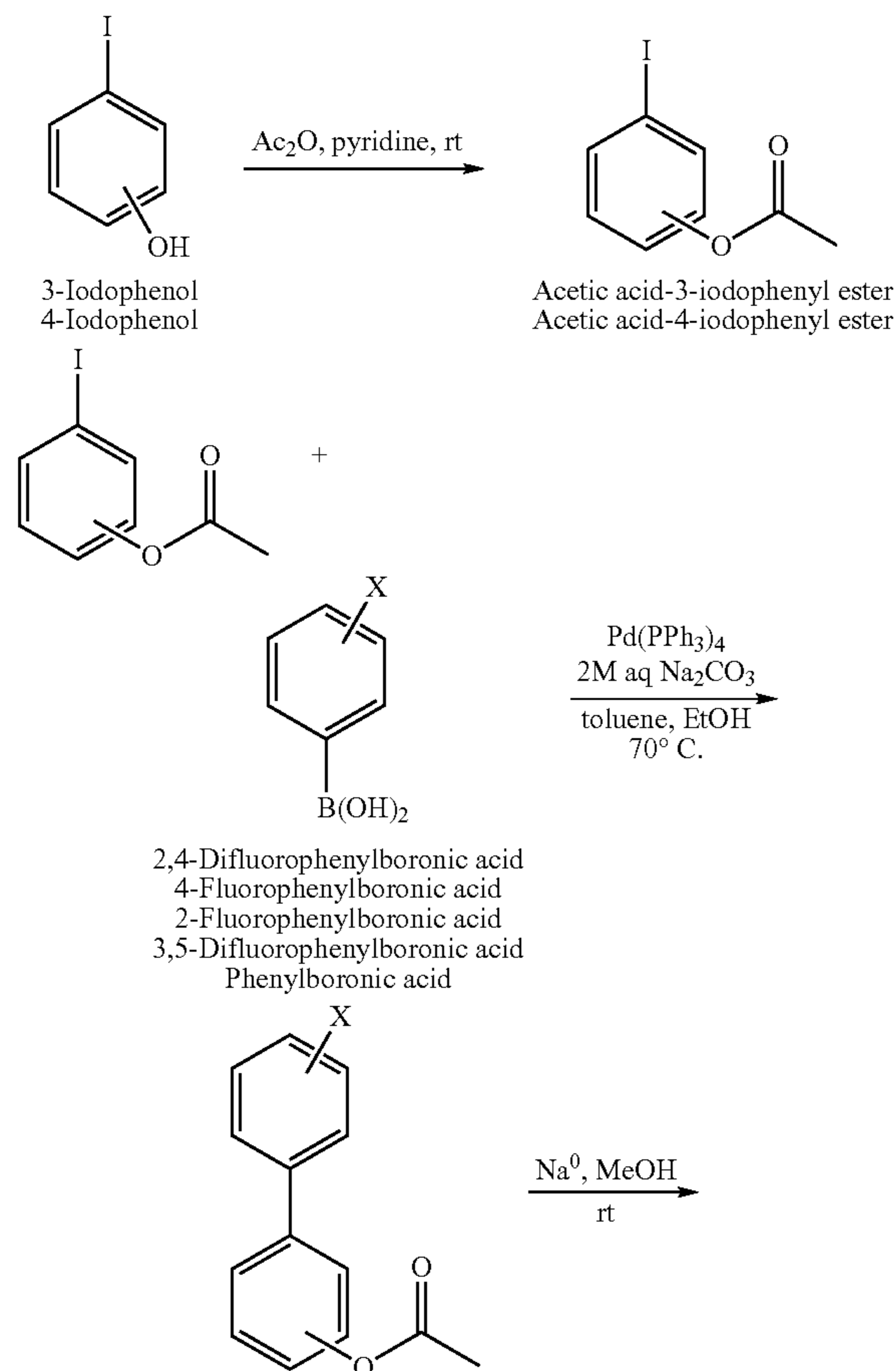
Scheme 1
