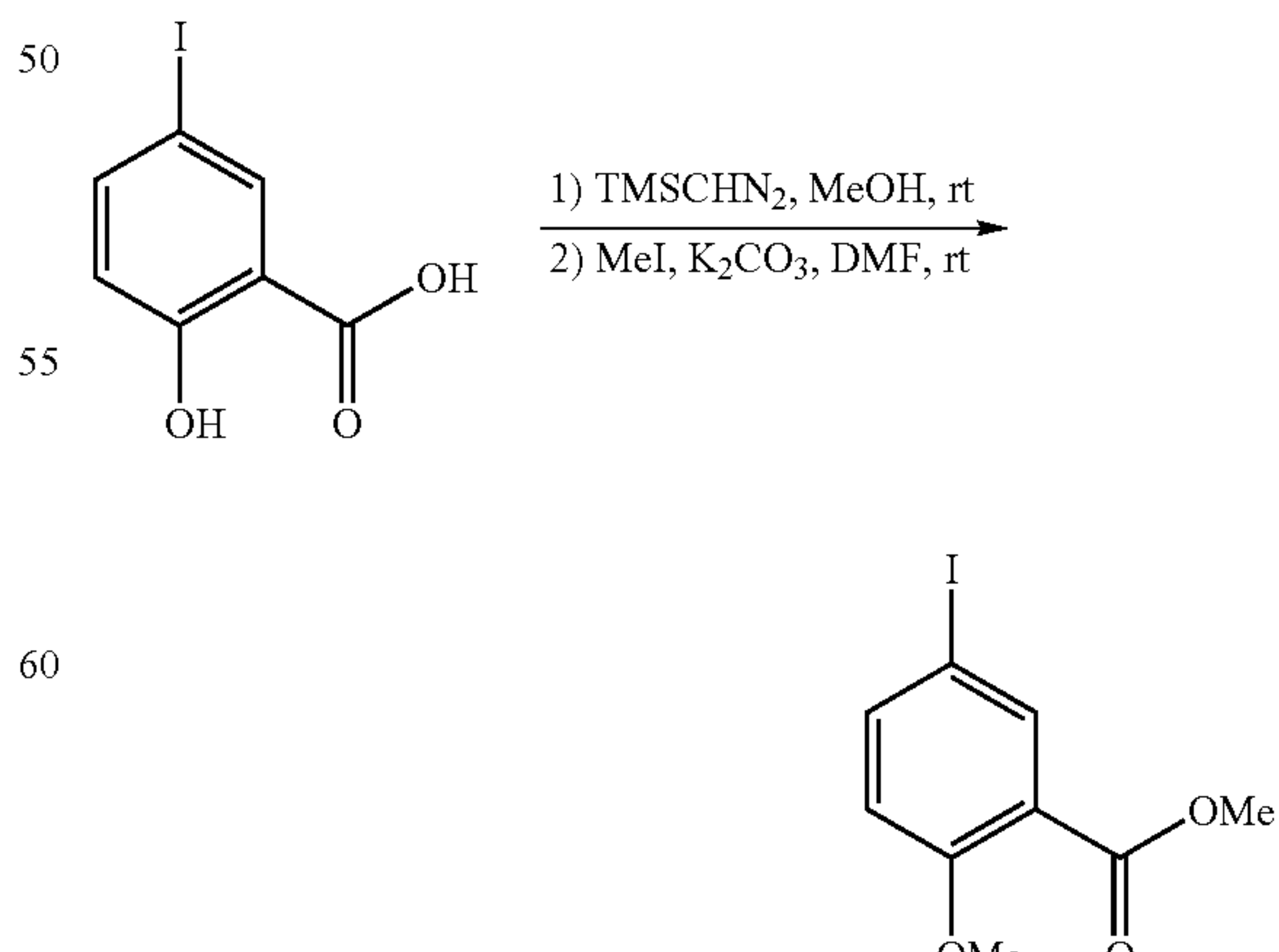
Methyl-5-iodo-2-methoxybenzoate
