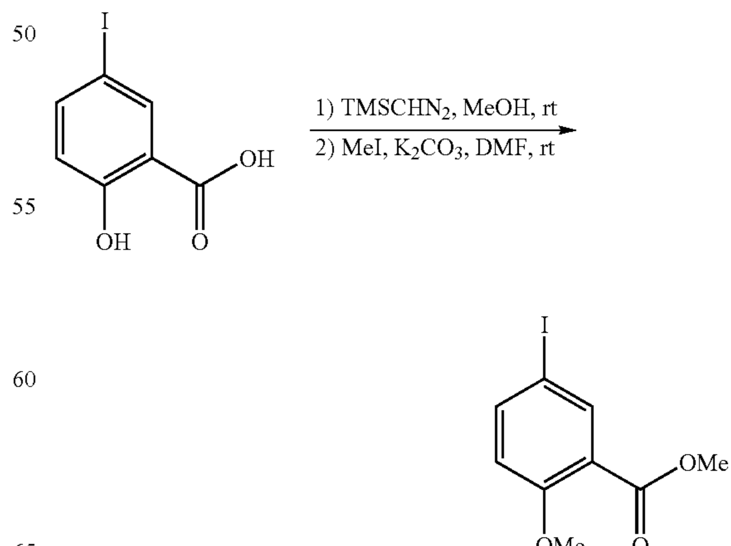
Methyl-5-iodo-2-methoxybenzoate
