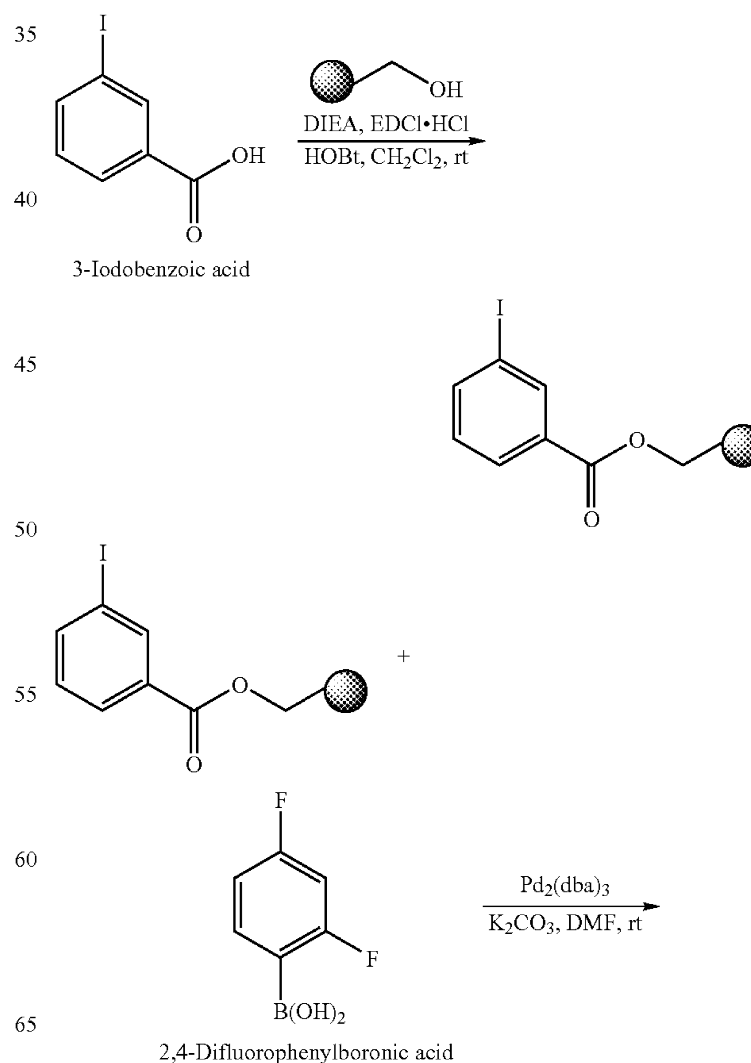
Scheme 2
