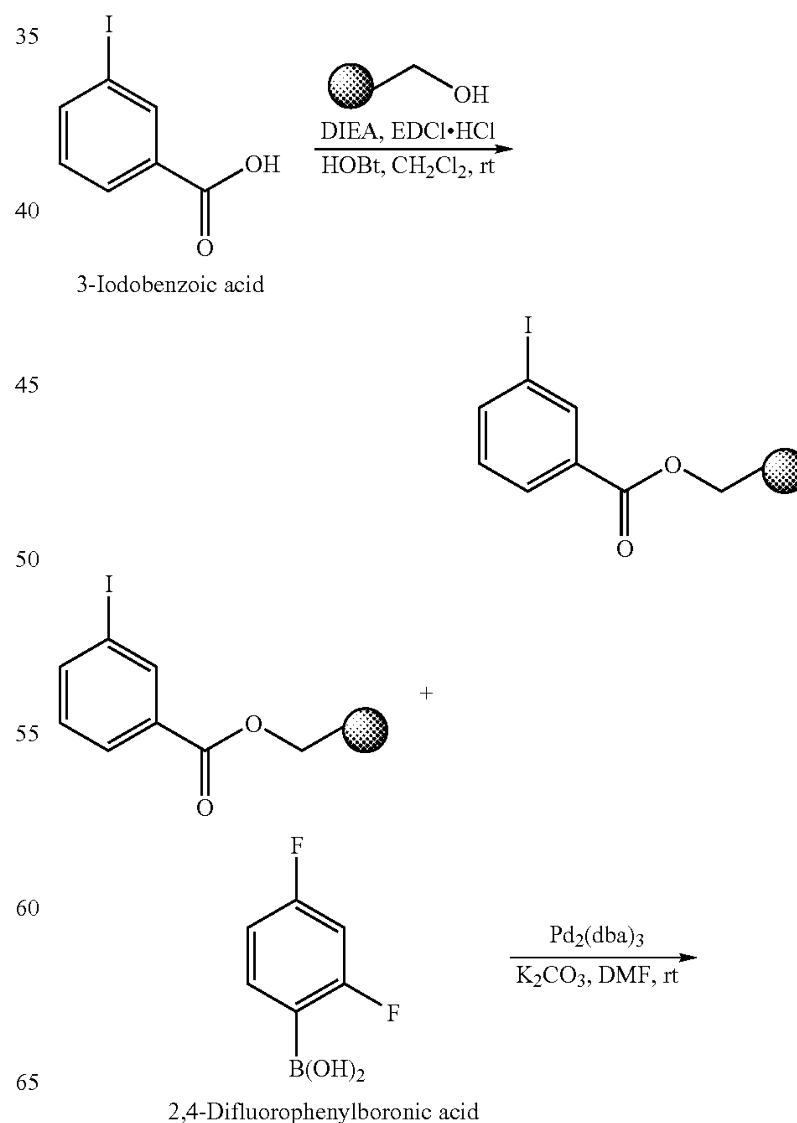
Scheme 2
