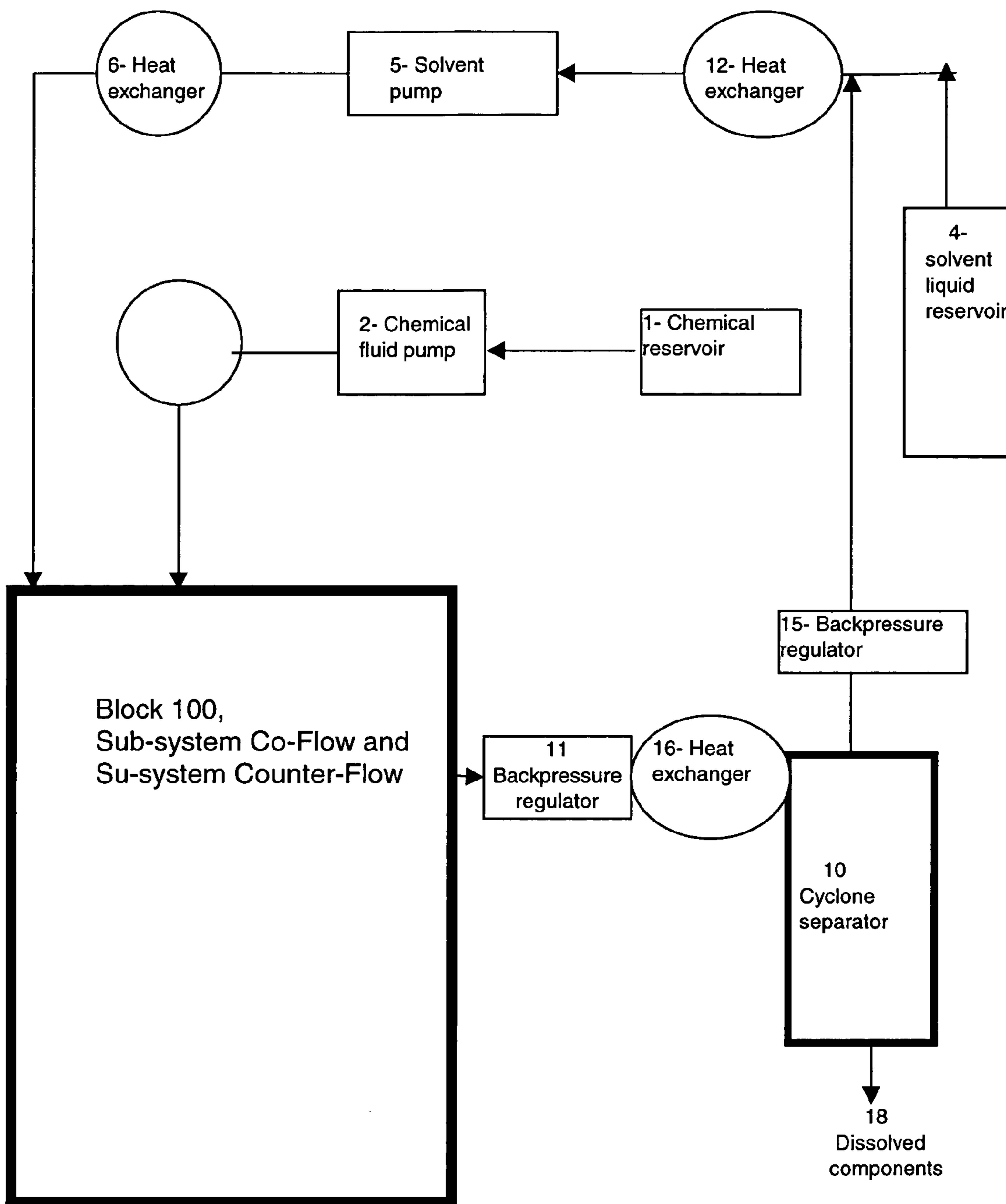
Figure 1 Overall Block Diagram Co-Flow and Counter-Flow Sub-systems
