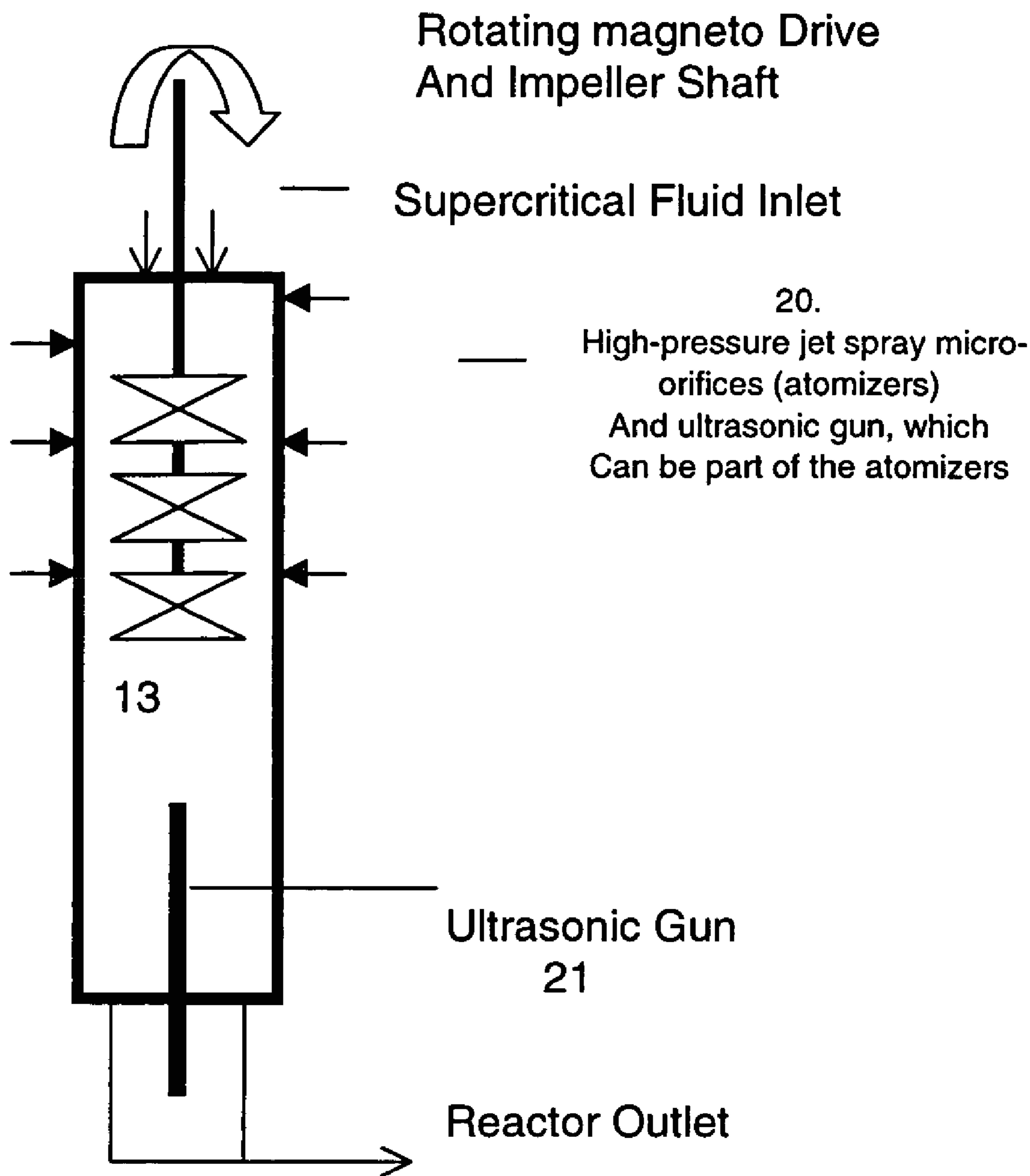
Figure 3, Co-Flow Reactor
