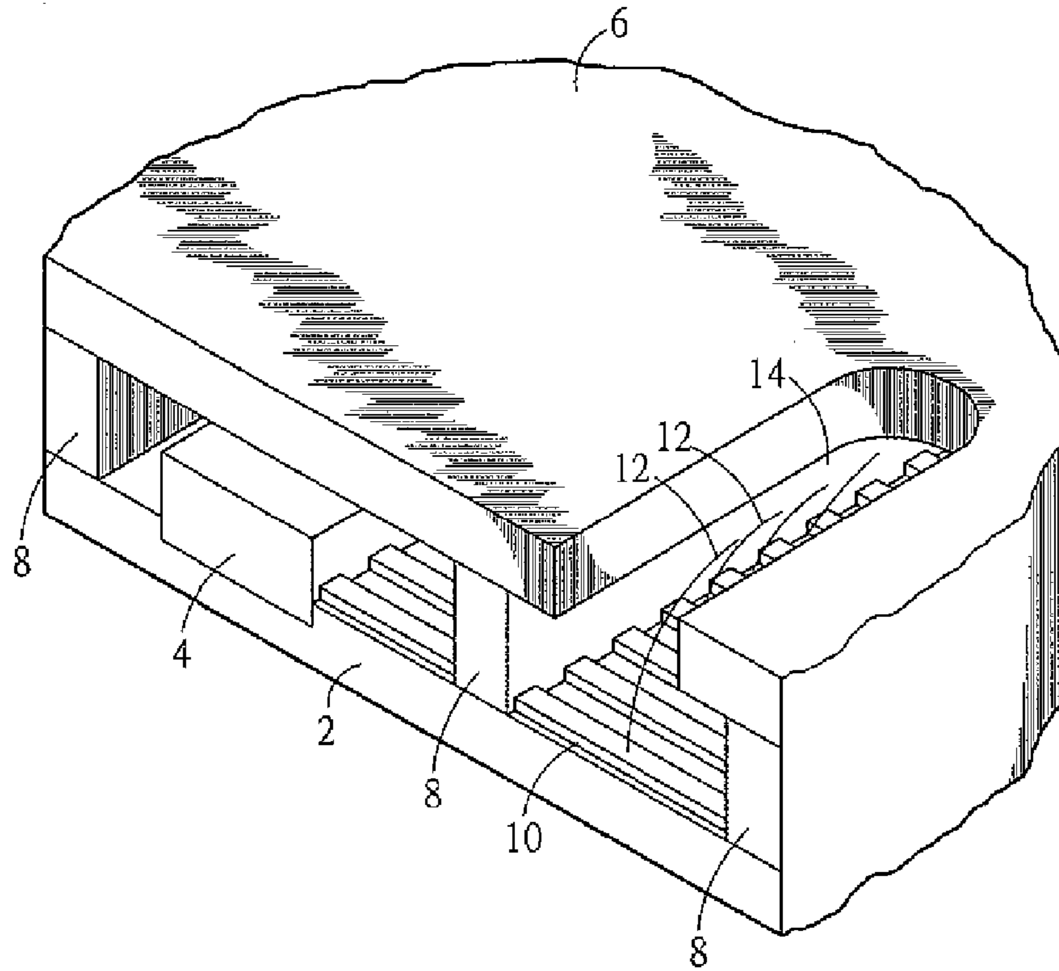
FIG. 1 (Prior Art)
