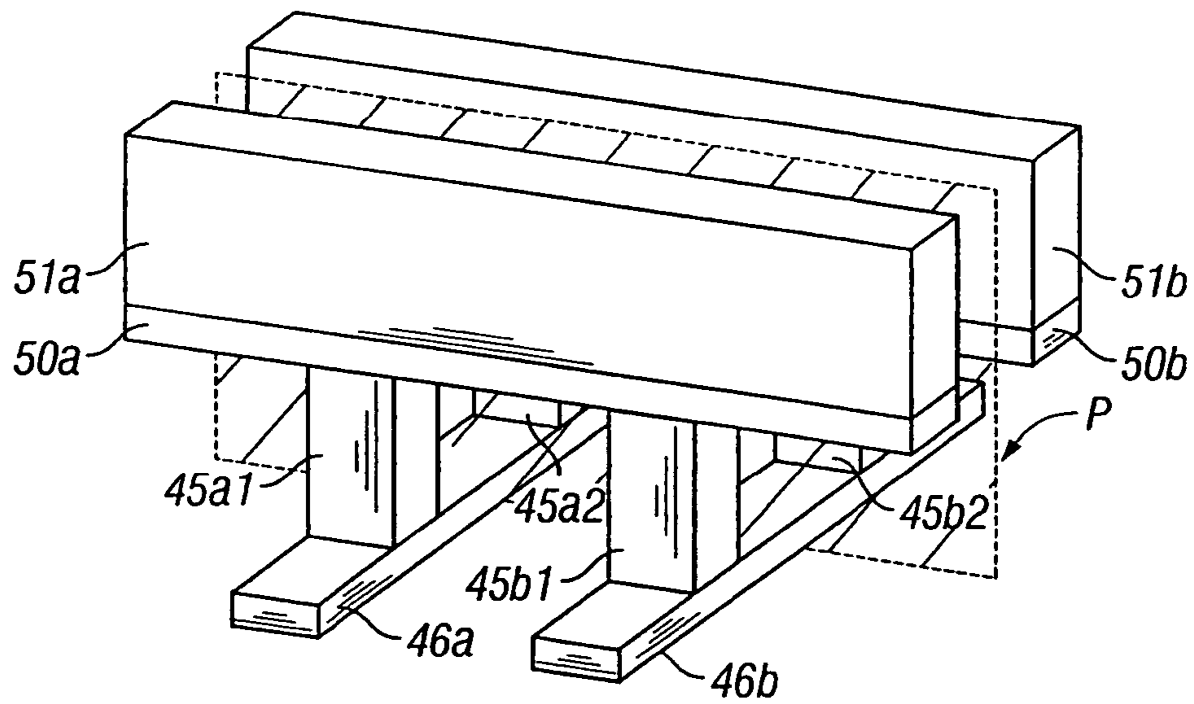
Prior Art
