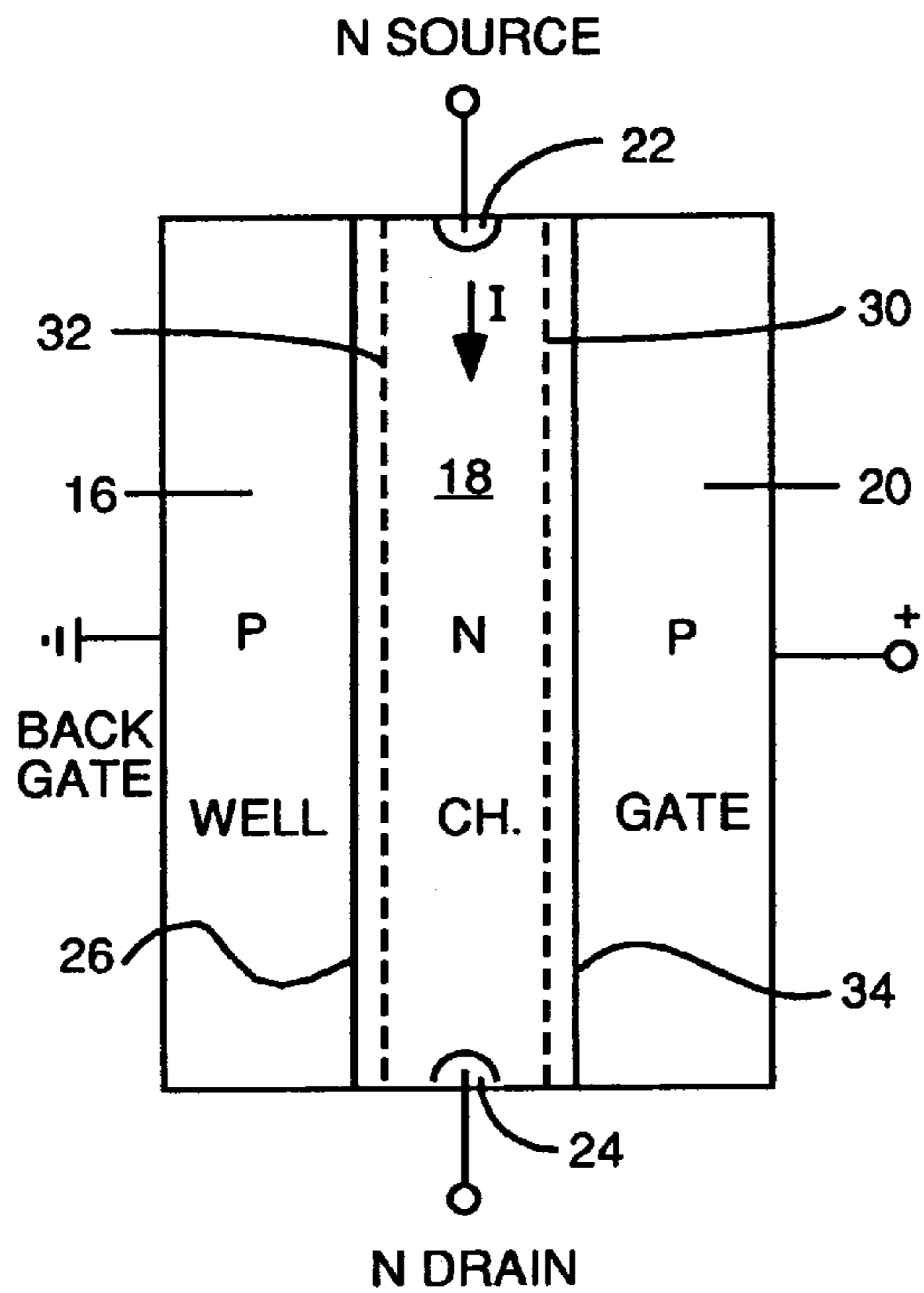
CONVENTIONAL JFET SCHEMATIC
