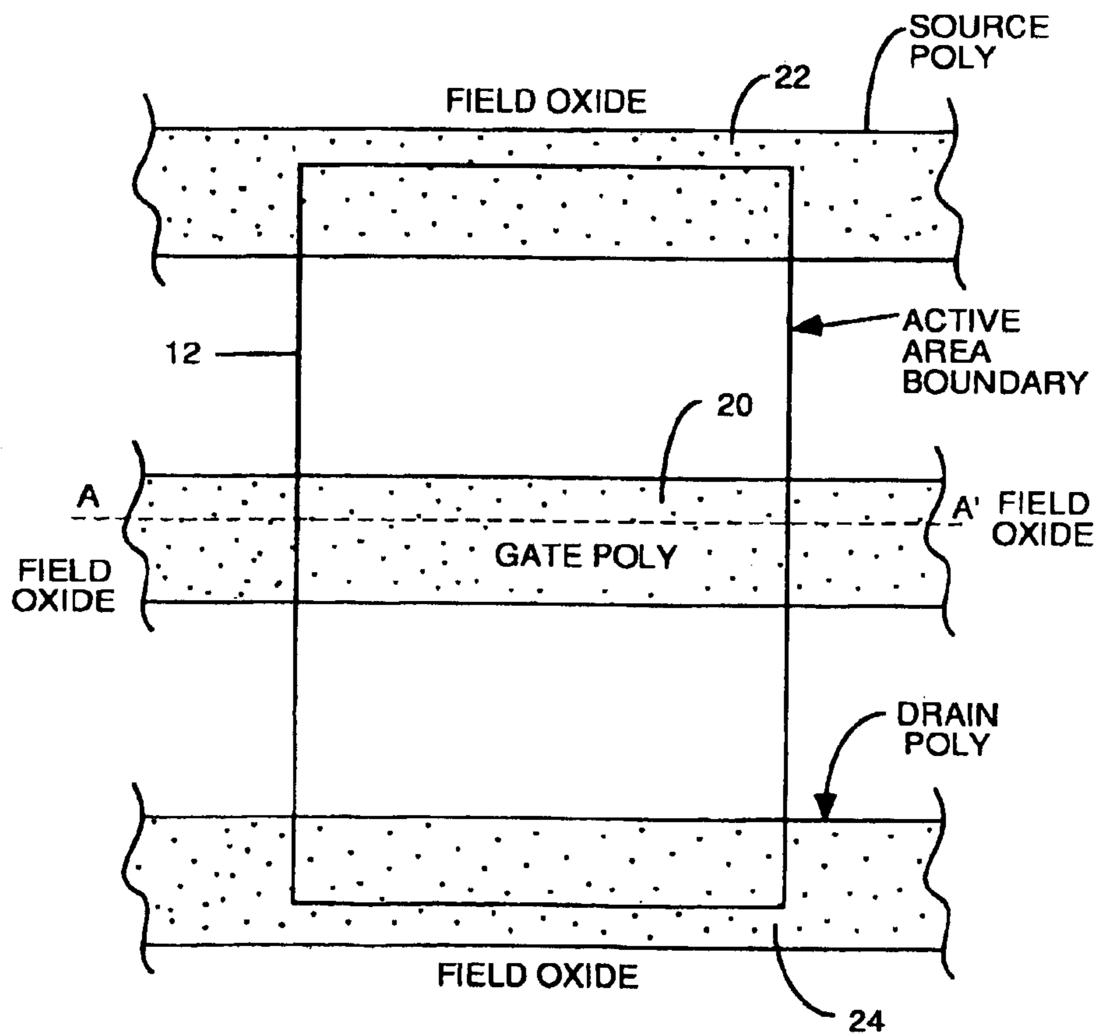
TOP VIEW
