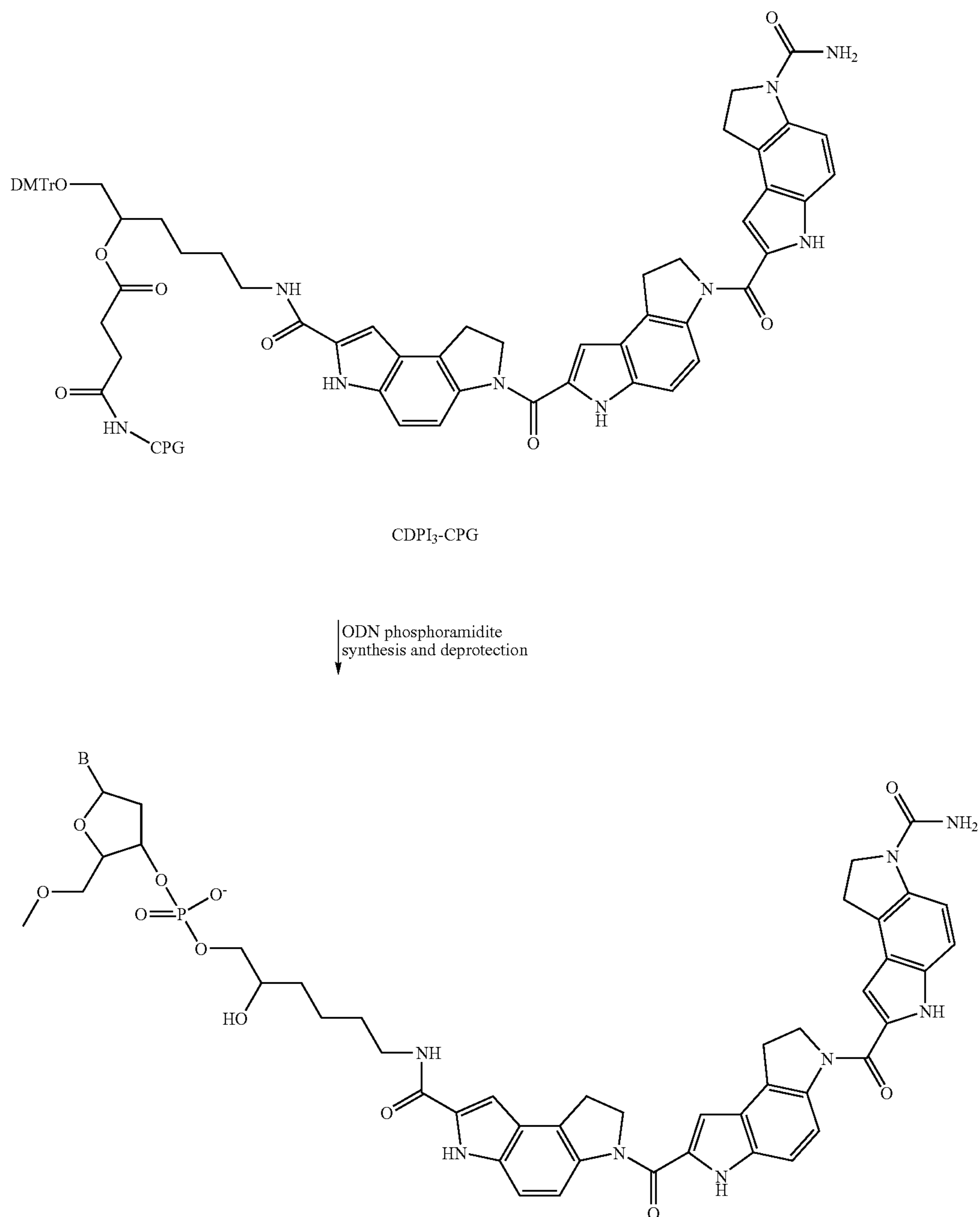
Scheme 7: Introduction of 3'-CDPI 3 residue using the CDPI 3 -CPG support (below)
