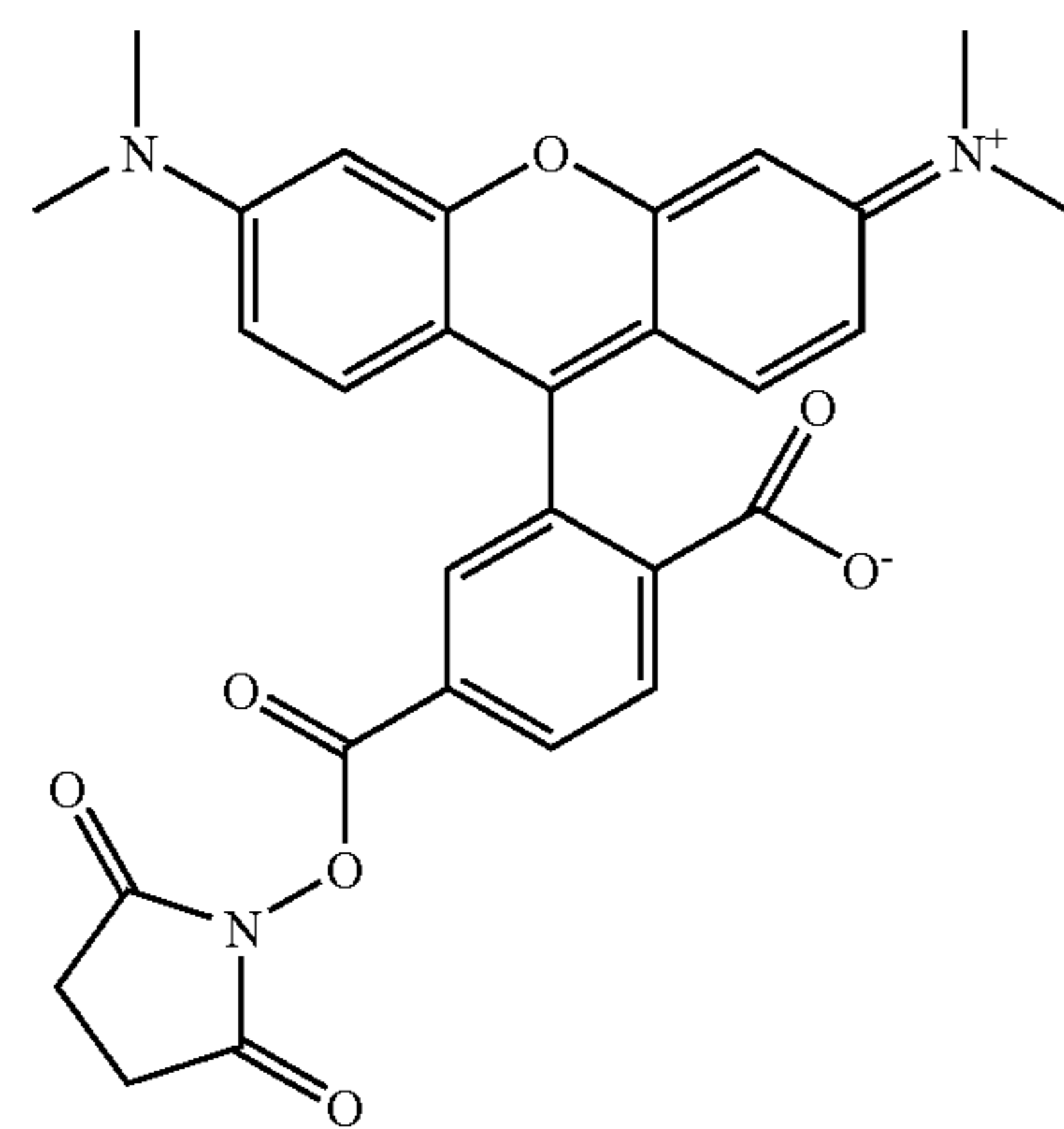
TAMRA NHS ester Glen Research
