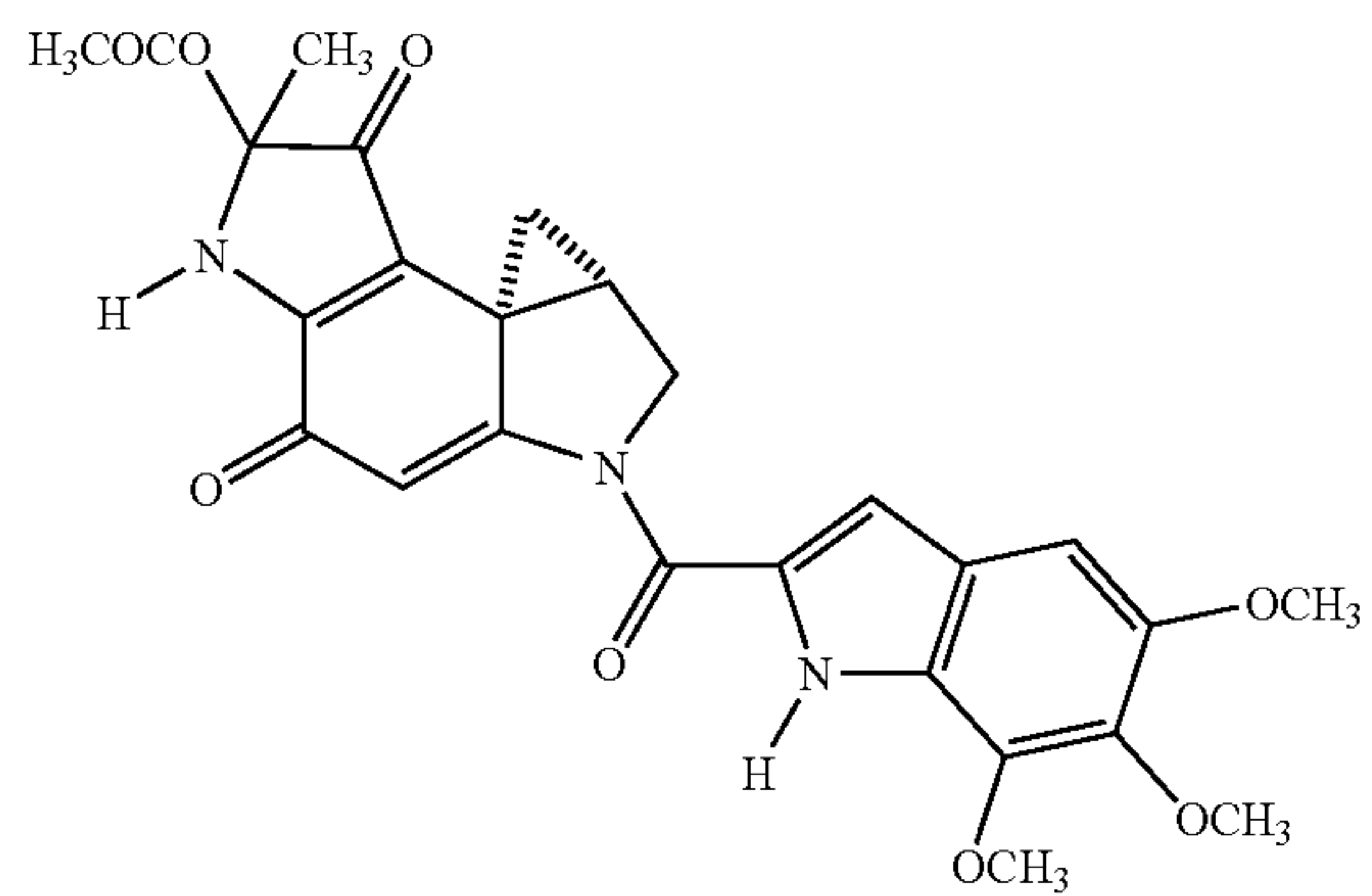
Duocarmycin A
