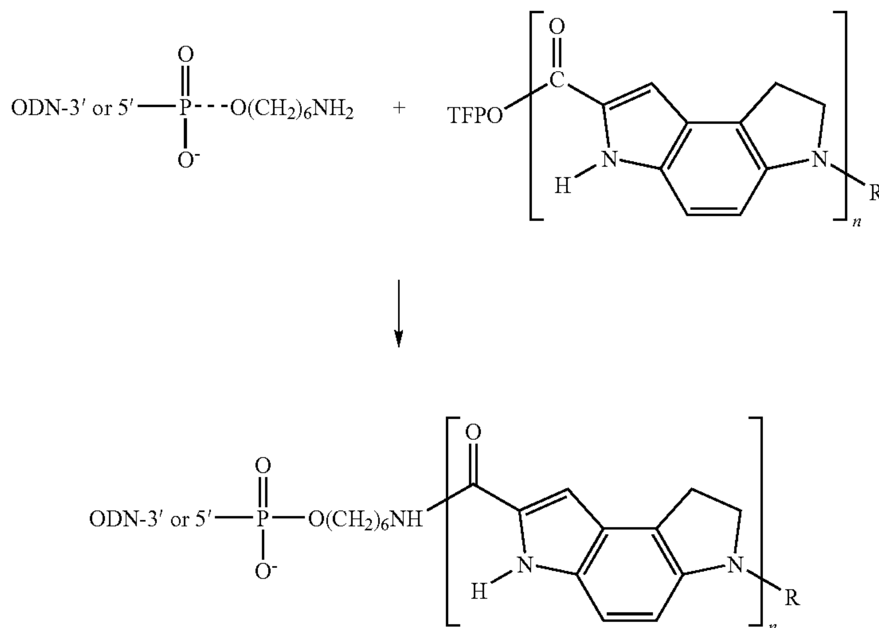
Reaction Scheme 3
