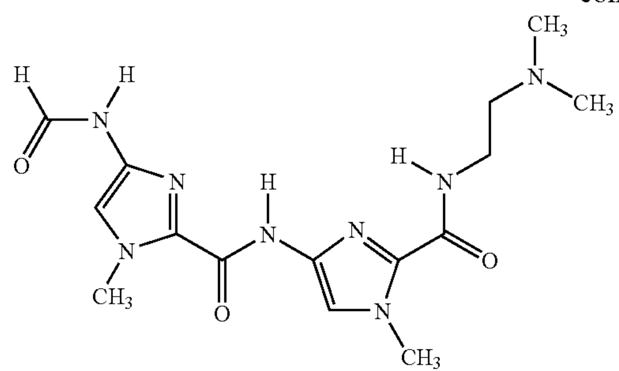
Lexitropsin
