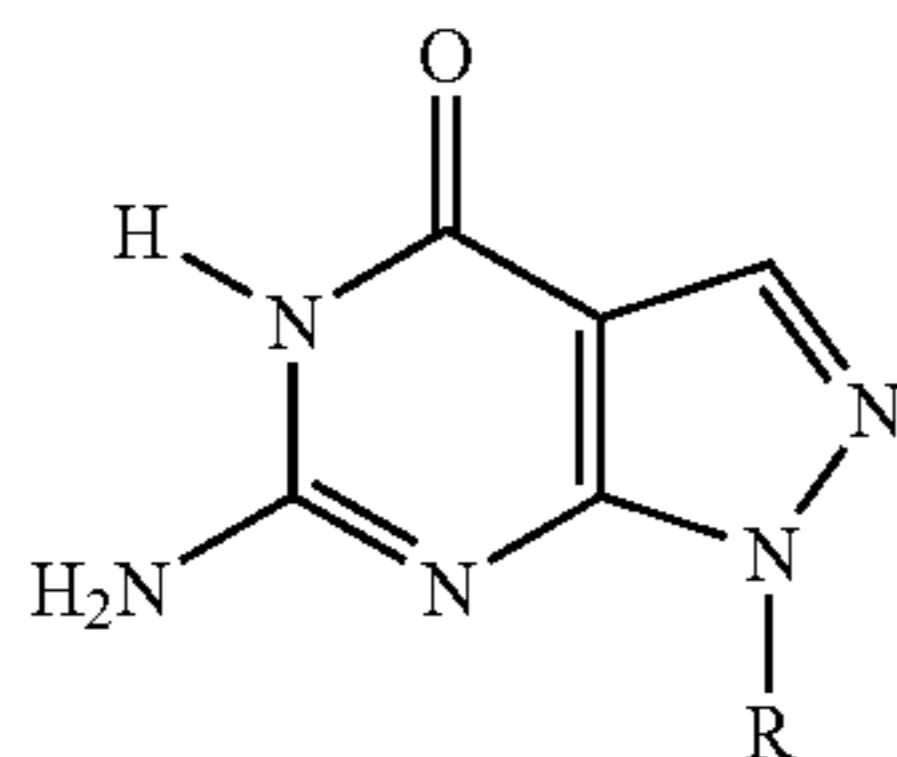
4-aminopyrazolo [3, 4-d] pyrimidine 2-deoxyribosides
