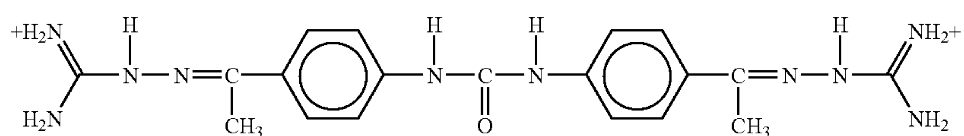
DDUG
