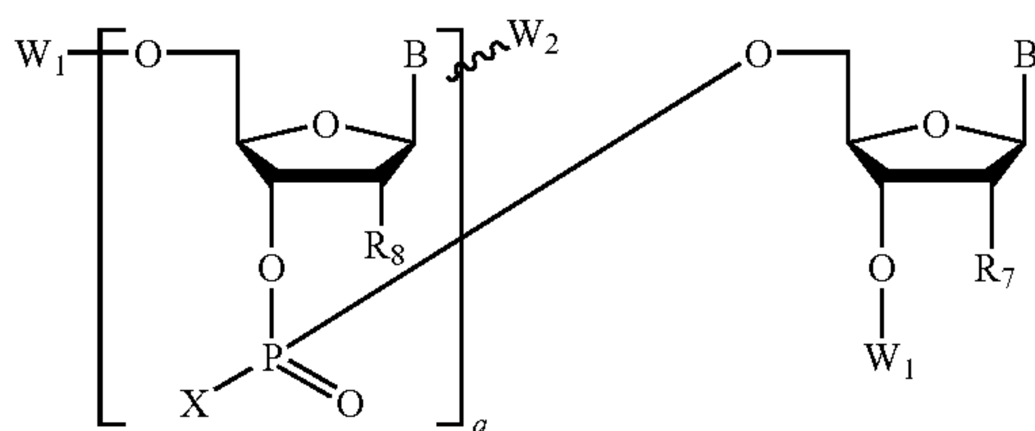
Formula 1
