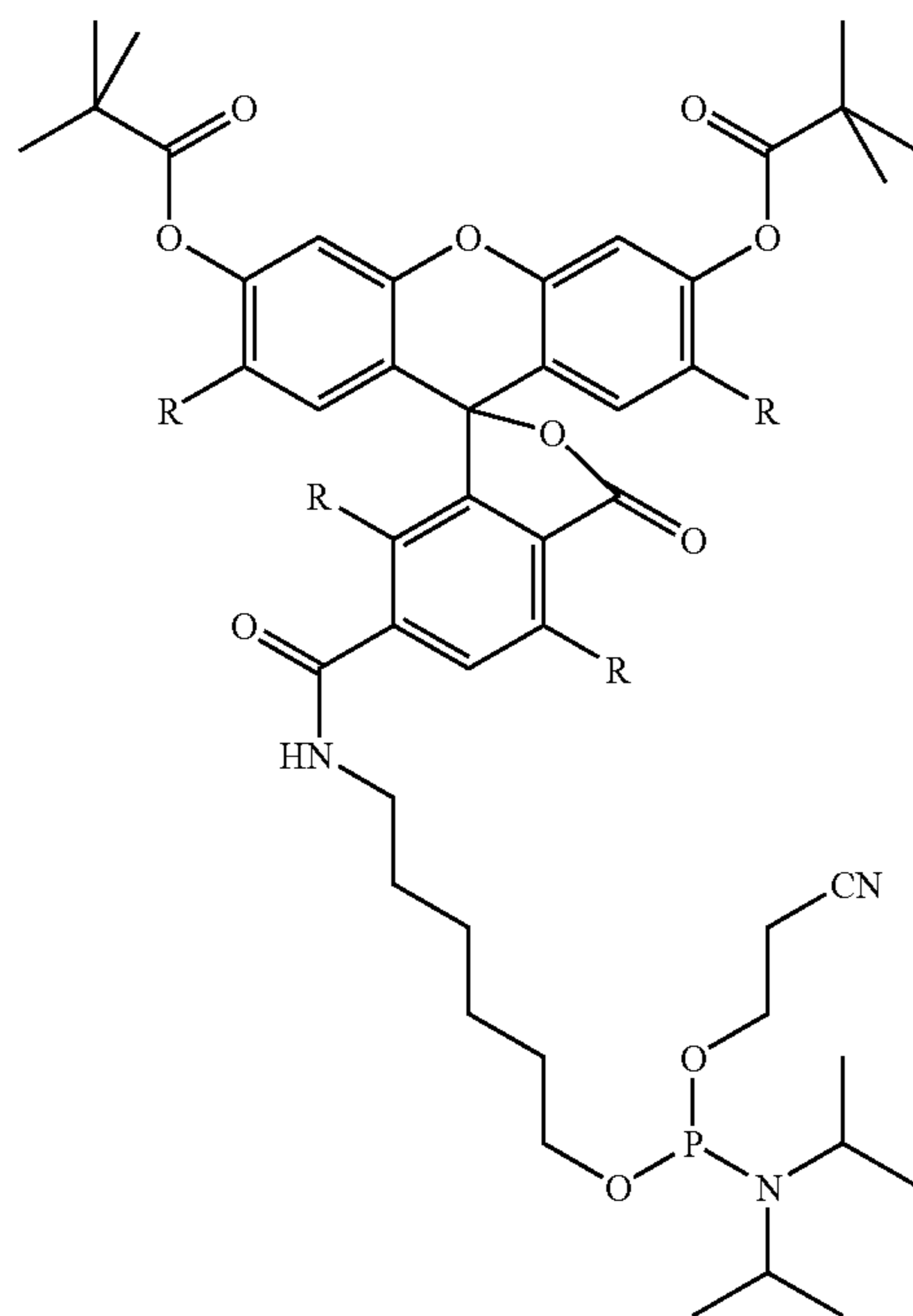
Scheme 8: Introduction of fluorophores at the 5[40 -end using 6-FAM and TET phosphoramidates (below)
