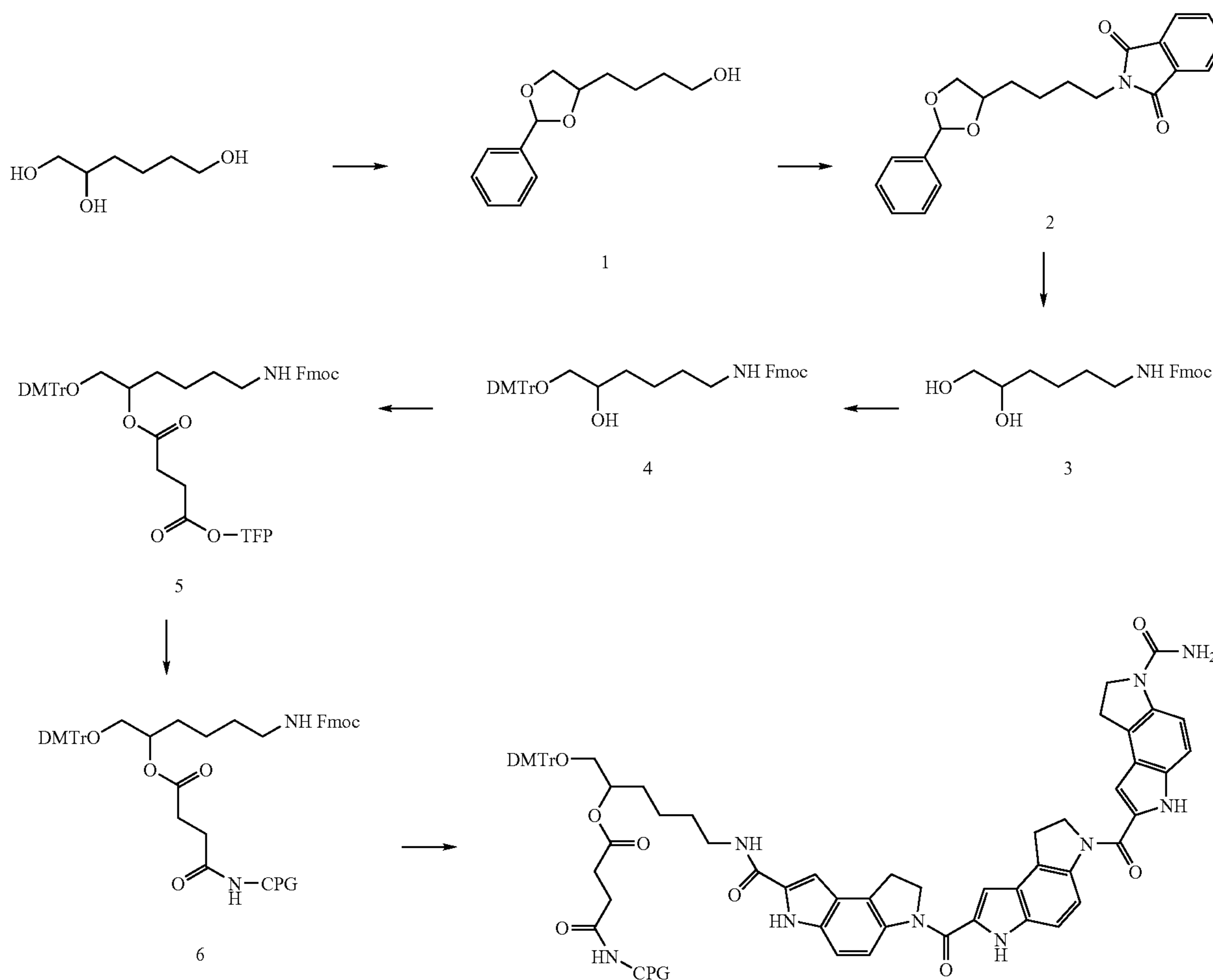
Scheme 6: Preparation of CDPI 3 -CPG support (below)
