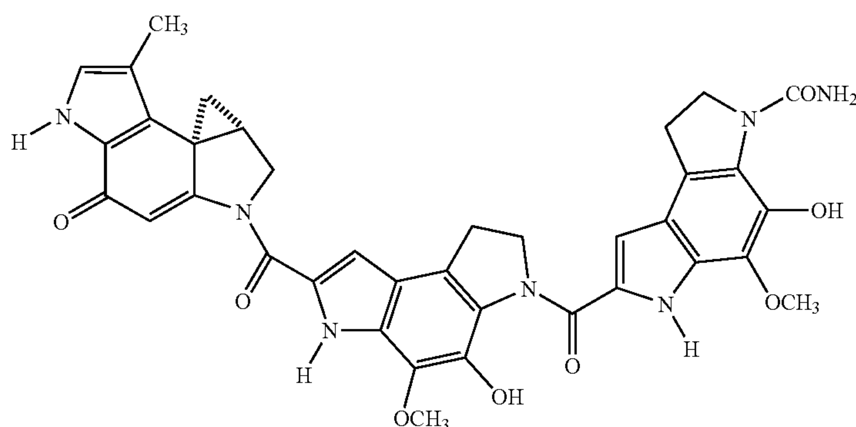
CC-1065
