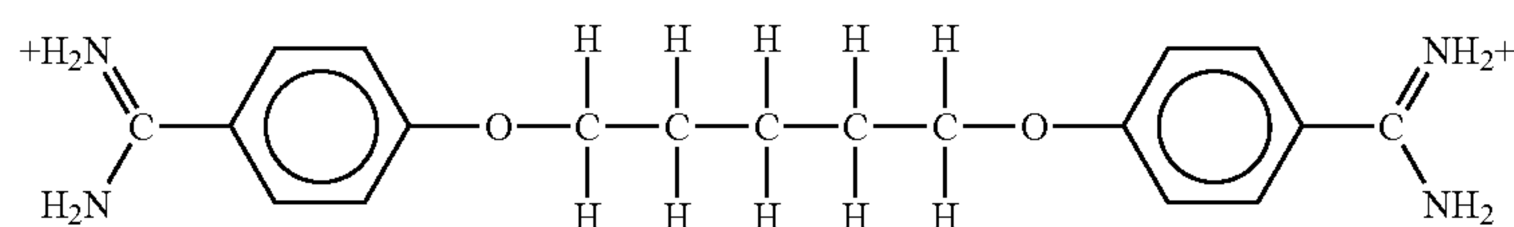
Pentamidine
