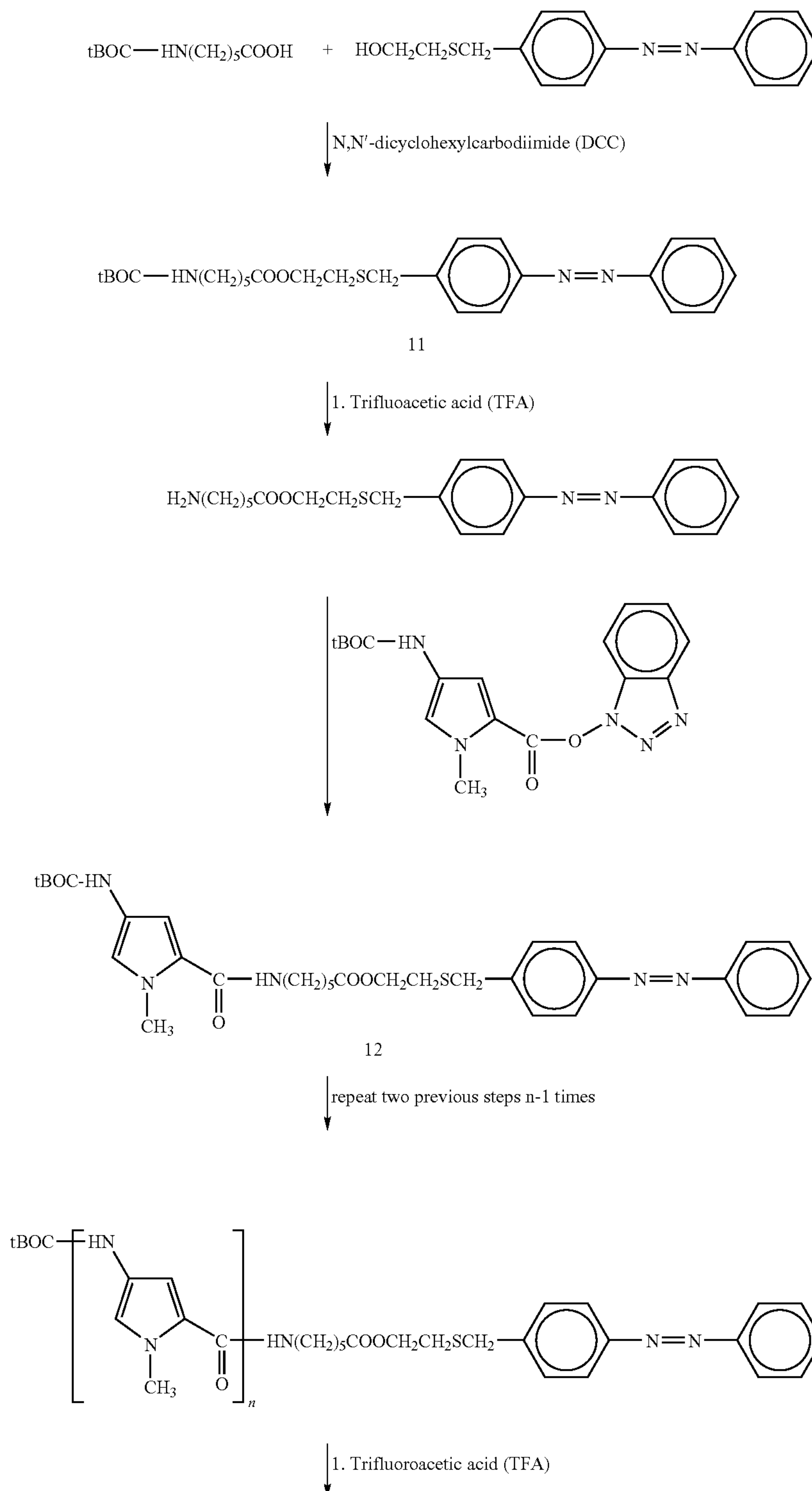
Reaction Scheme 2
