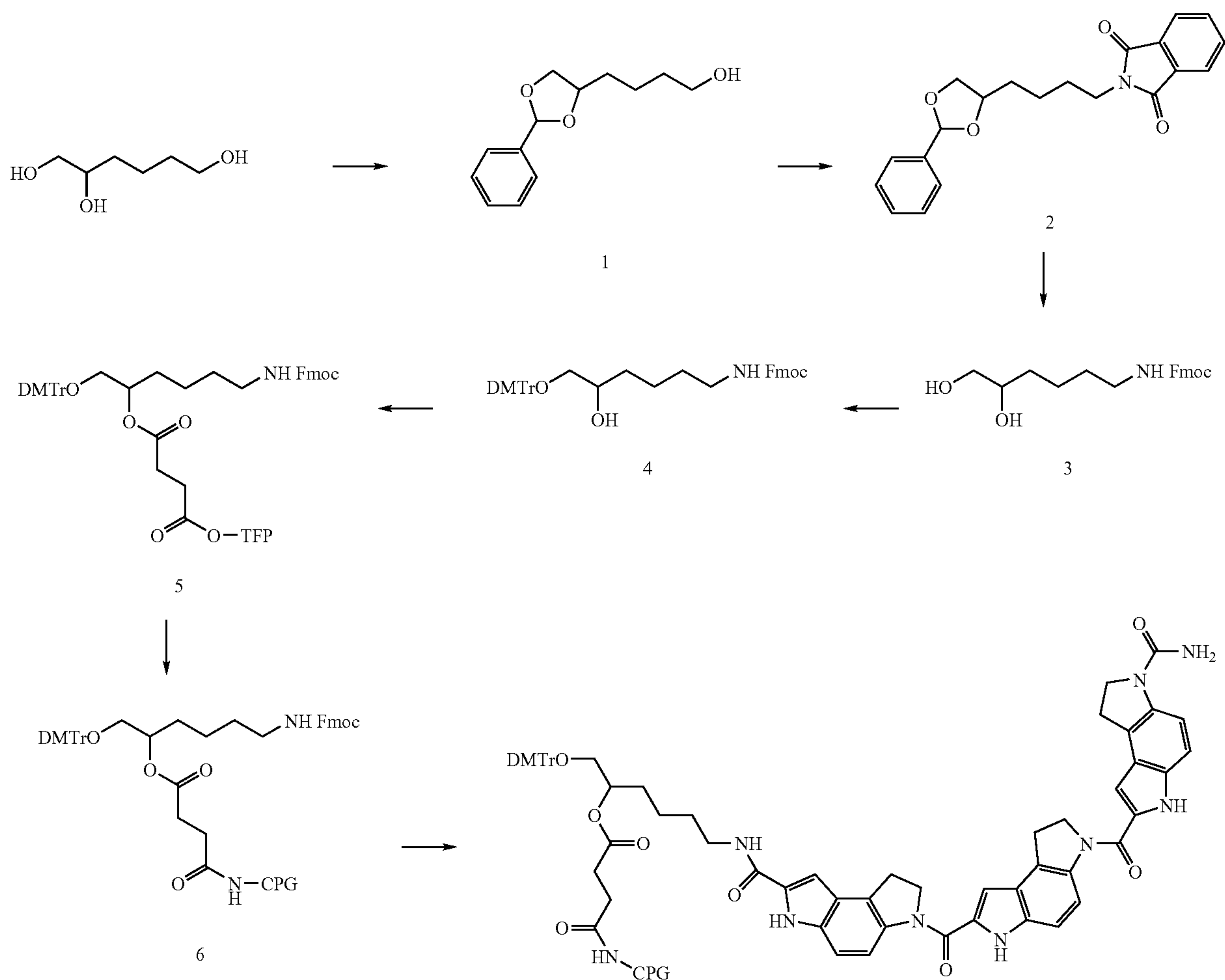
Scheme 6: Preparation of CDPI 3 -CPG support (below)
