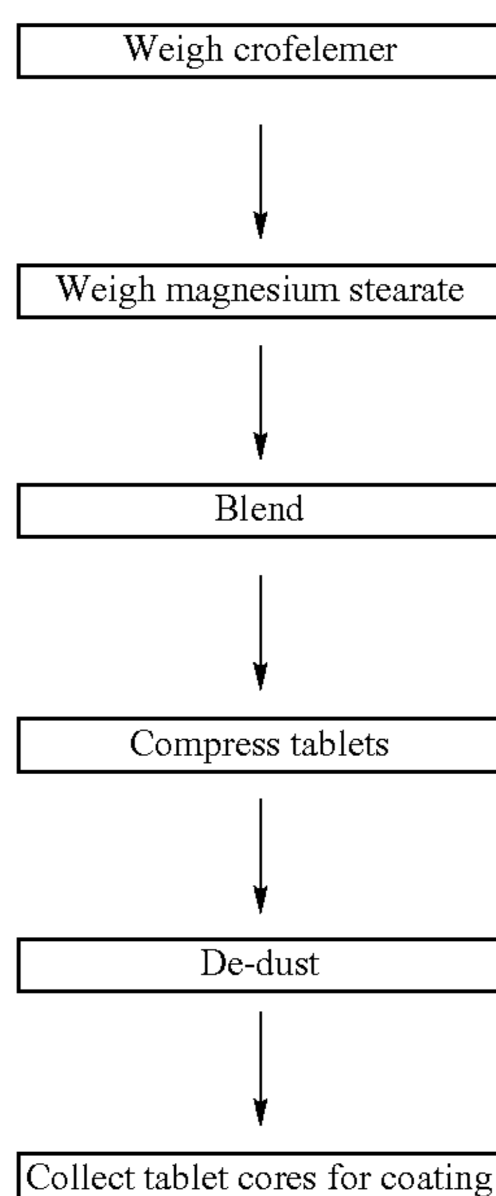
Schematic of Tablet Core Manufacturing Process
