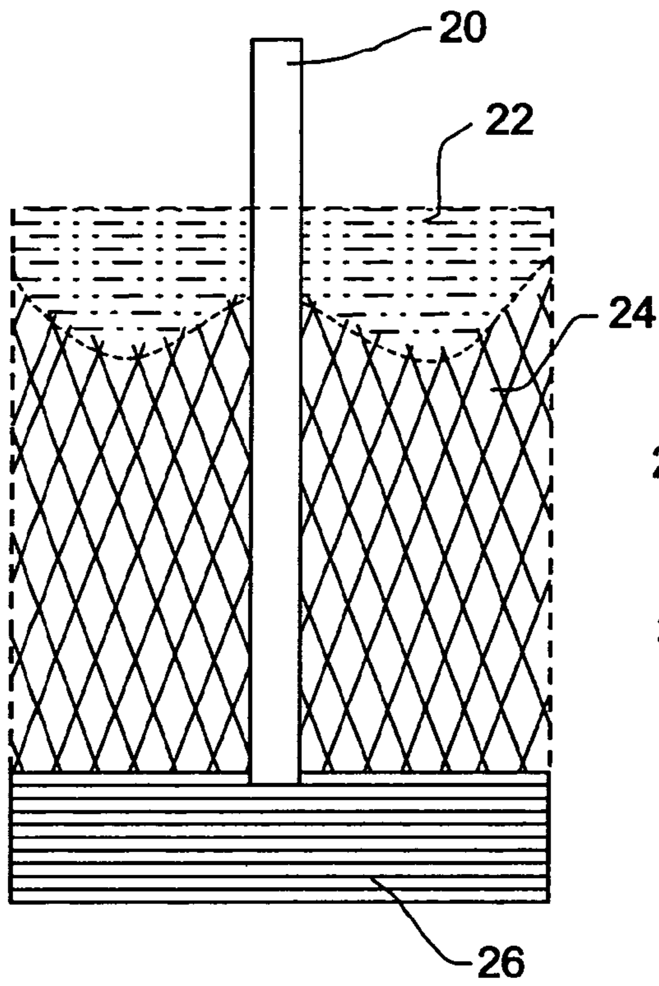
FIG. 10 Prior Art
