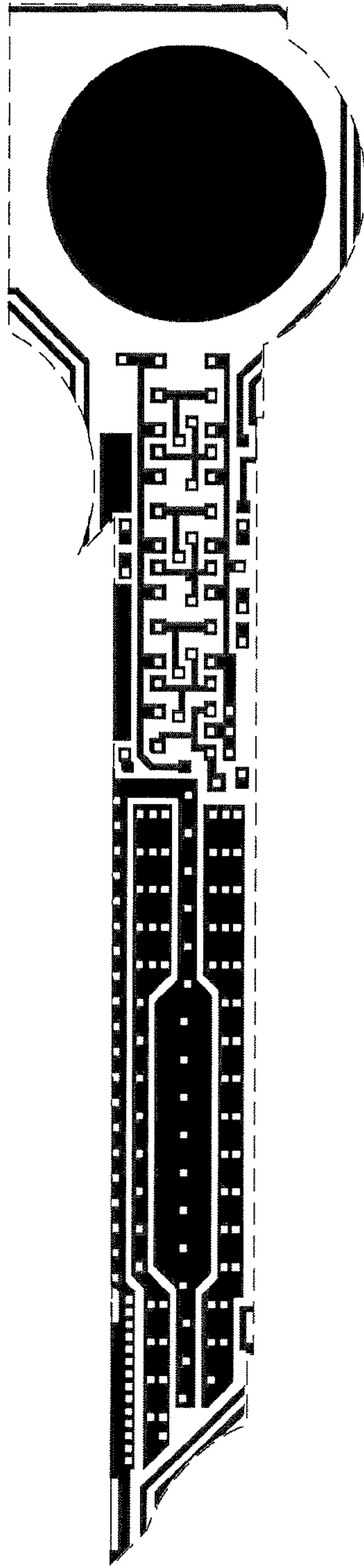
Metal 1 mask
