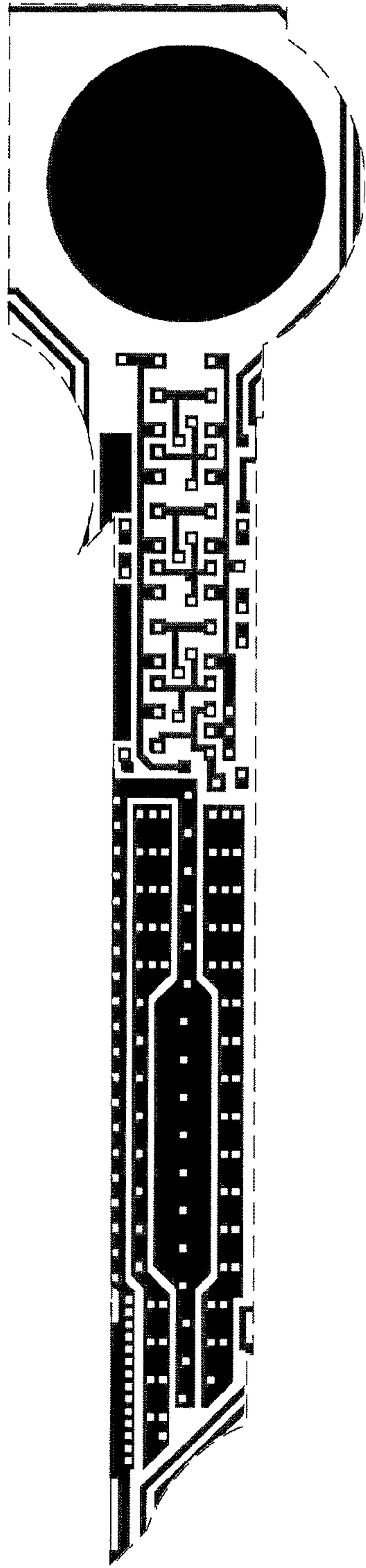
Metal 1 mask
