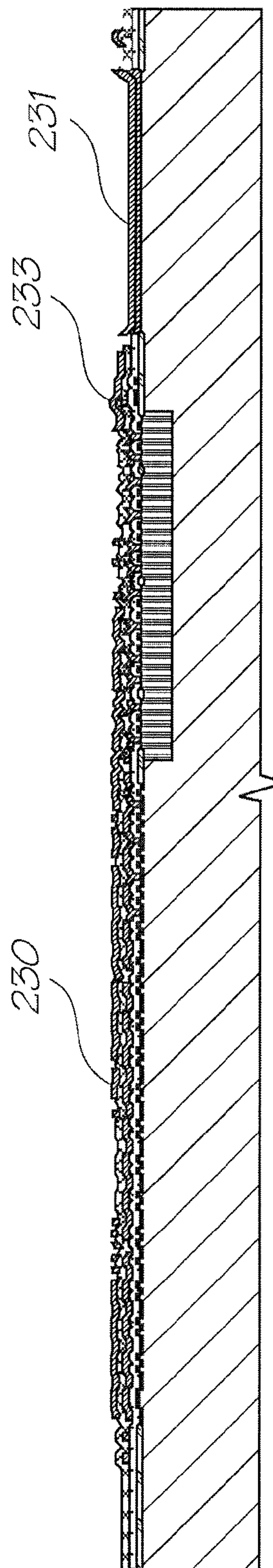
Deposit metal 2
