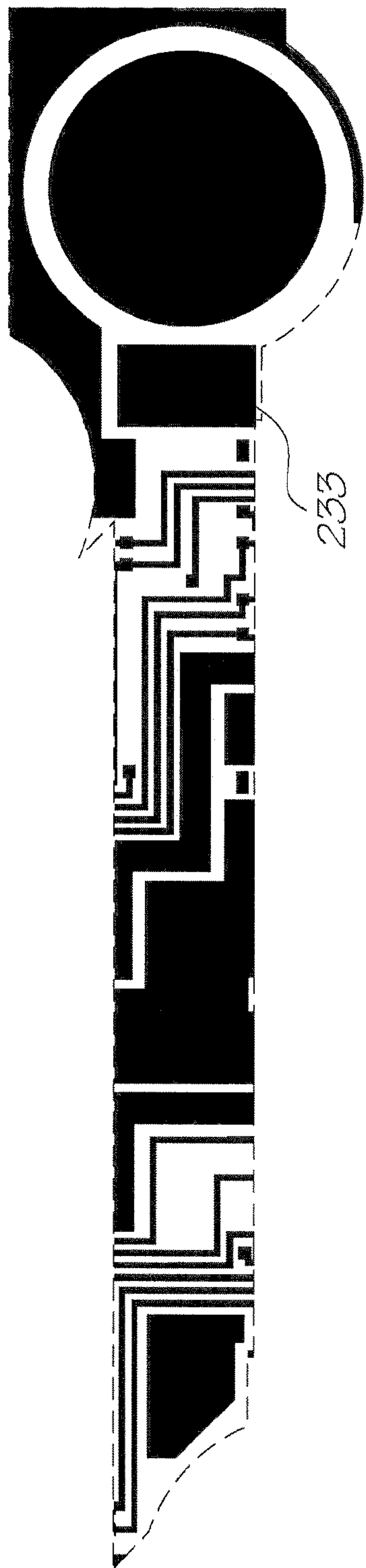
Metal 2 mask
