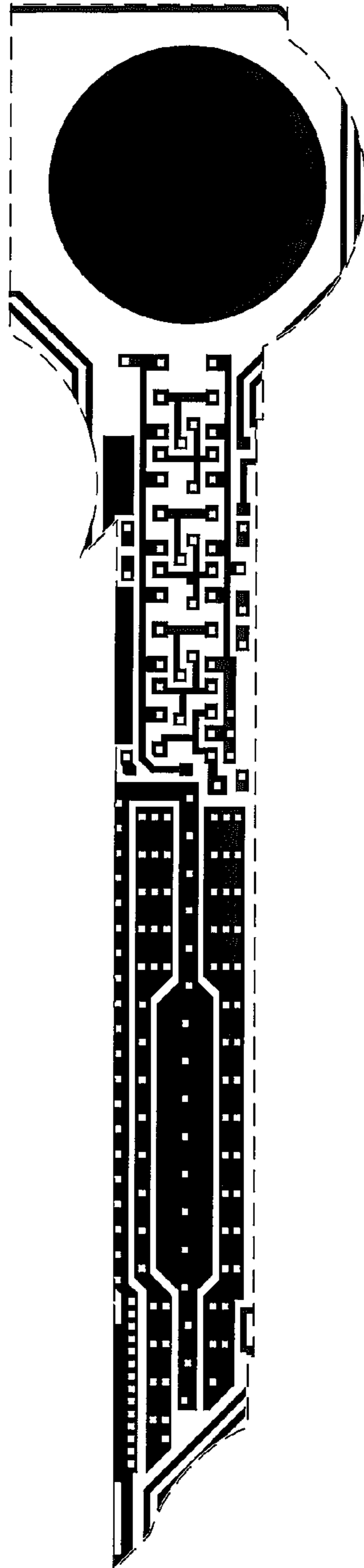
Metal 1 mask
