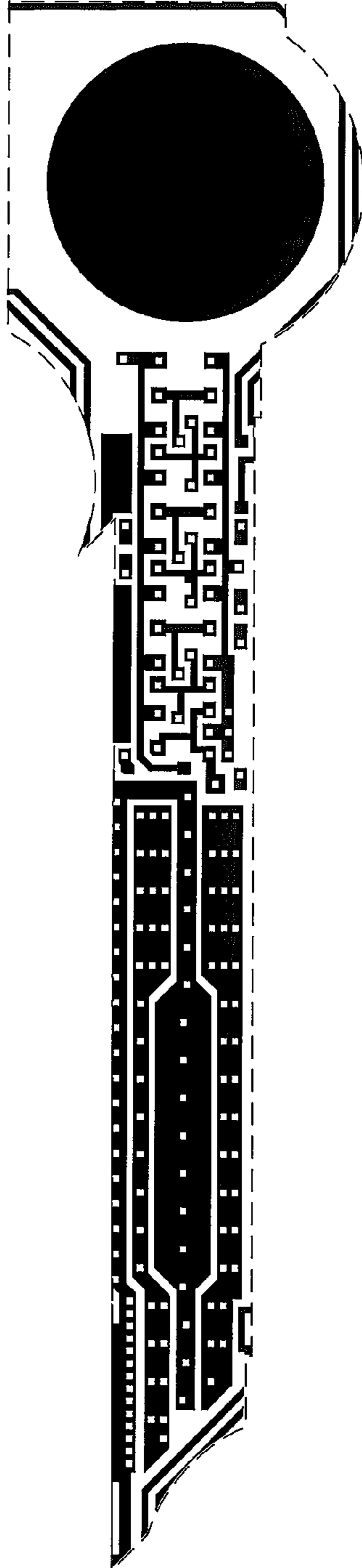
Metal 1 mask
