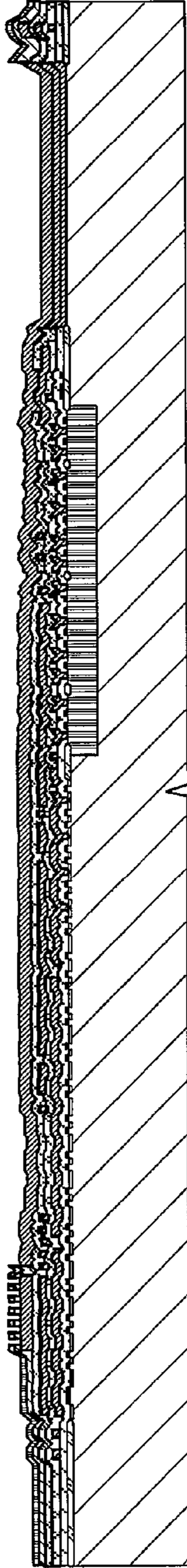
Deposit passivation oxide & nitride, etch vias
