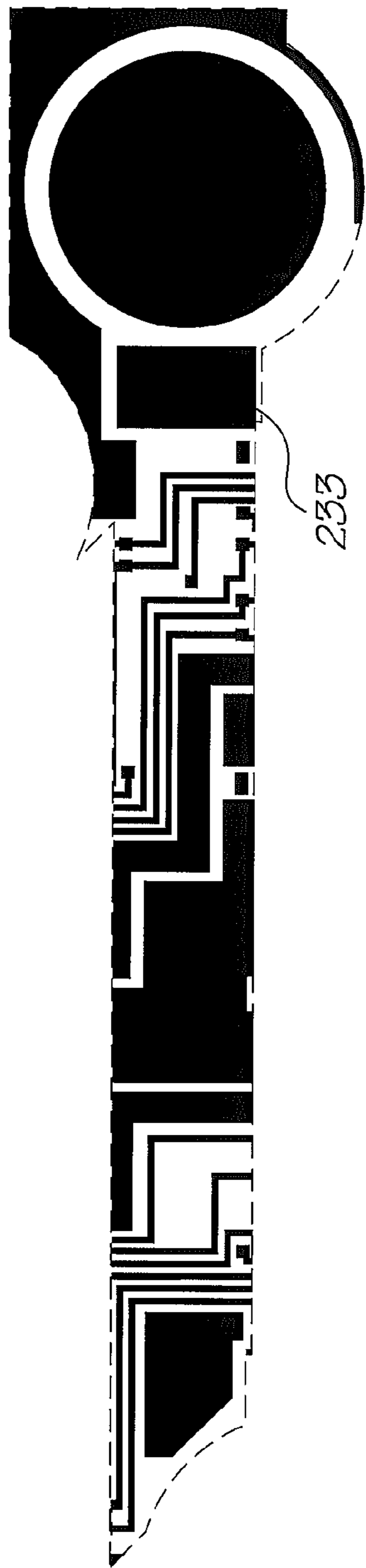
Metal 2 mask
