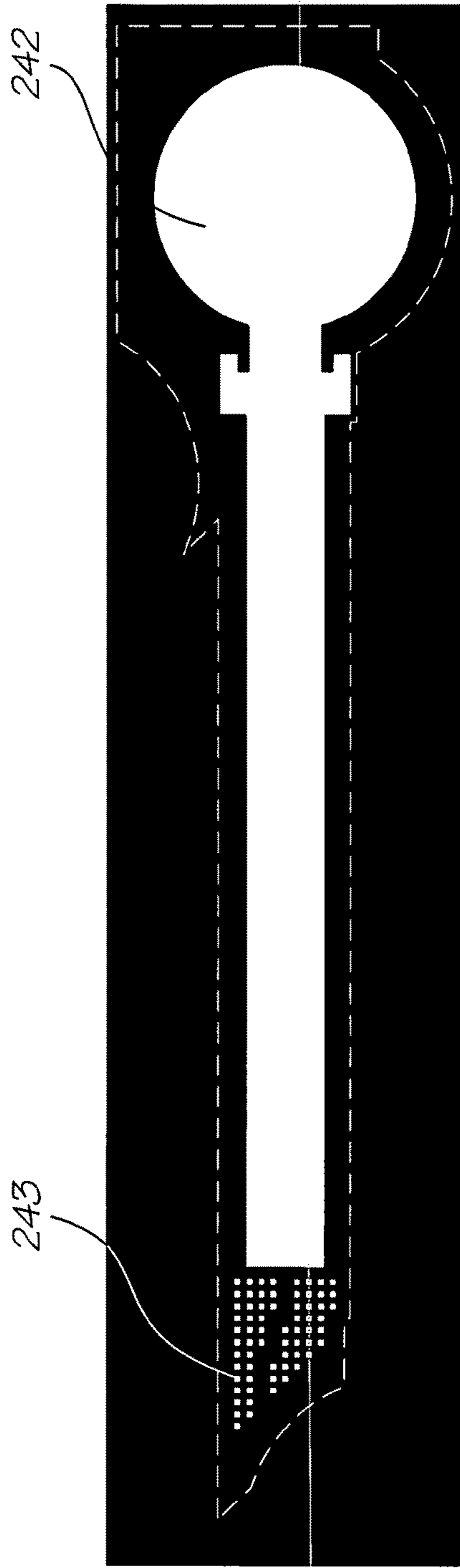
Via 3 / Passivation mask
