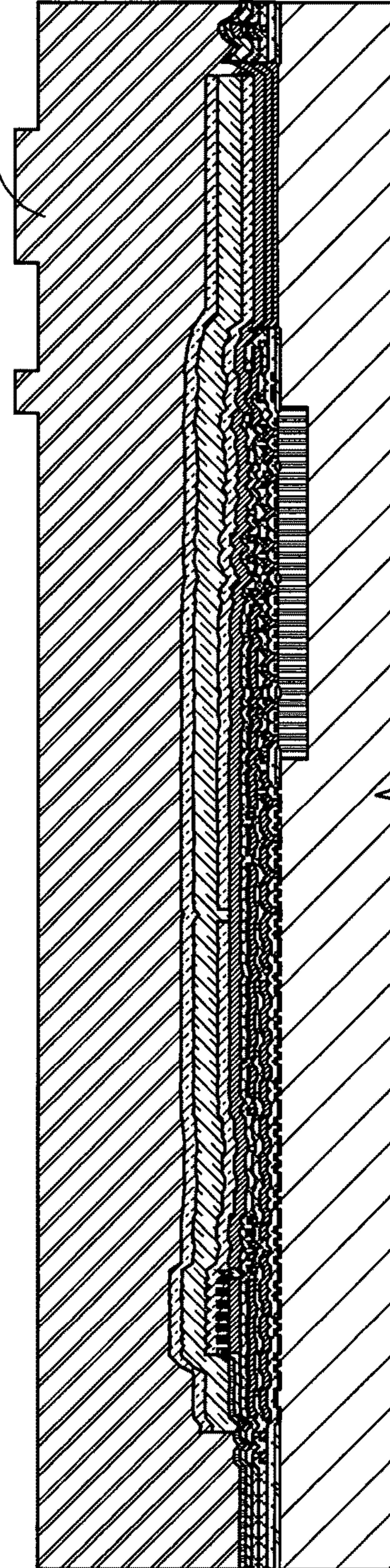
Deposit sacrificial layer, etch nozzles
