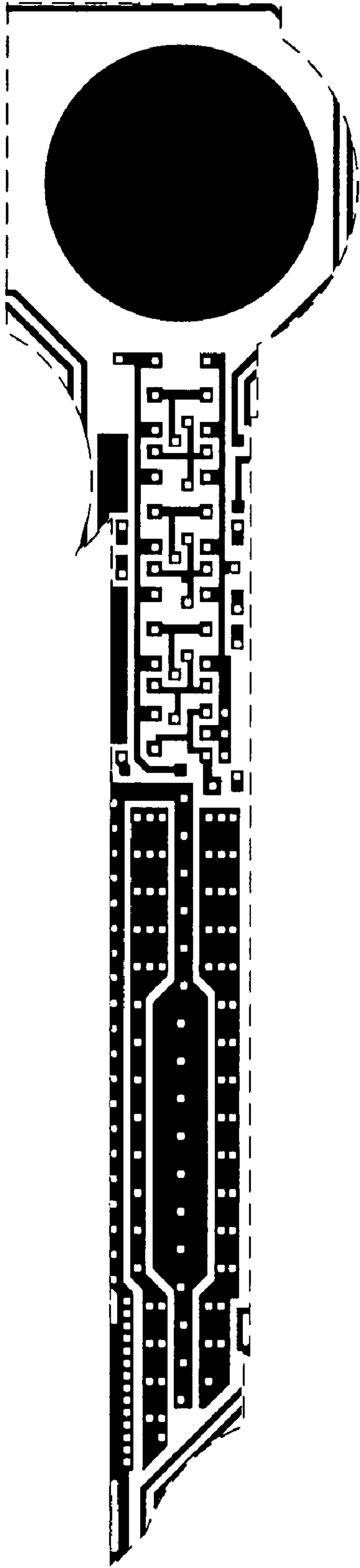
Metal 1 mask
