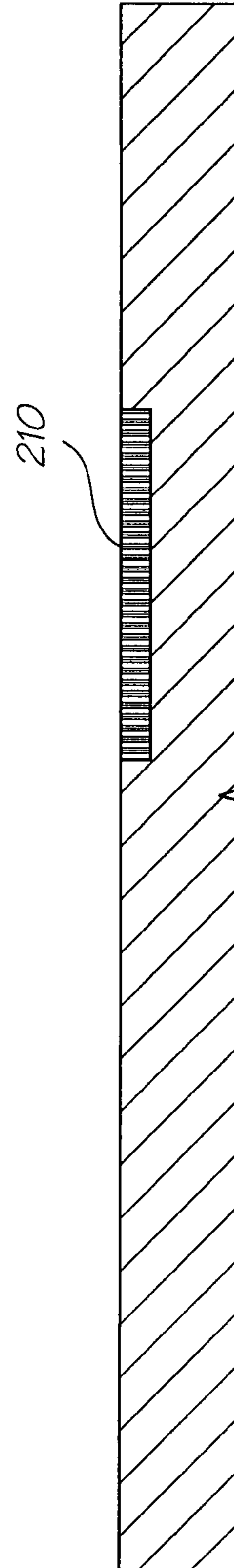
Implant N-Well
