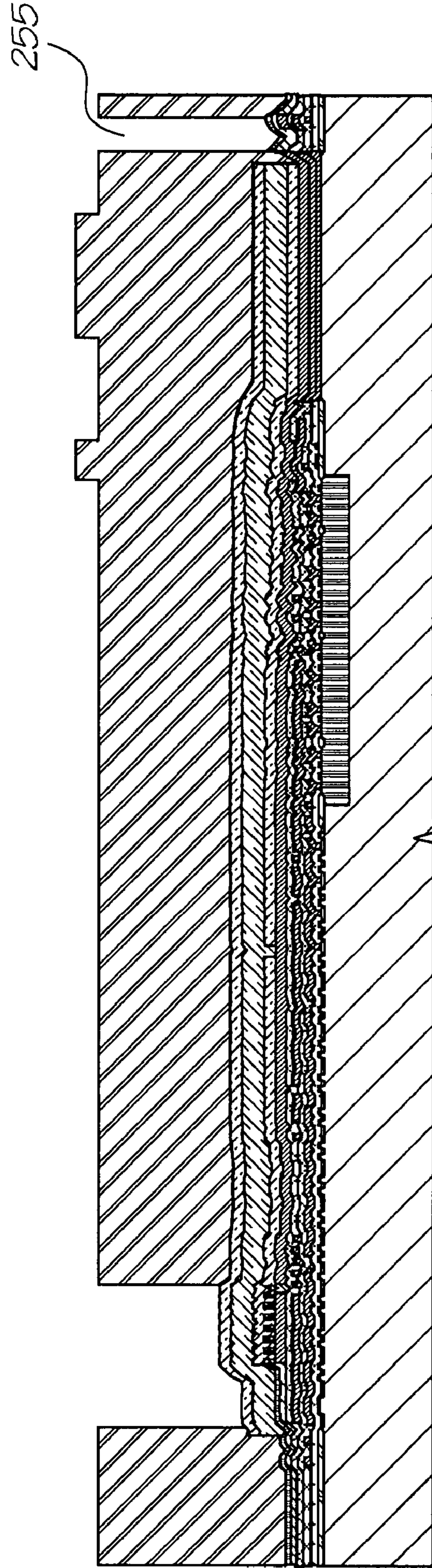
Etch chambers in sacrificial layer
