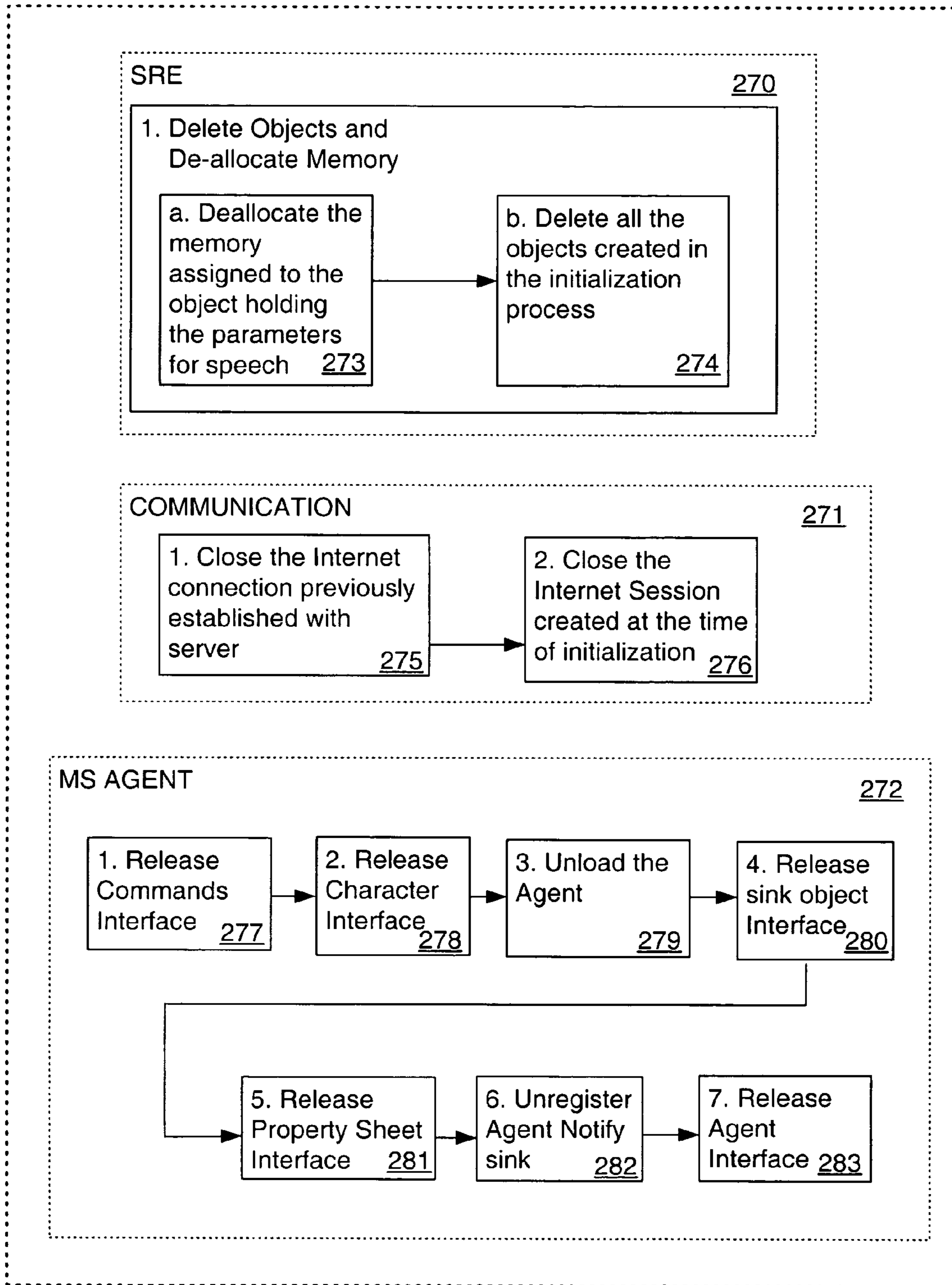
Fig. 4 Client-side Un-Initialization
