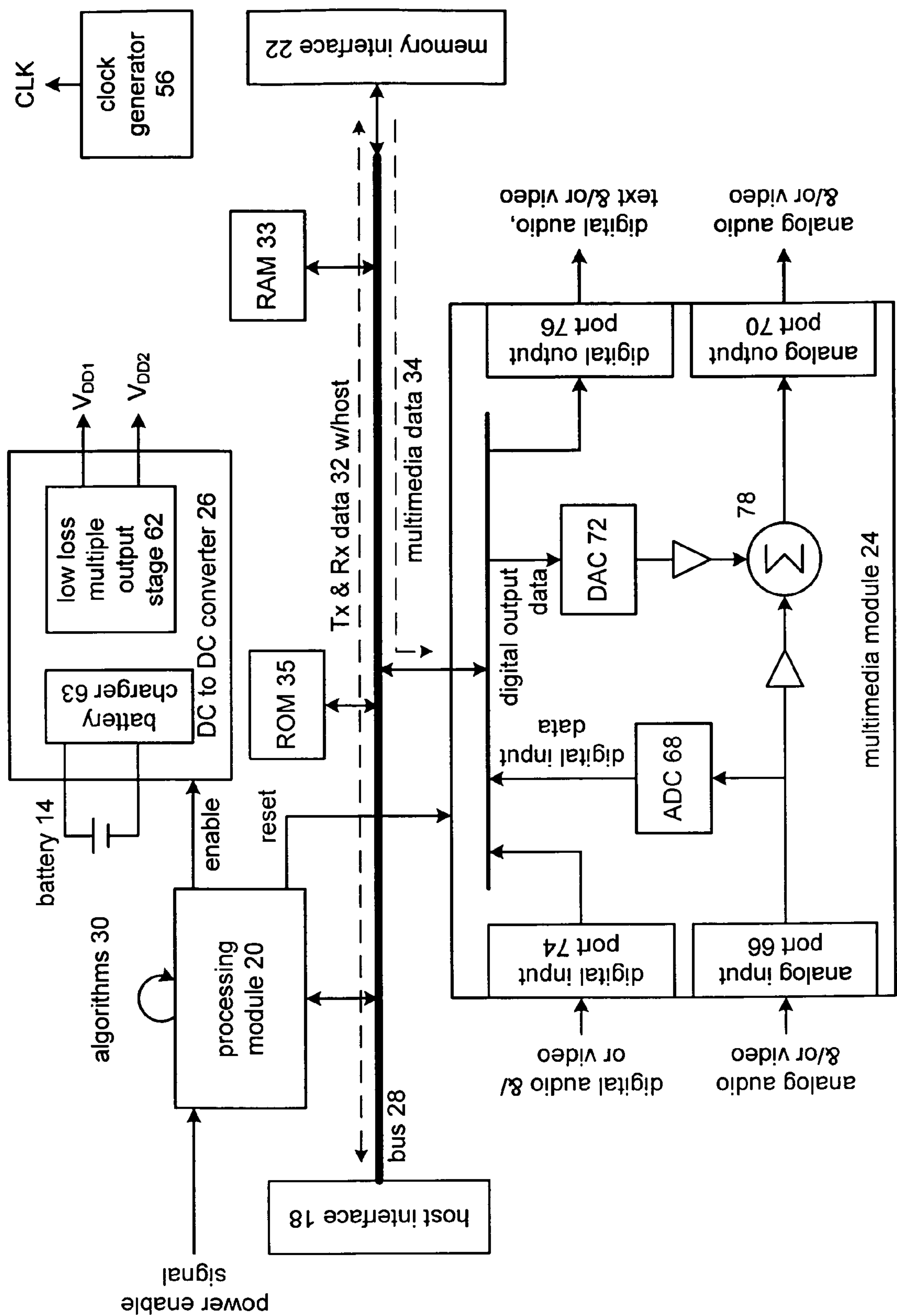
FIG. 3 integrated circuit 12-2
