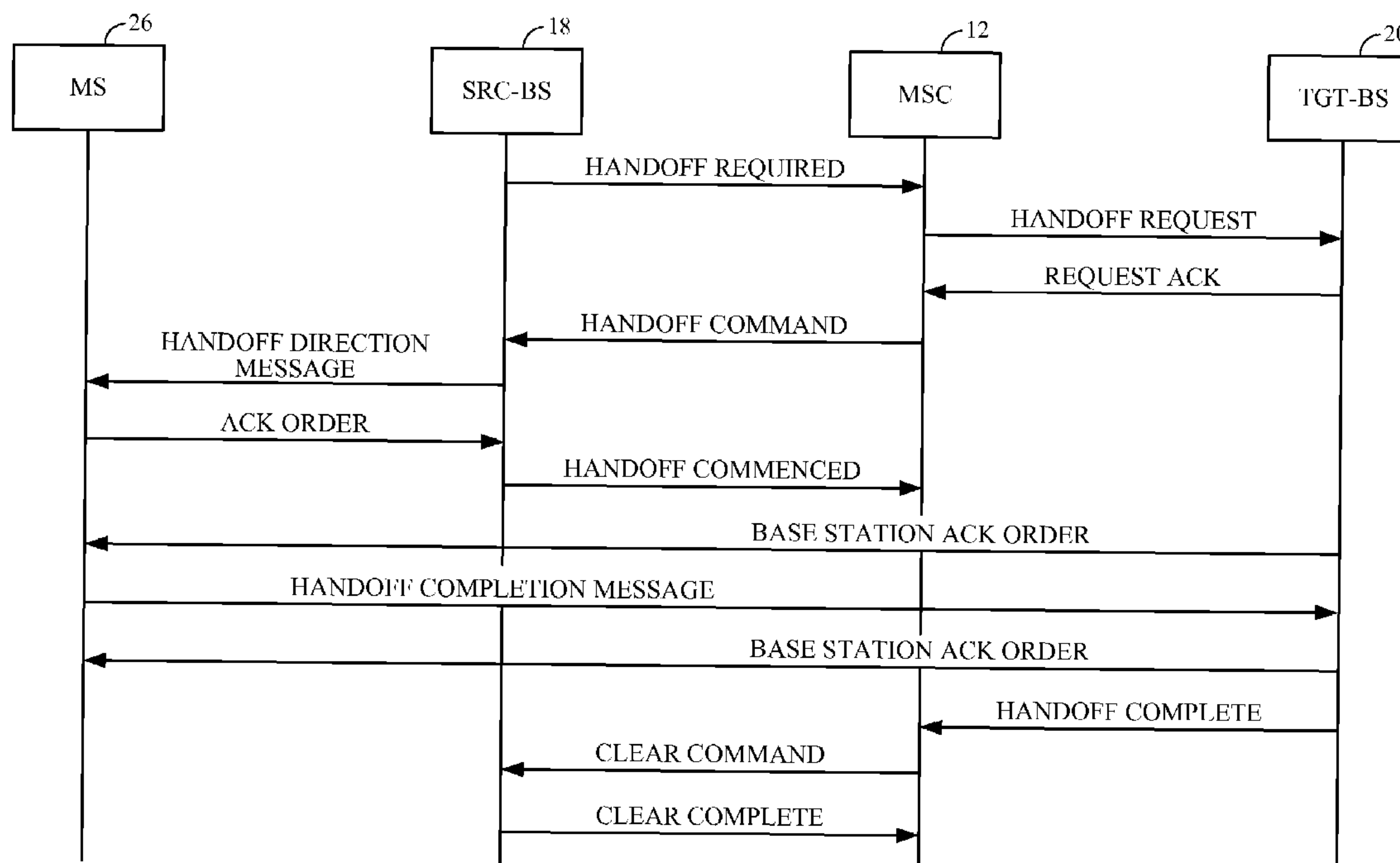
SUCCESSFUL IS-95 TO IS-95 HARD HANDOFF
