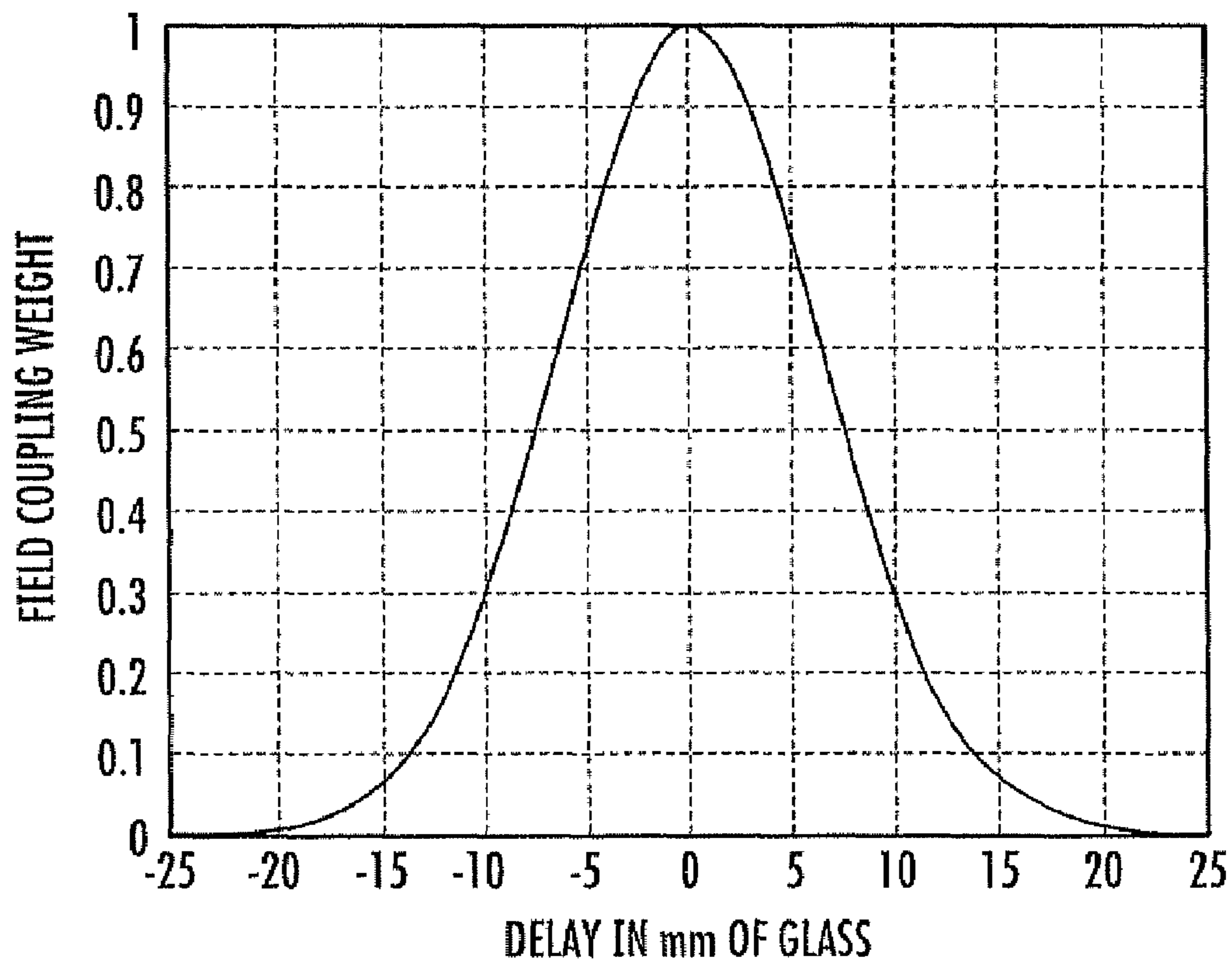
IMPULSE RESPONSE OF 10 GHz BANDPASS GAUSSIAN FILTER
