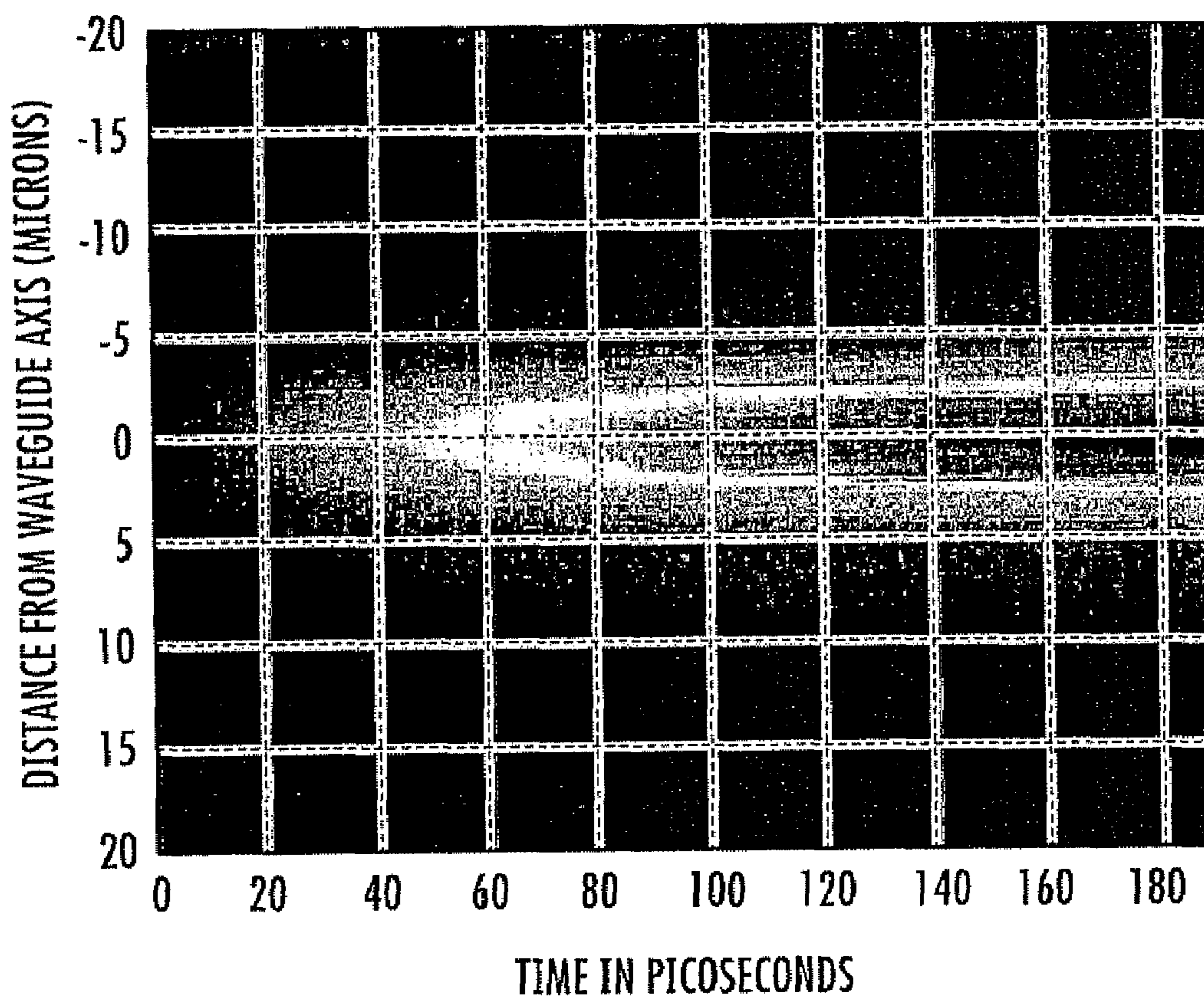
TRANSIENT FIELD PATTERNS IN RESONATOR GUIDE
