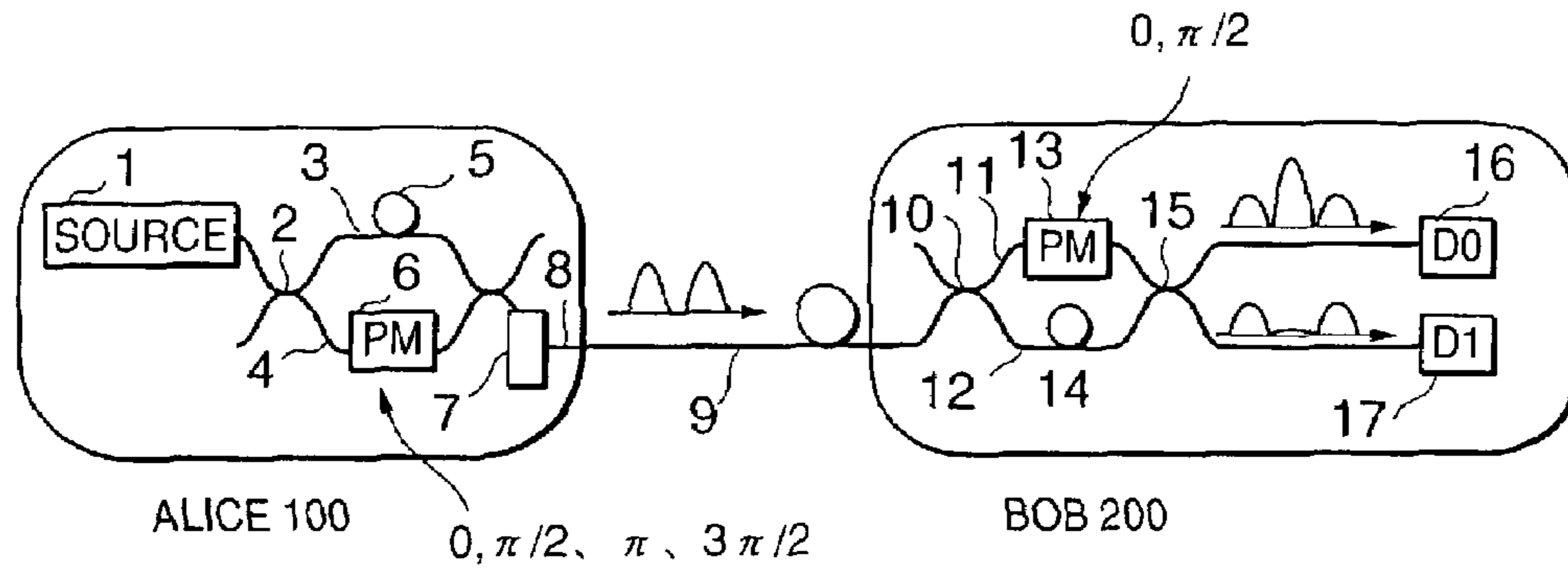
FIG. 1 PRIOR ART
