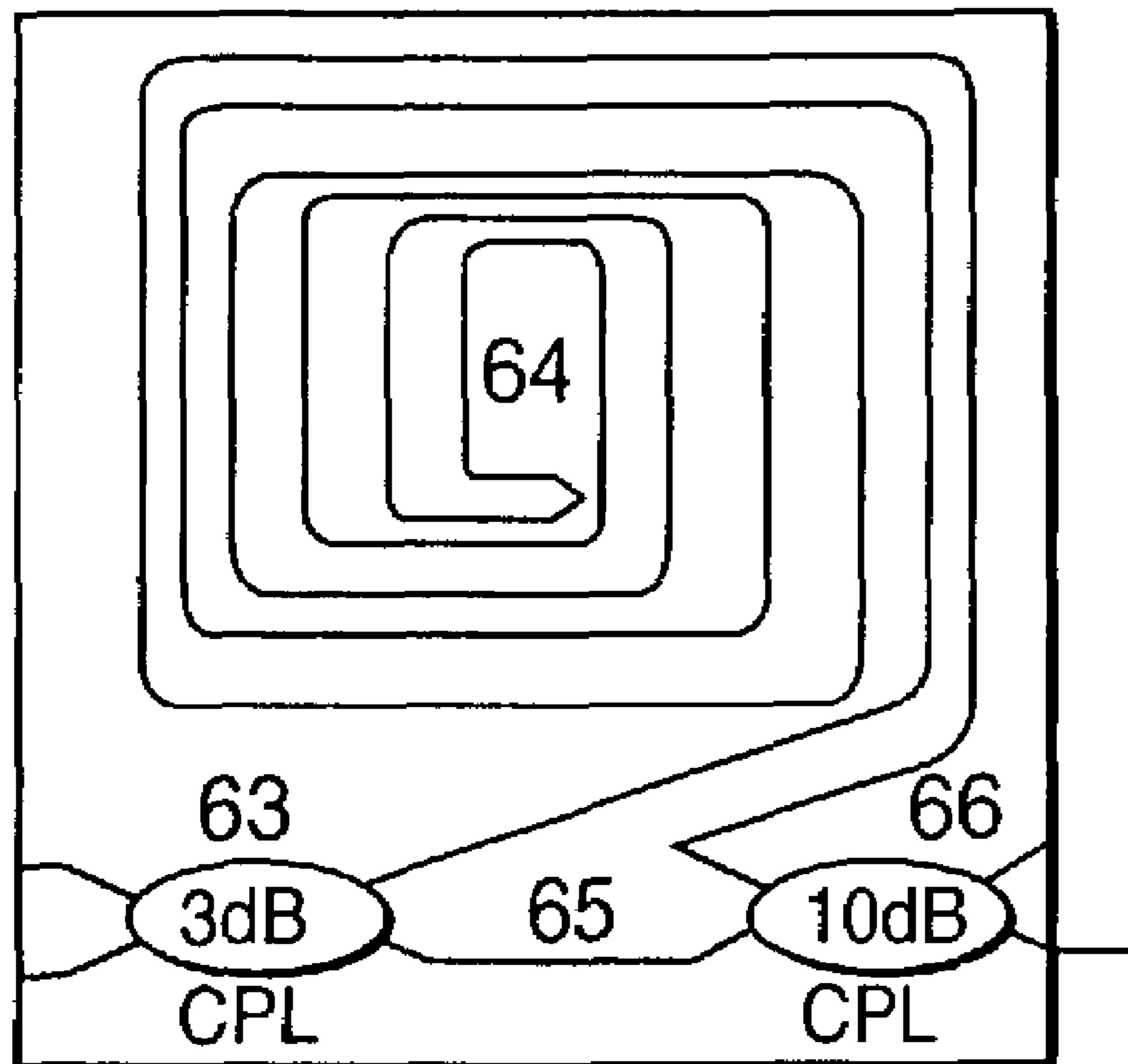
SILICA - BASED UNBALANCED INTERFEROMETER PORTION 80
