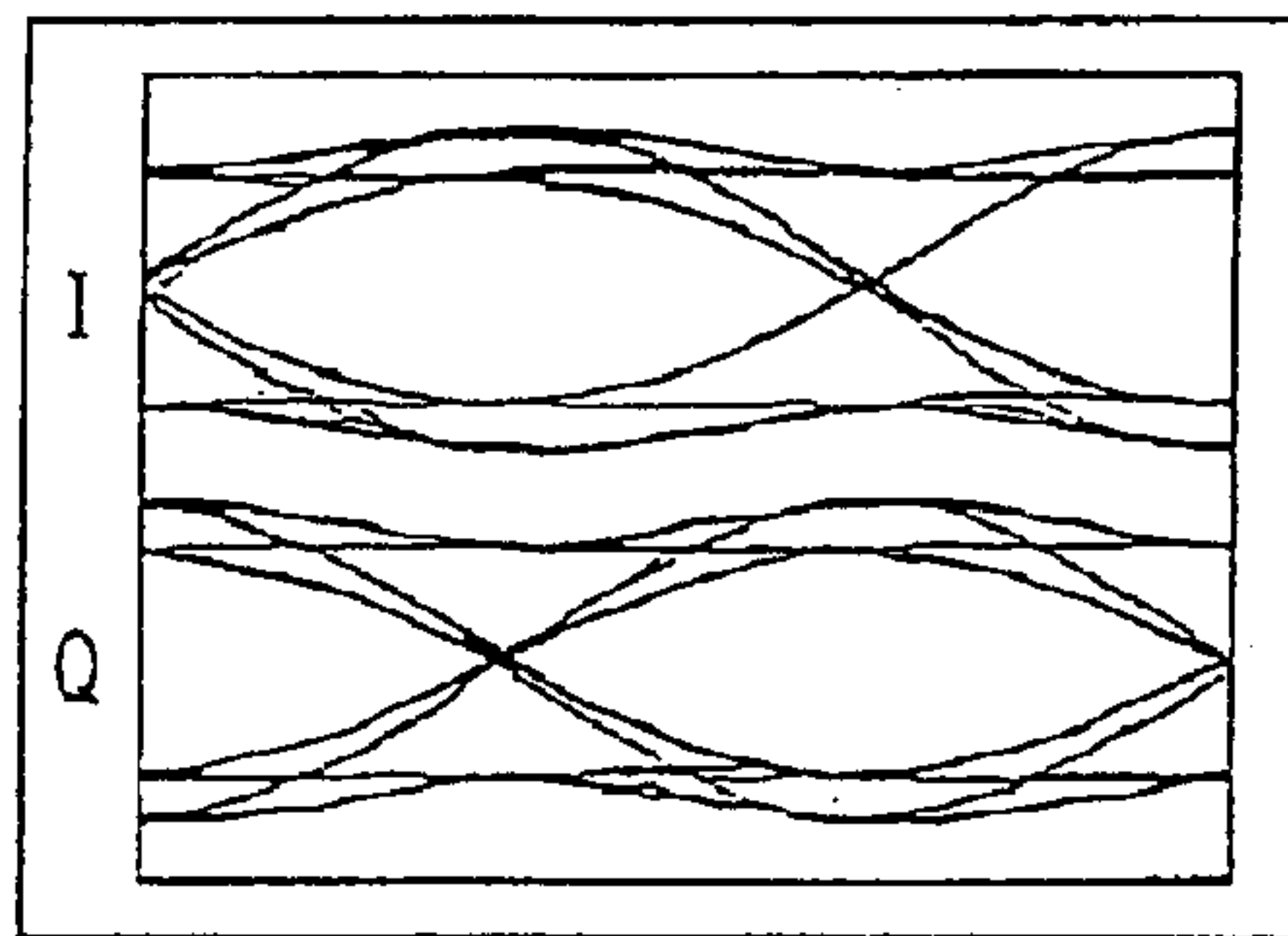
FQPSK-B MEAS. FIG. 19D
