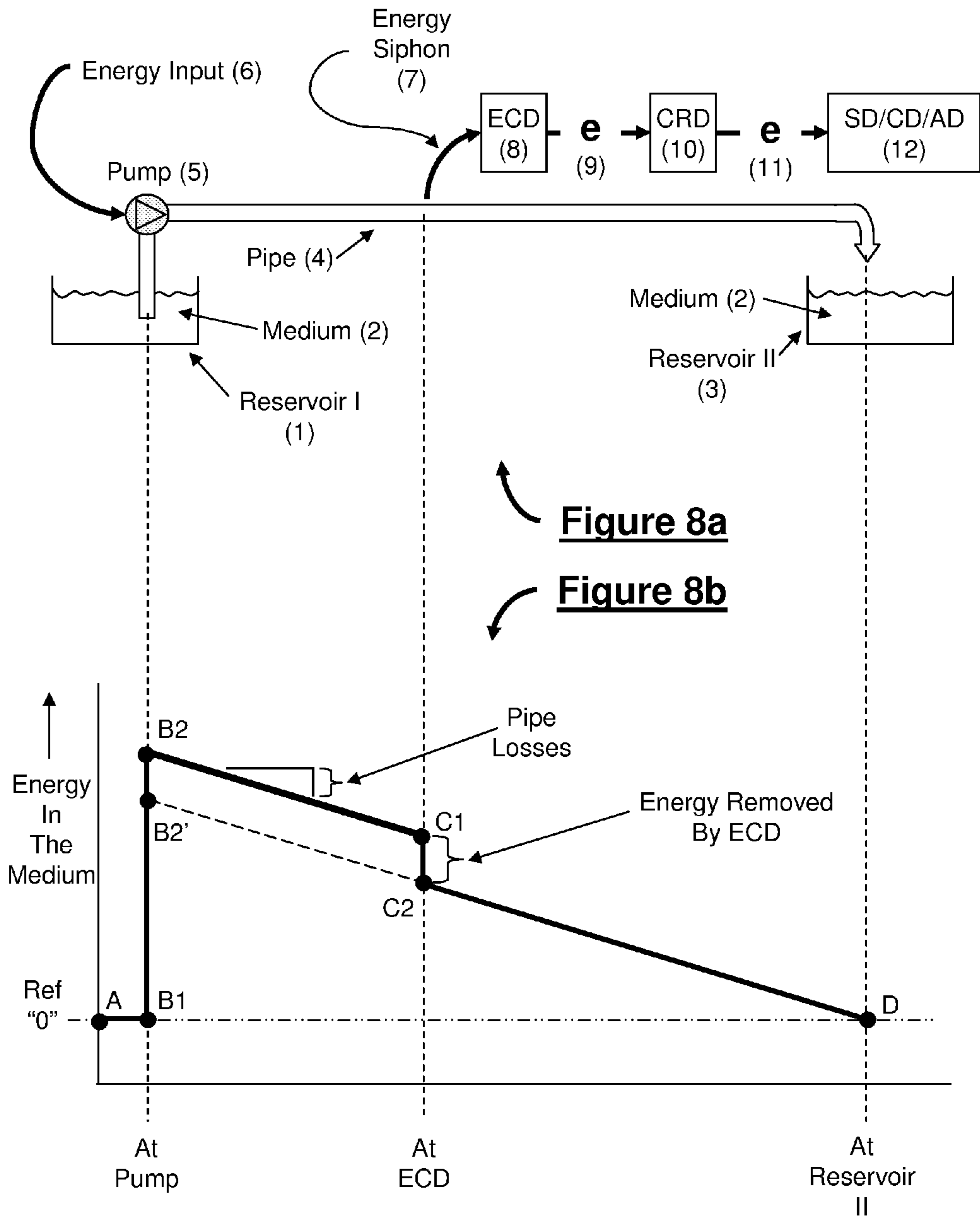
Figure 8-Example of Siphoning Process
