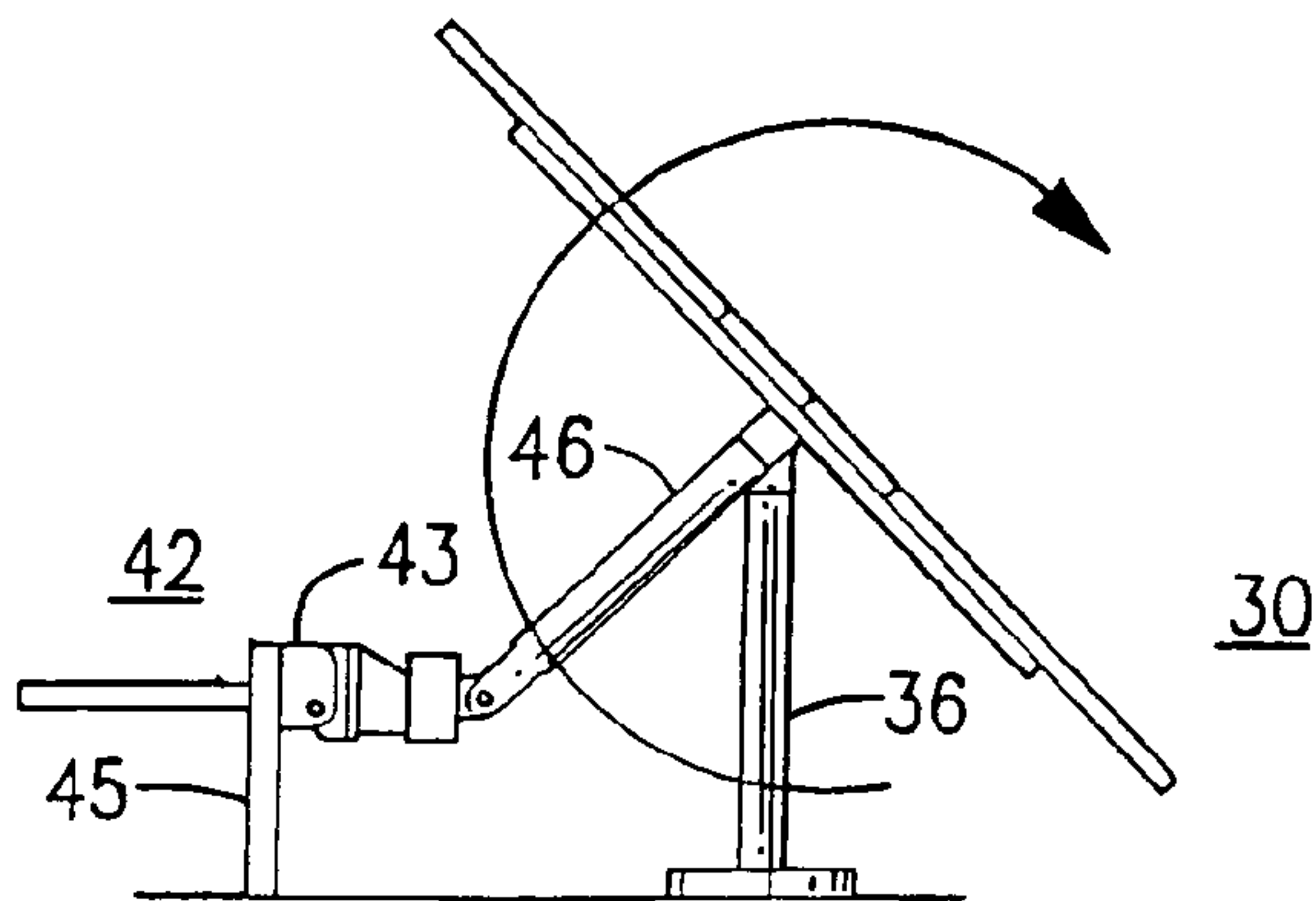
FIG. 2C PRIOR ART
