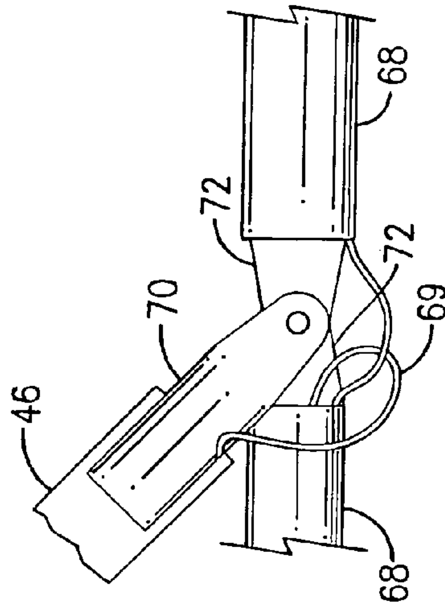
FIG. 5 PRIOR ART
