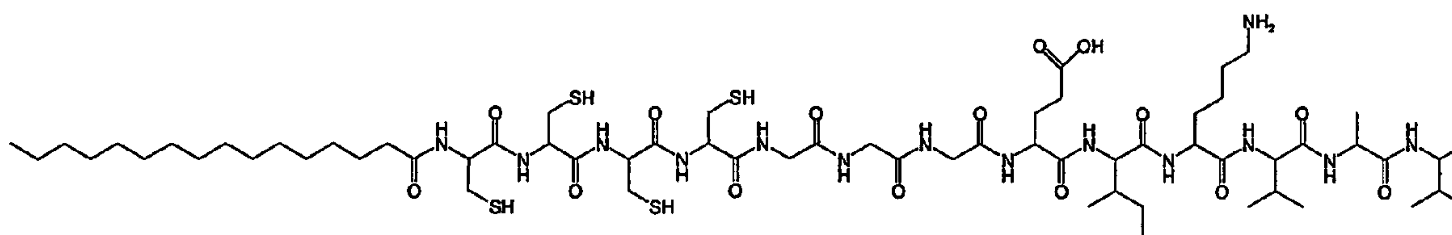
Molecule 1
